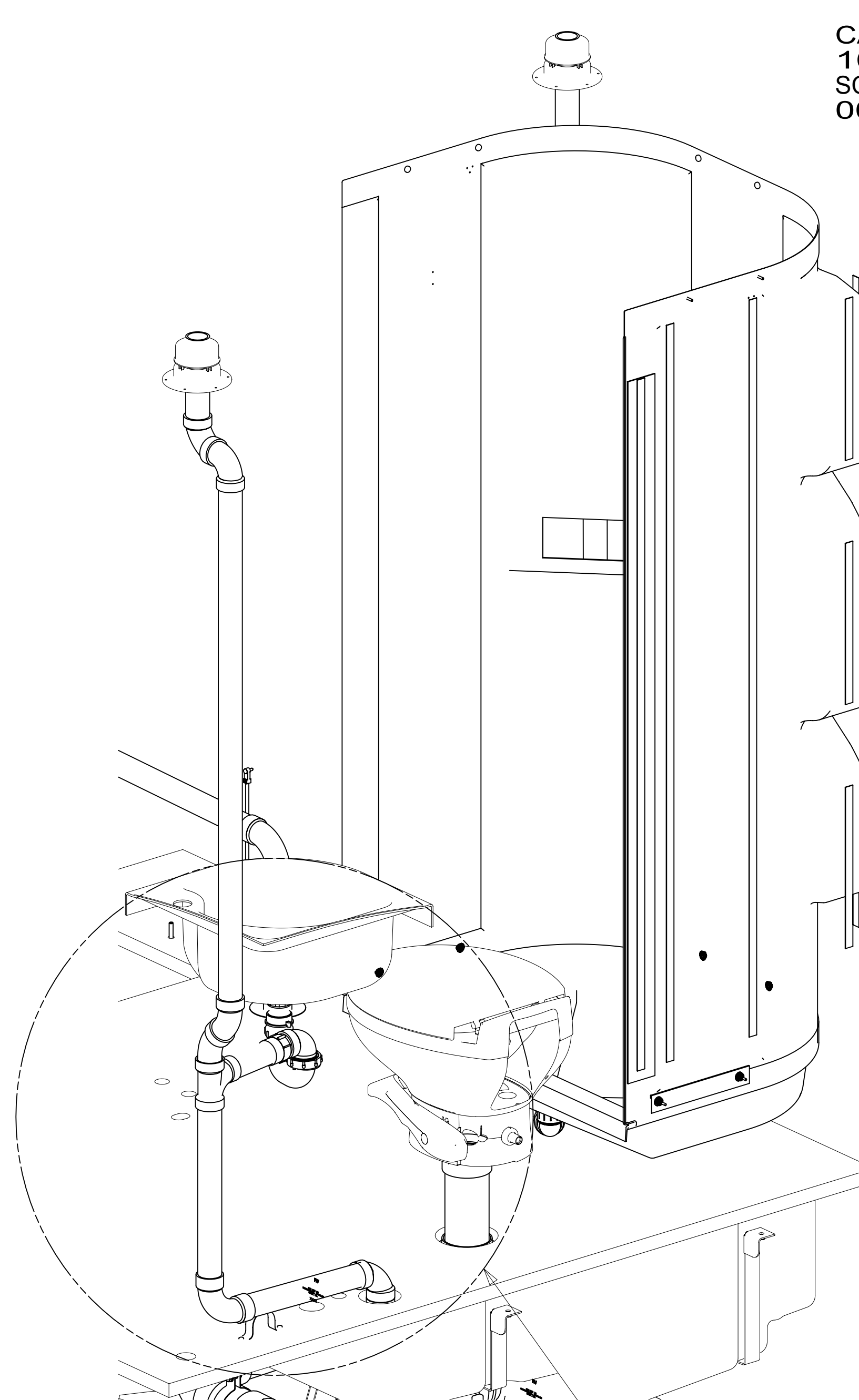
DETAIL BC
