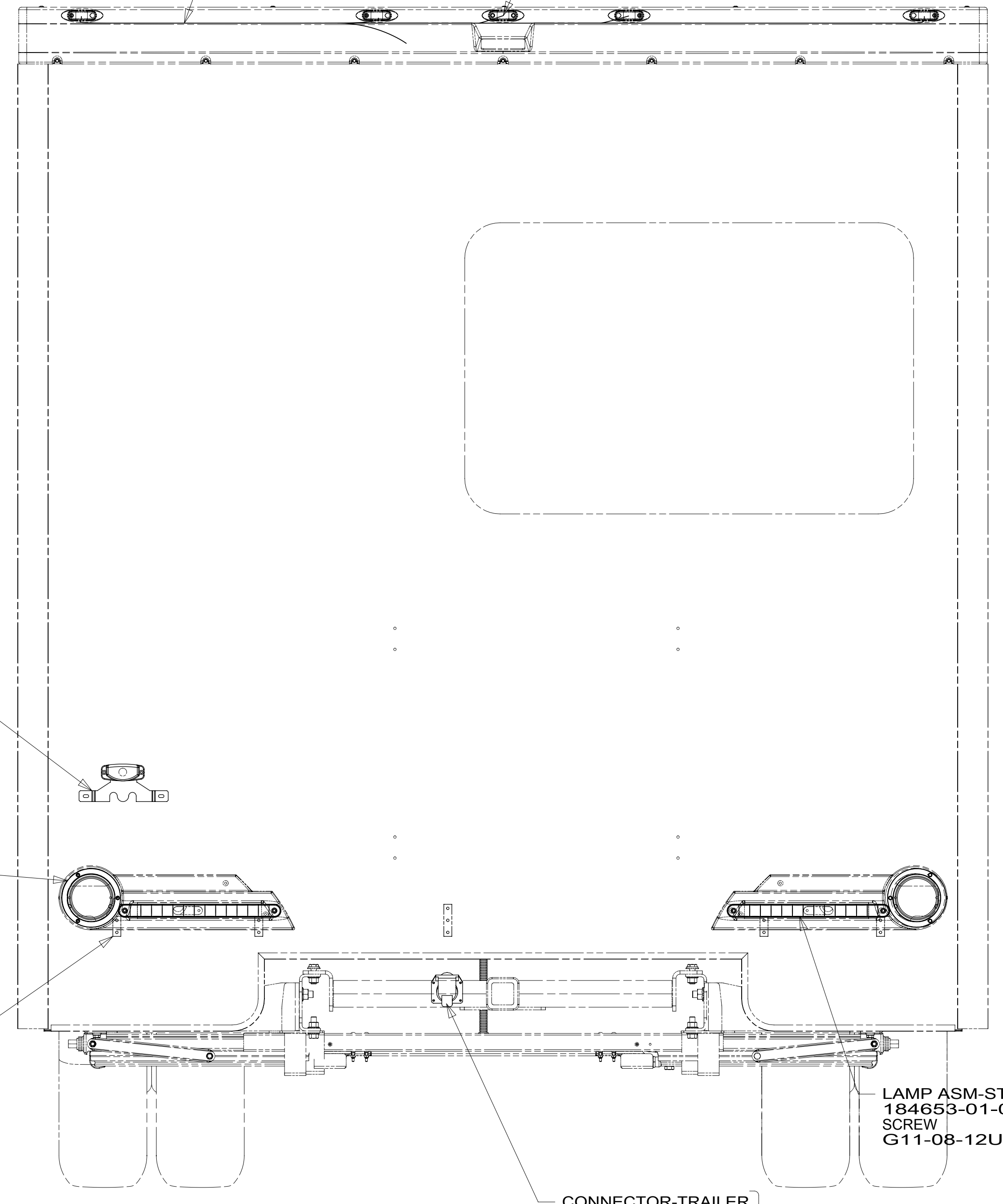
VIEW BB
