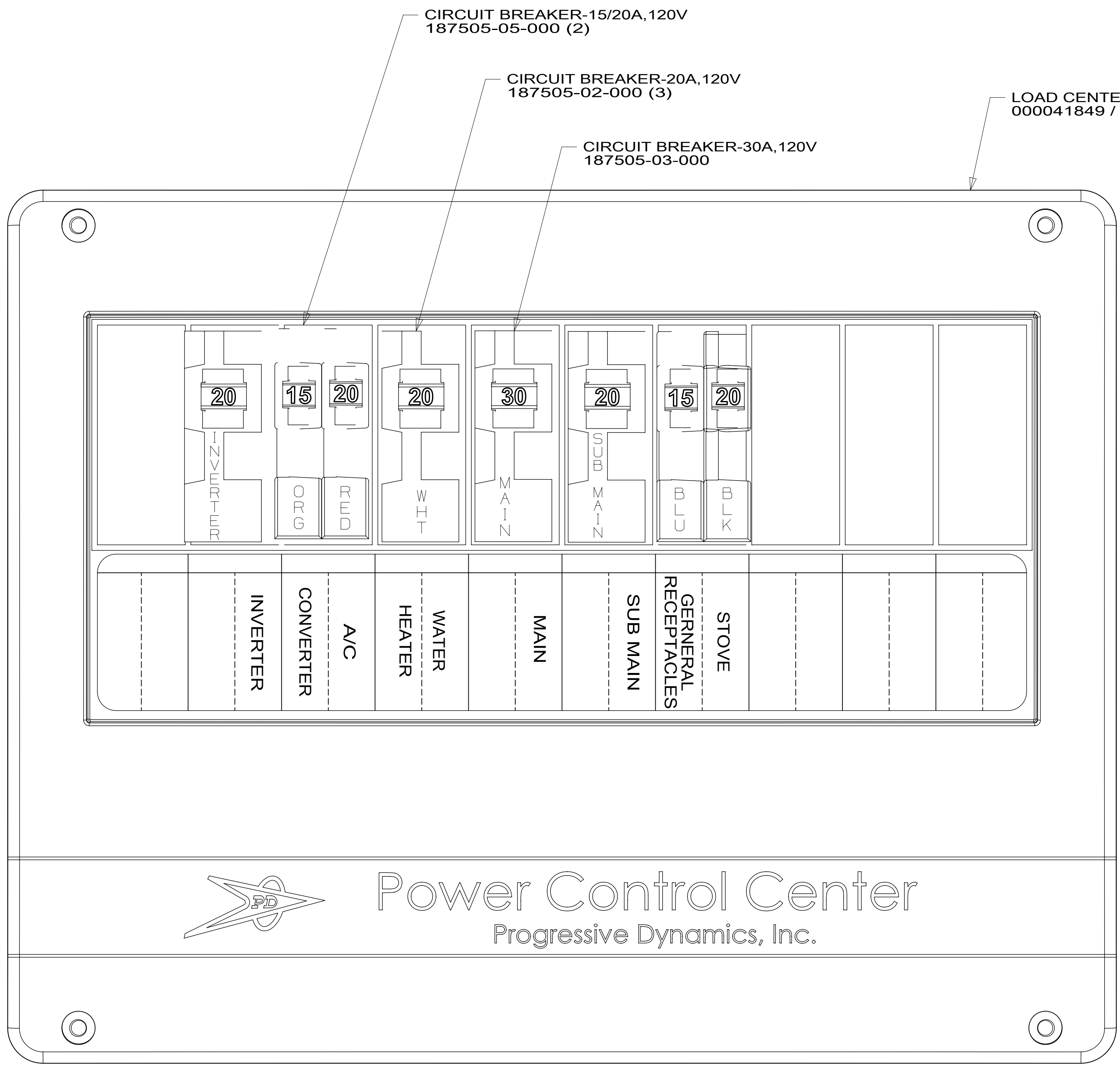
FRONT VIEW
