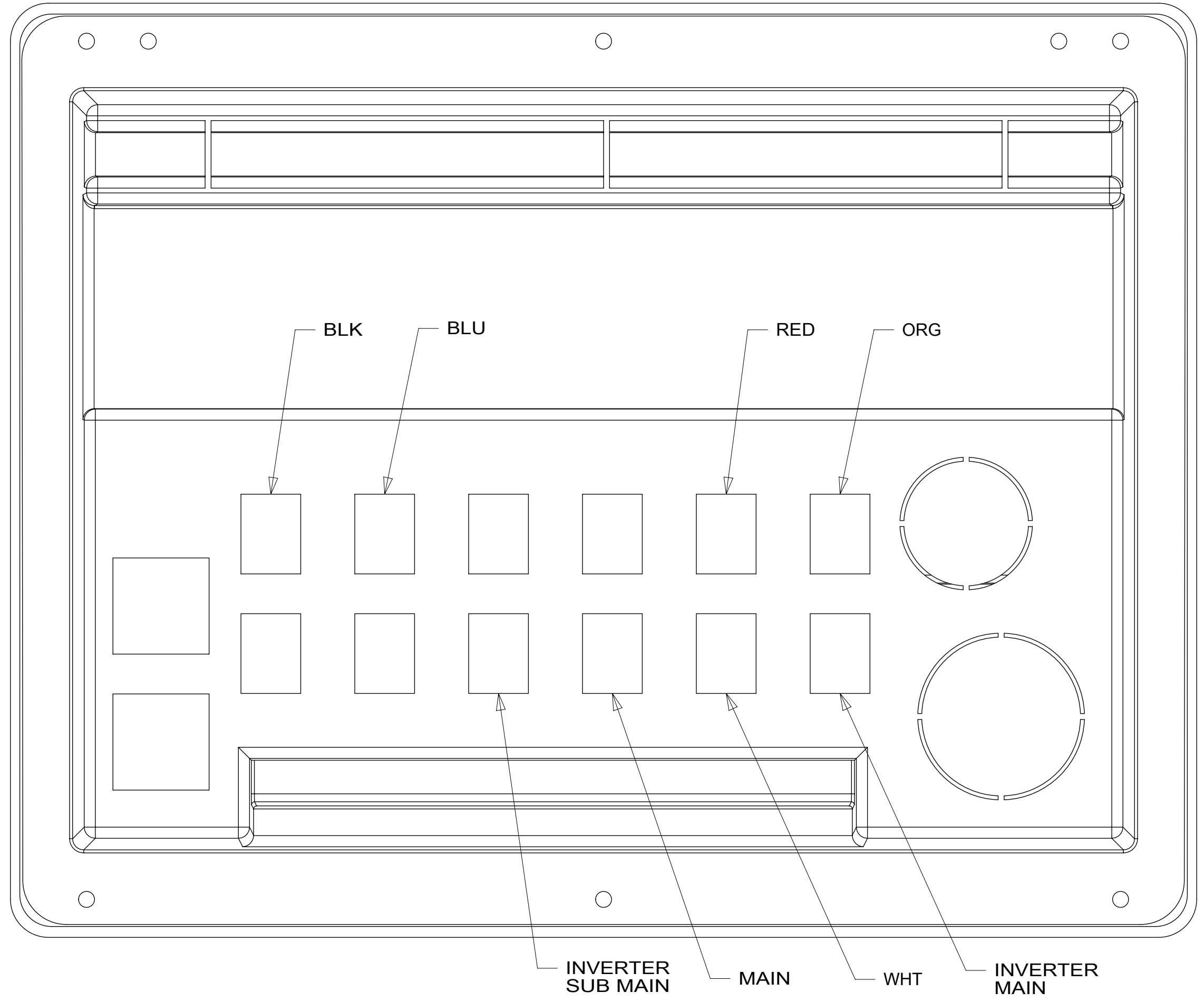
BACK VIEW
