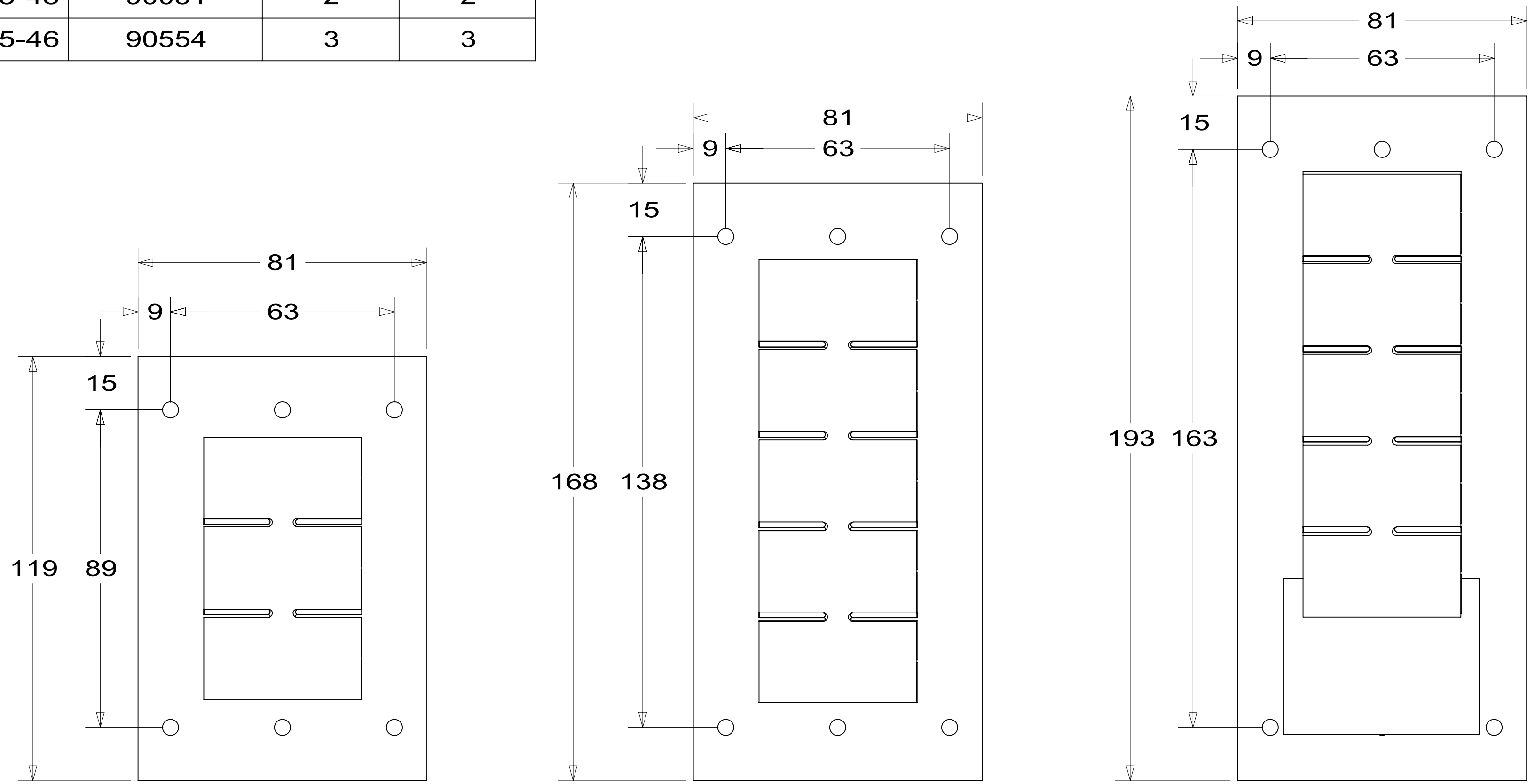
FIGURE 1 (6 POSITION SWITCH PANEL) FIGURE 2 (10 POSITION SWITCH PANEL) FIGURE 3 (10 POSITION SWITCH/LCD PANEL)
