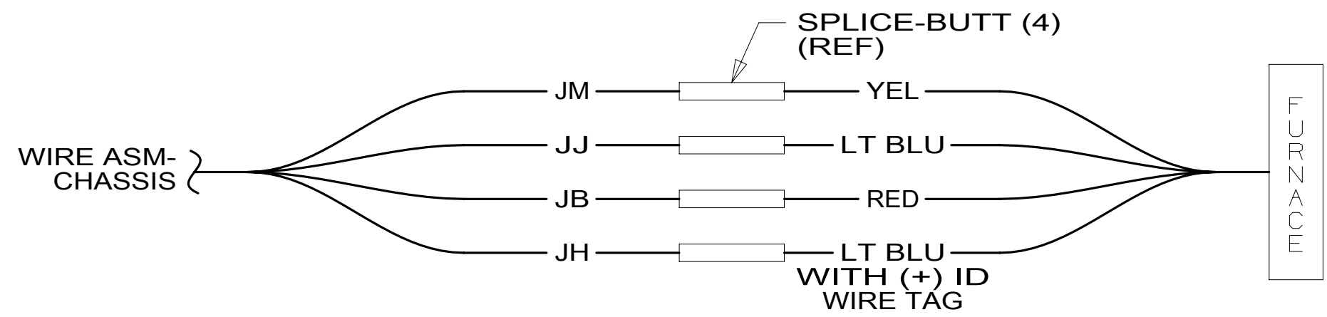
DETAIL AC
