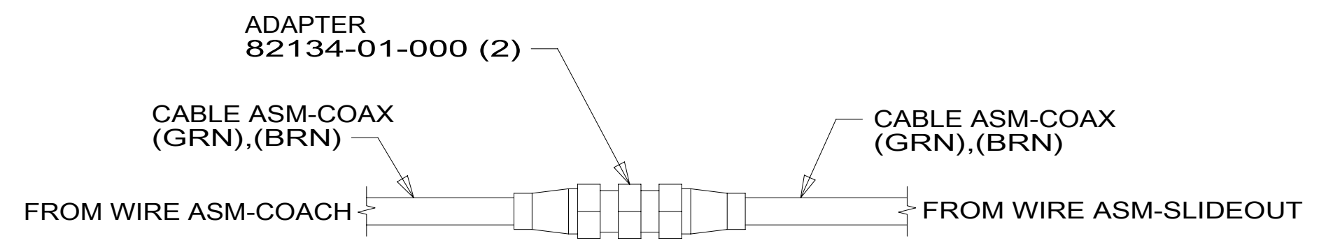
DETAIL DR
