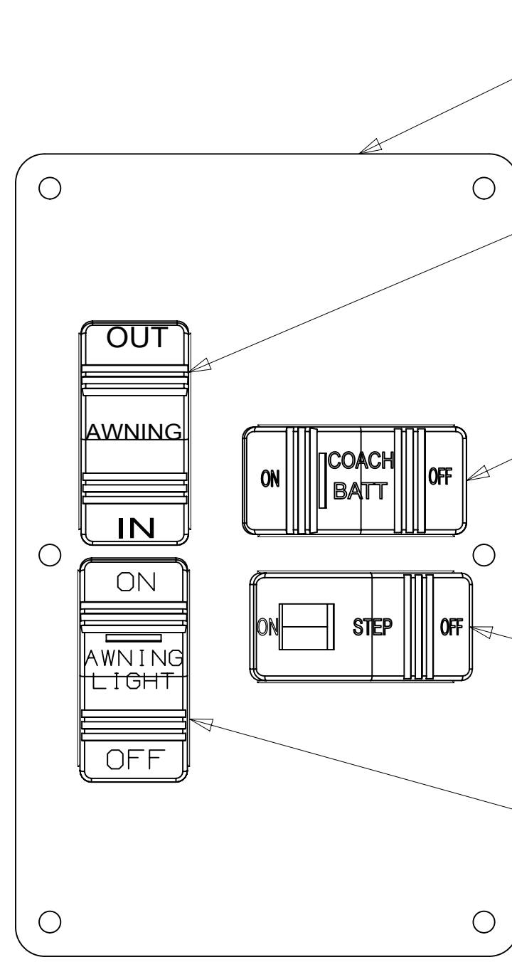
DETAIL DB 1
