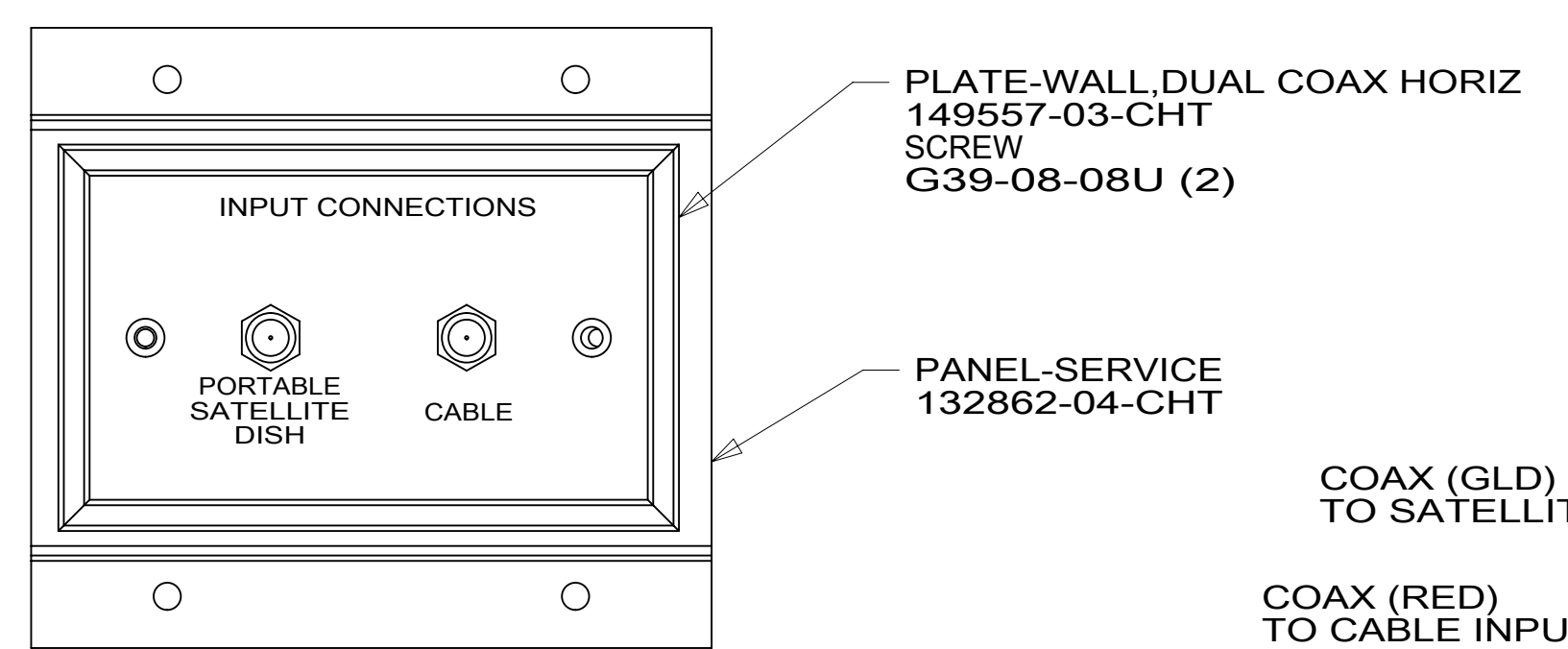
VIEW AA
