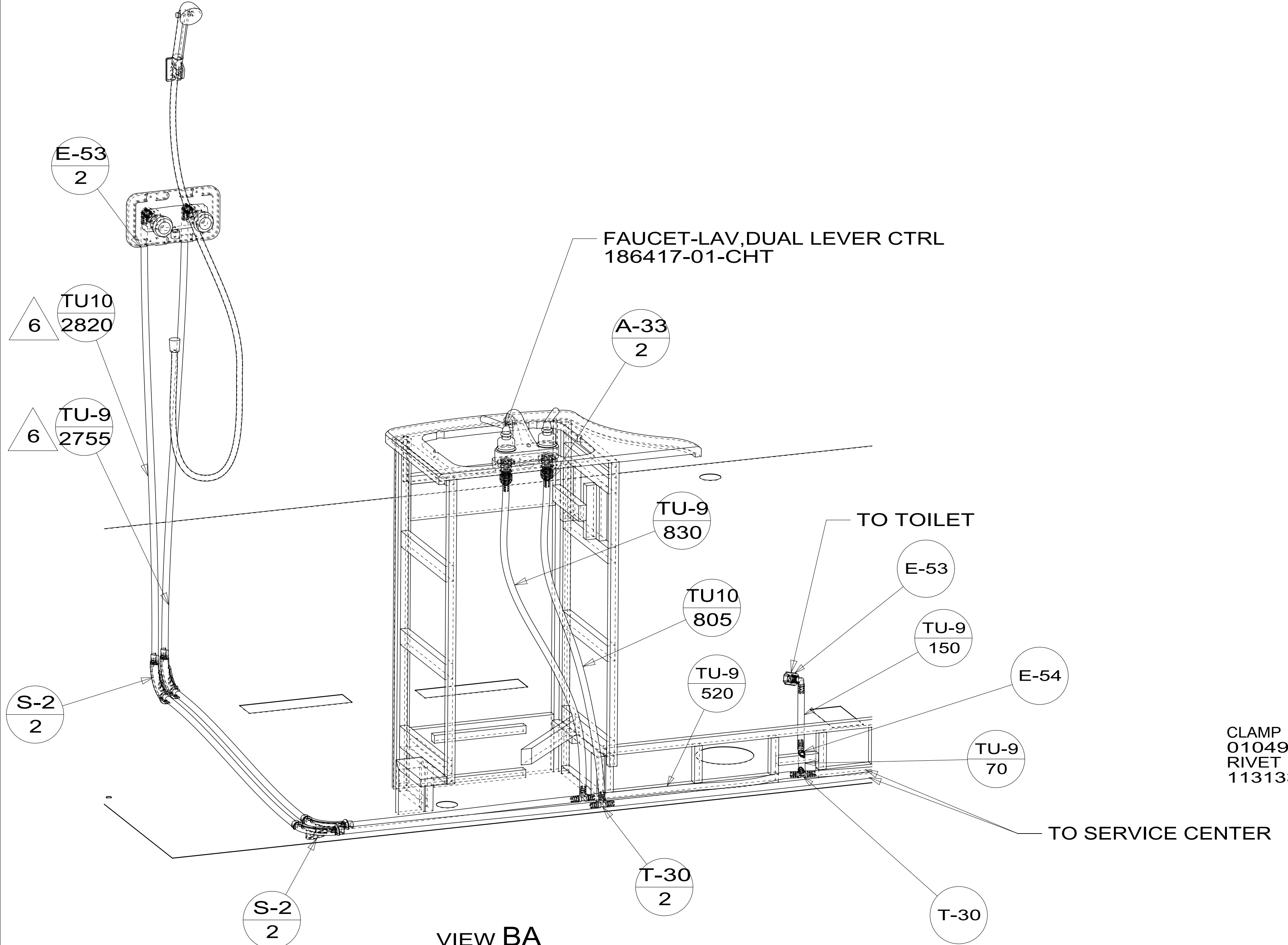
VIEW BA
