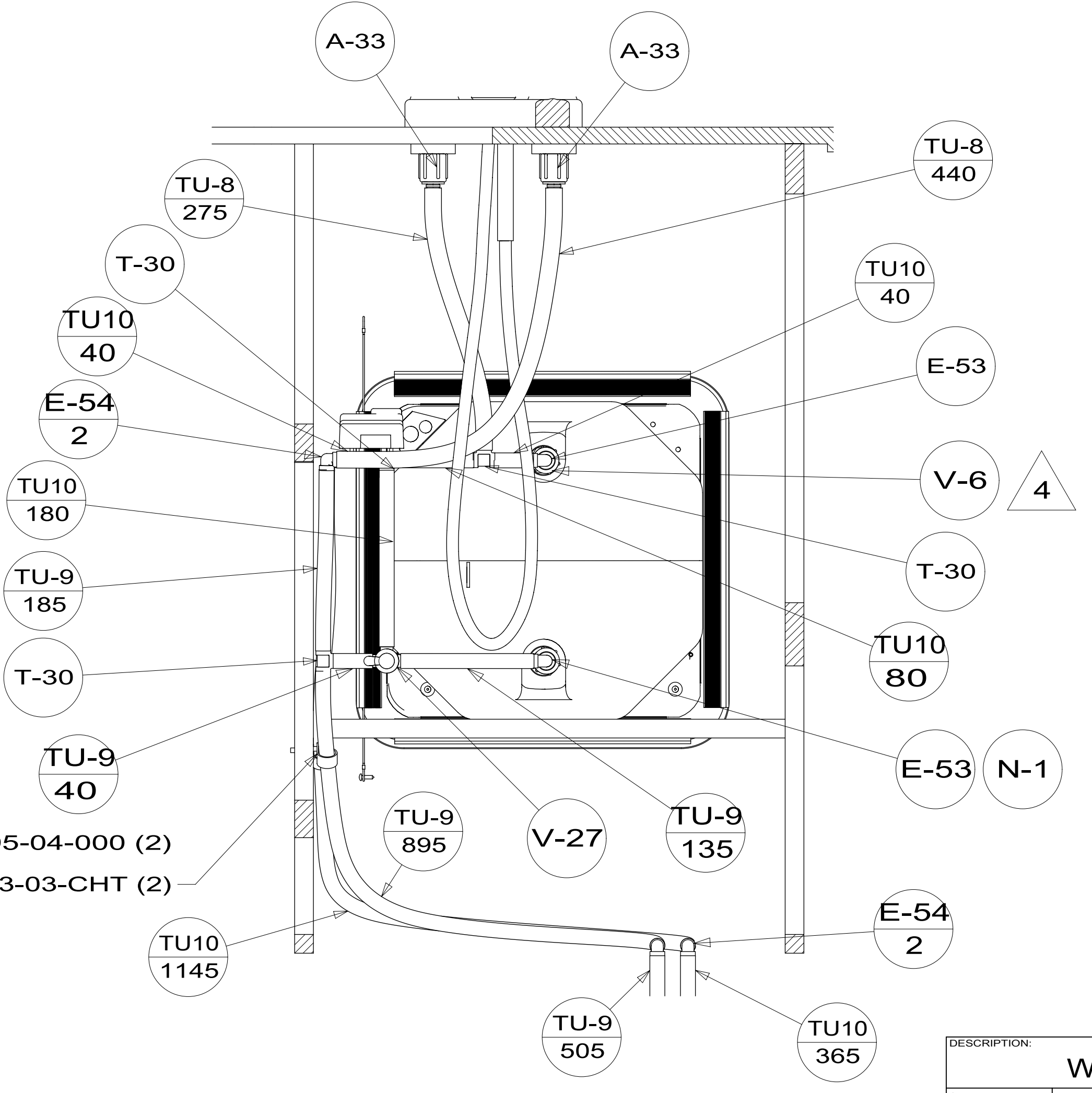
SECTION BD-BD
