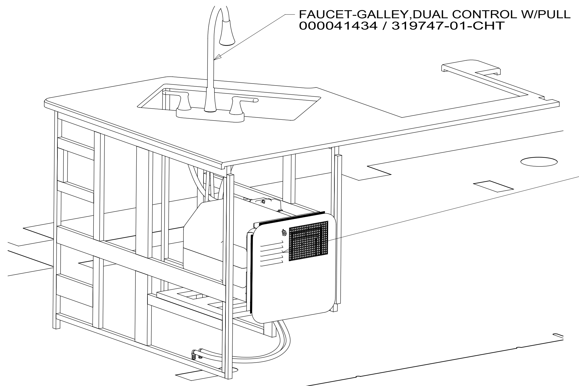
VIEW BB
