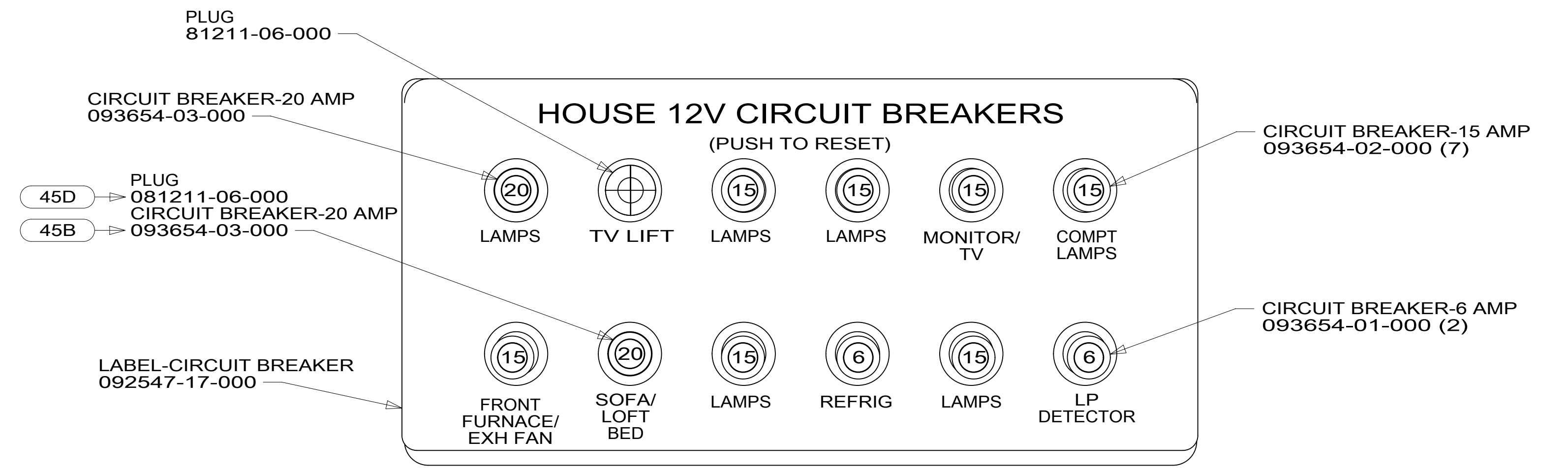
DETAIL EB (BACK VIEW)
