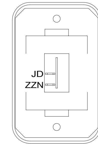
DETAIL DN 9PC
