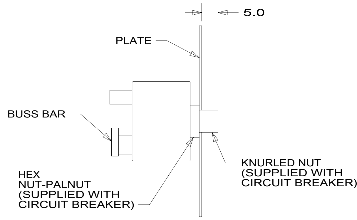
VIEW EC-EC
