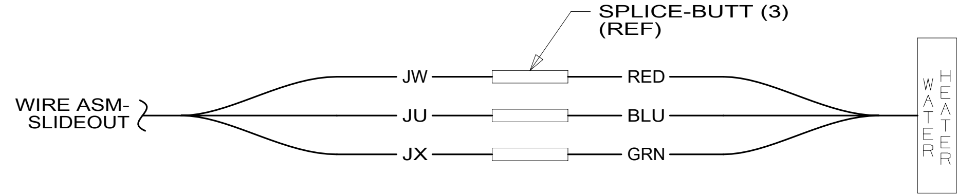
DETAIL BA
