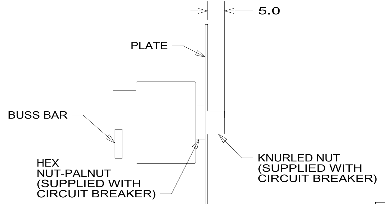
VIEW DB-DB
