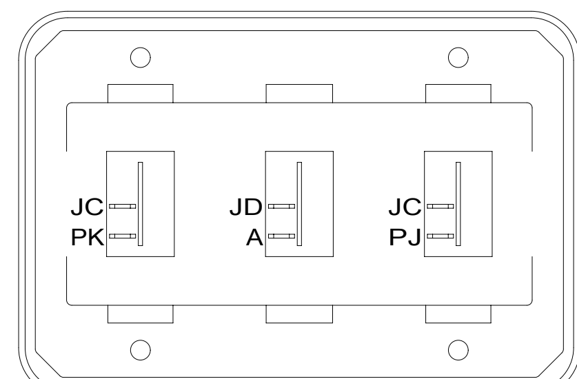
DETAIL DG
