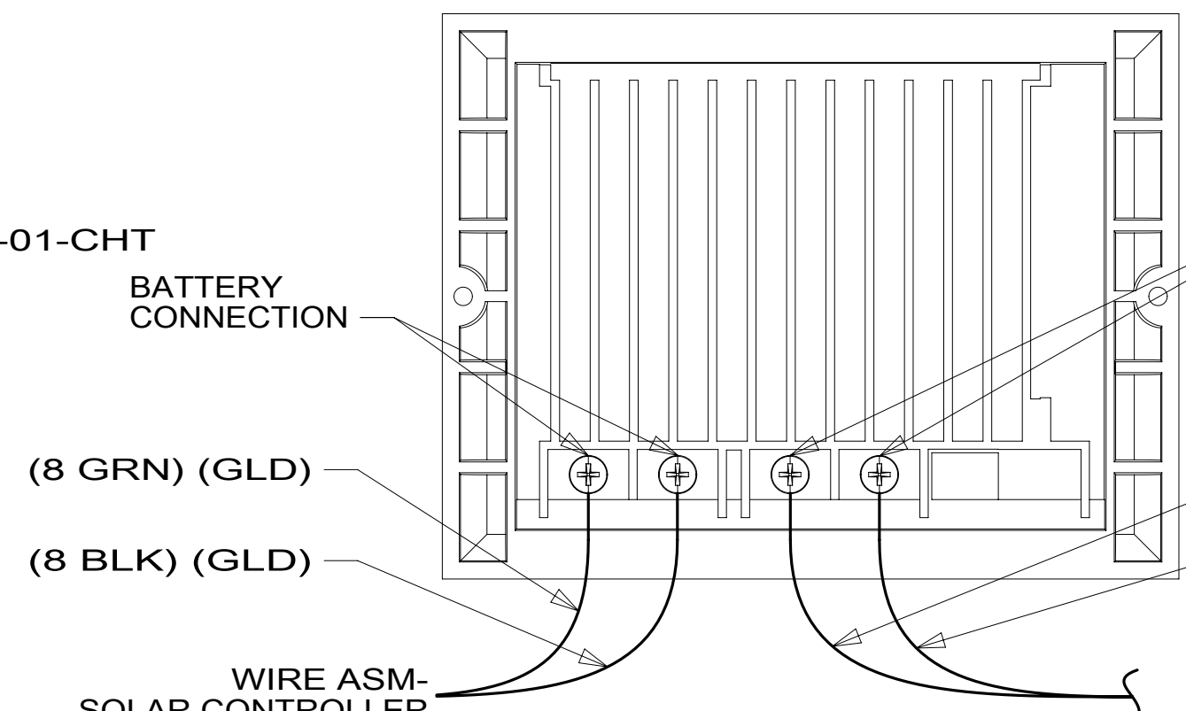
DETAIL DK
