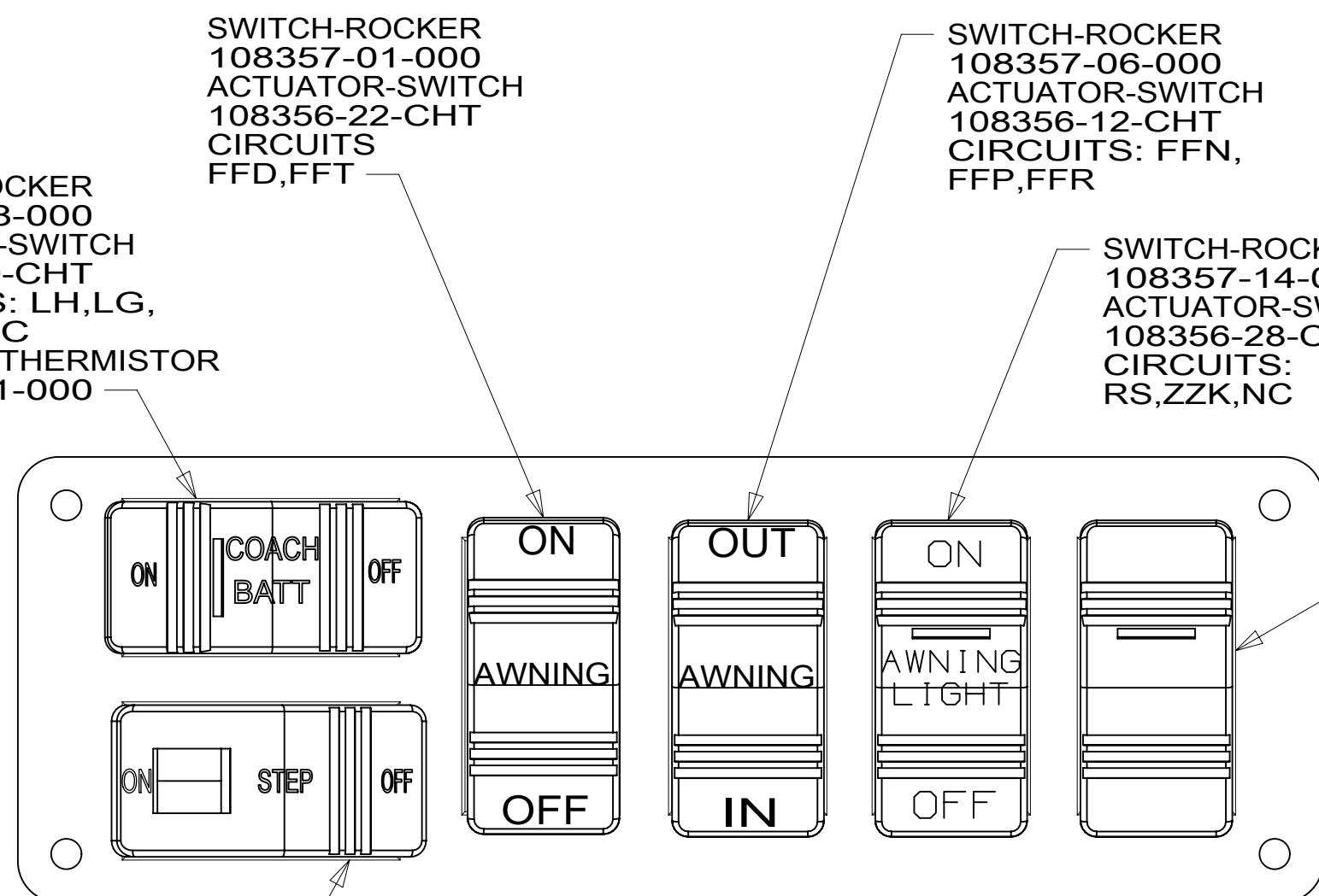
DETAIL DF
