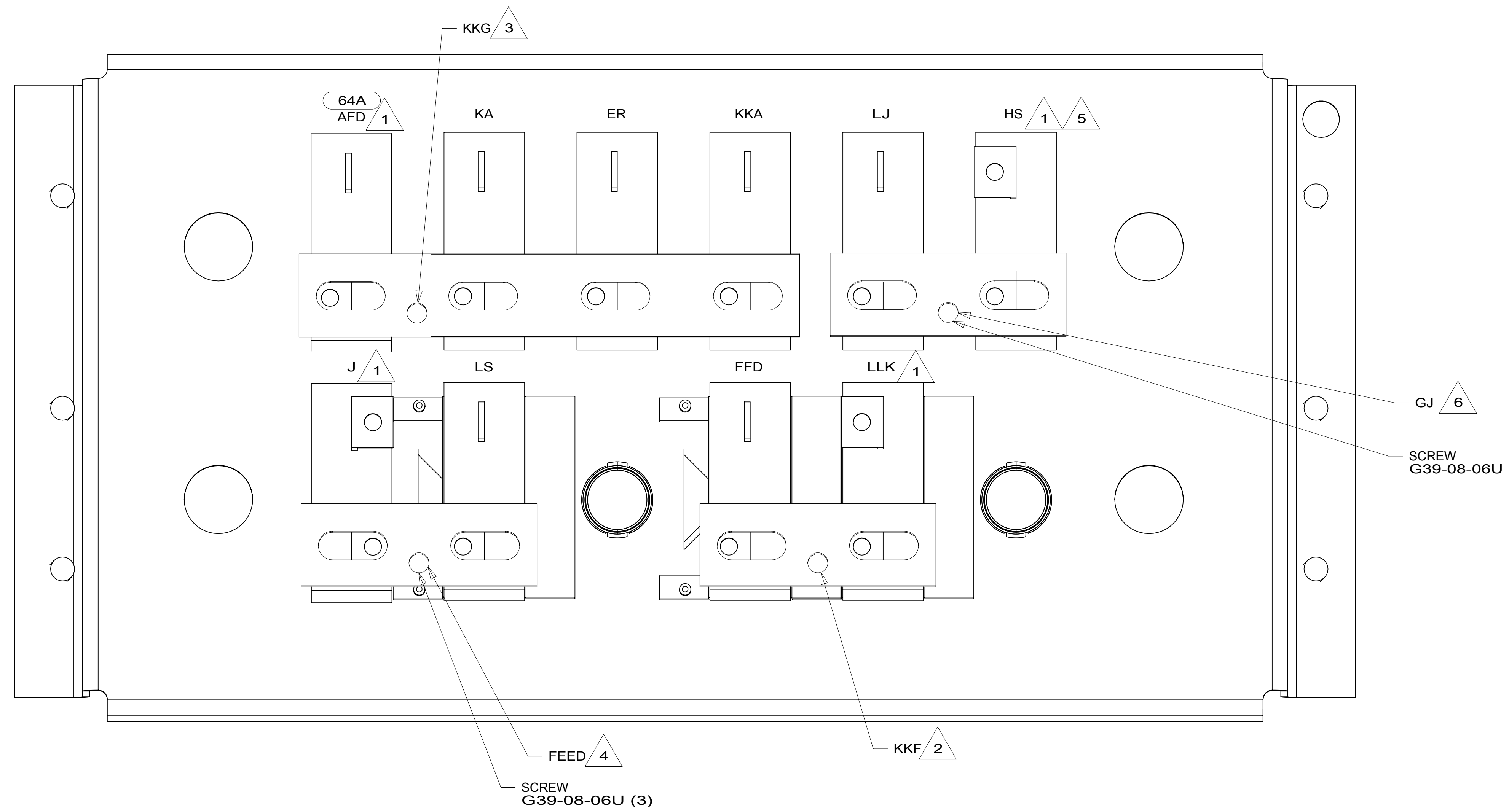
VIEW EA
