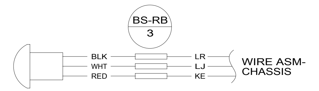
DETAIL GF
