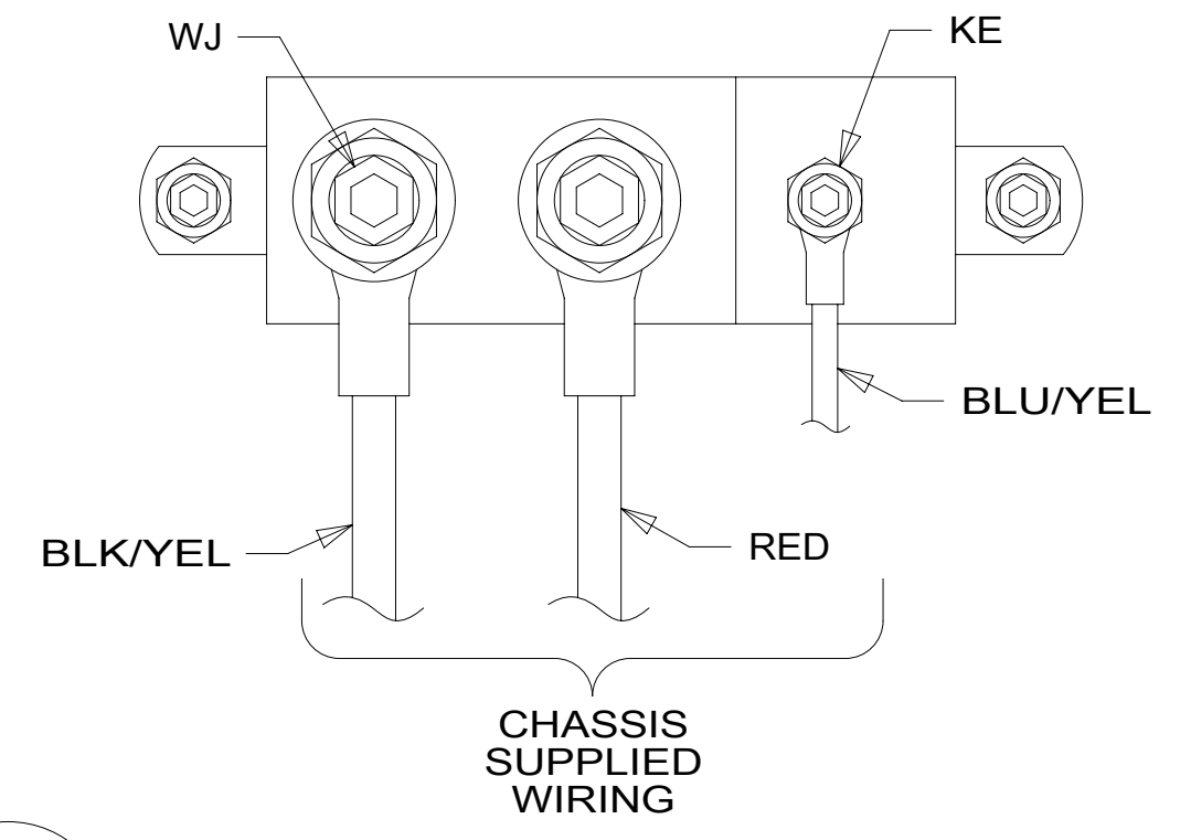
DETAIL GD 3
