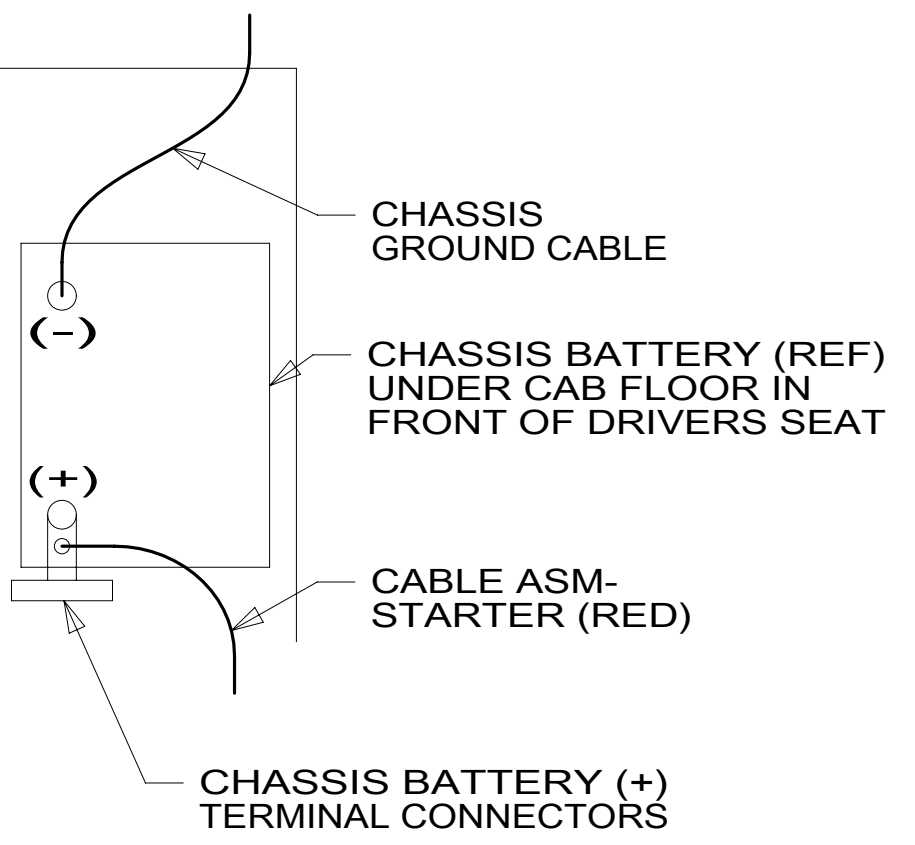
DETAIL AA
