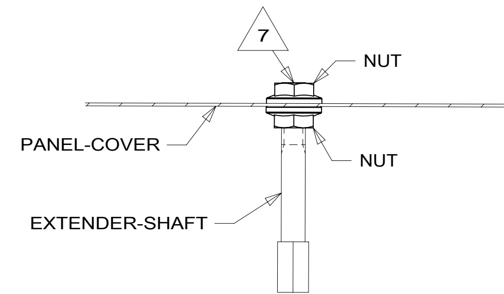
SECTION AC-AC
