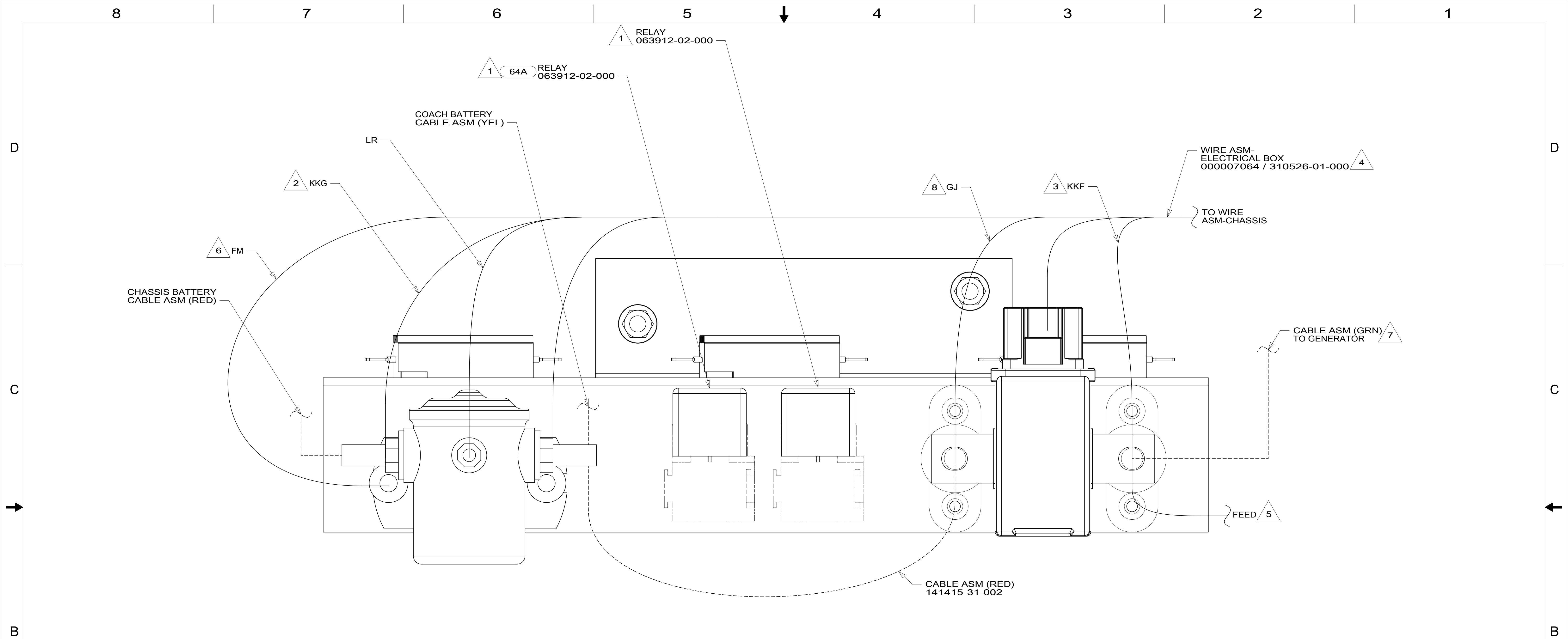
VIEW FA
