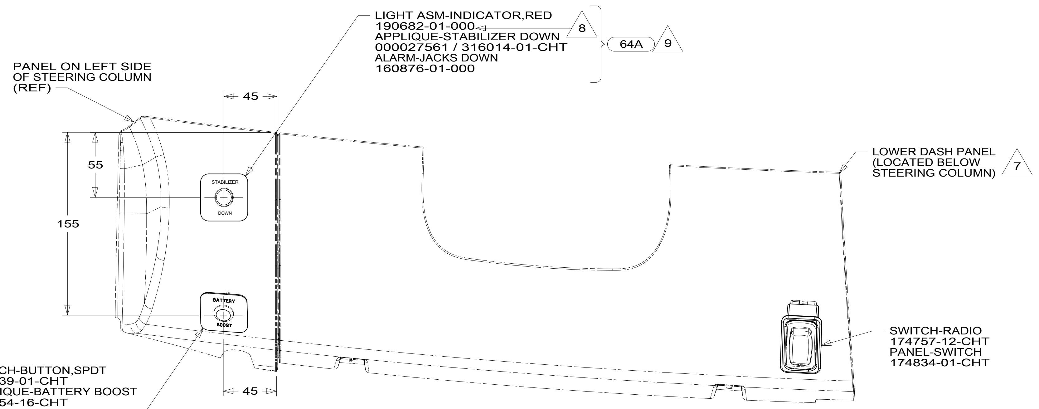
VIEW GA
