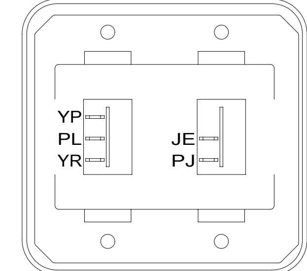
DETAIL CB
