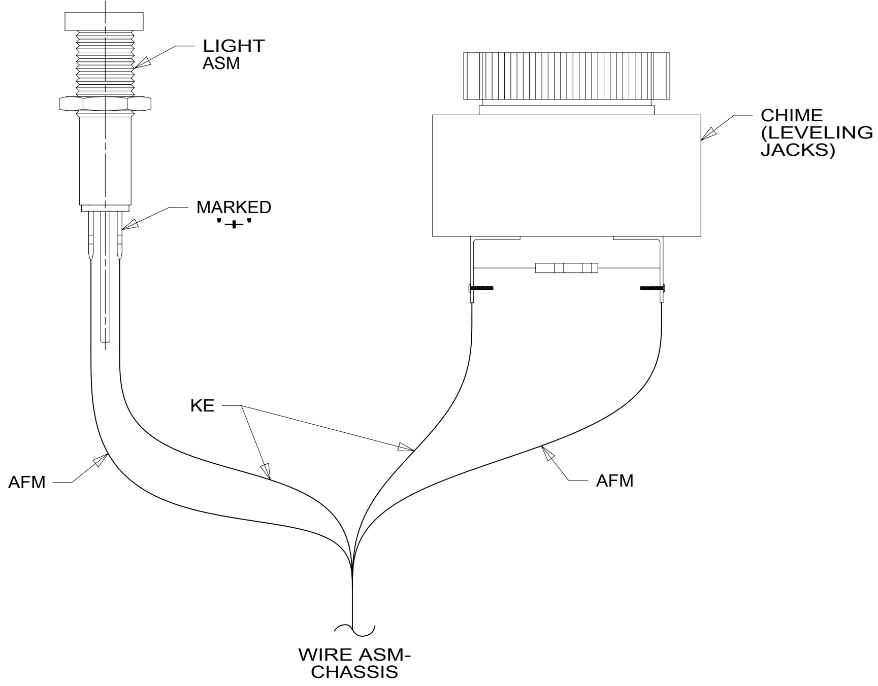
DETAIL CC 64A
