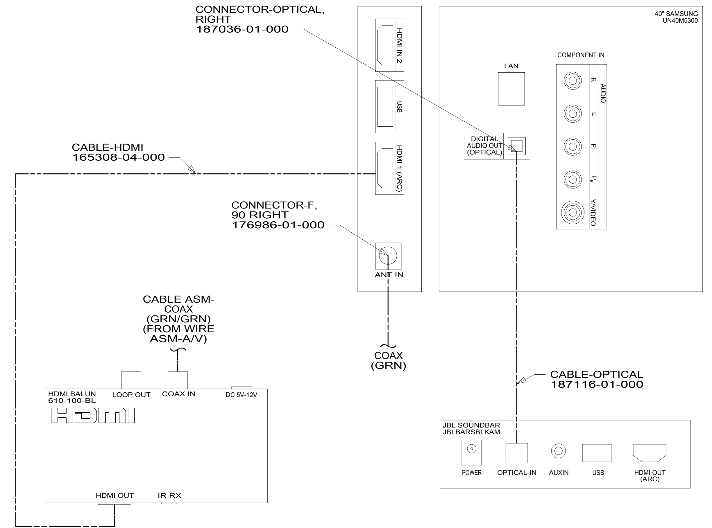
VIEW DB
