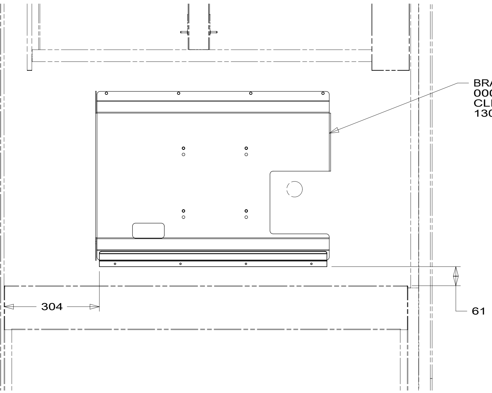
VIEW CC
