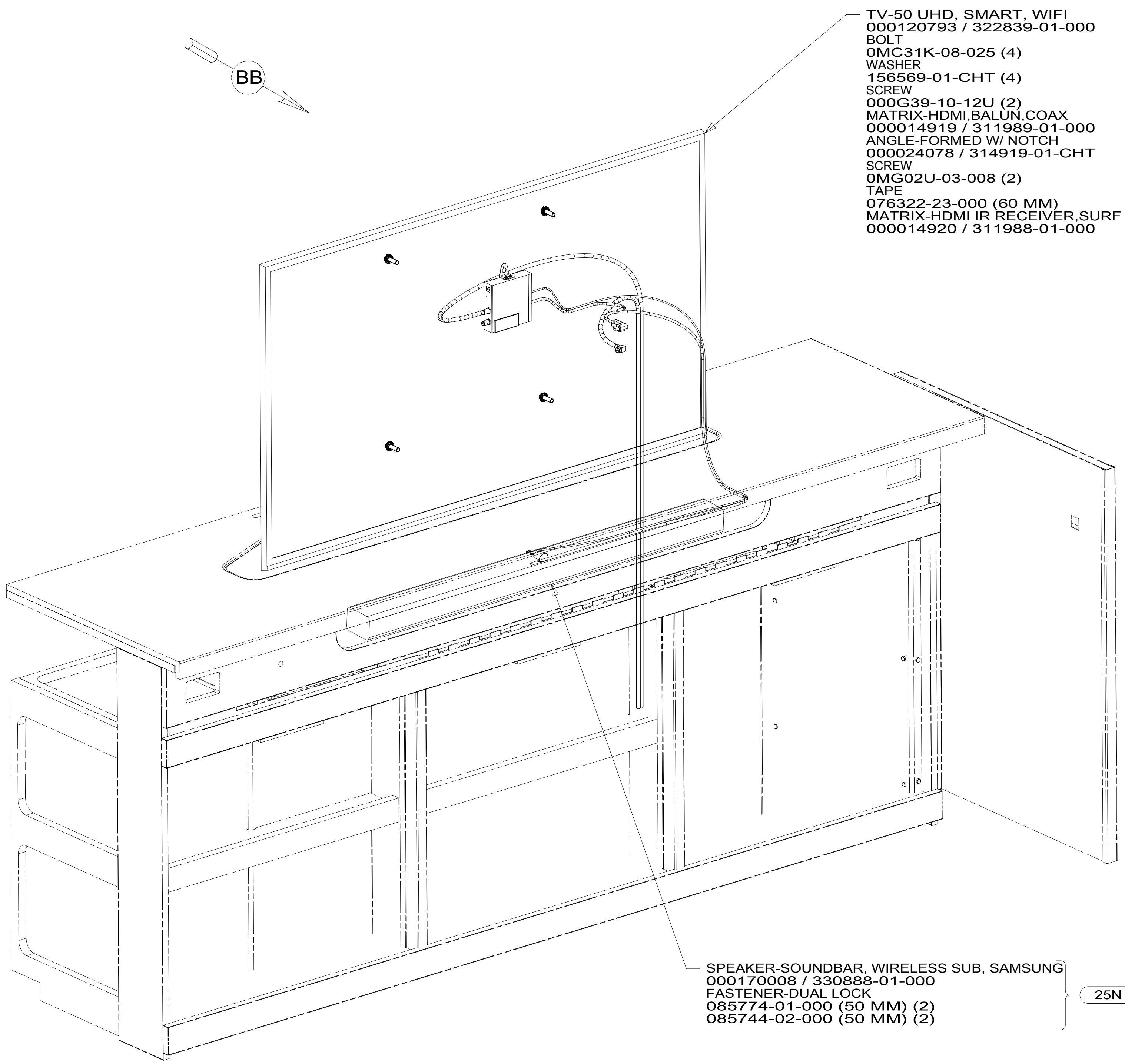
VIEW BA
