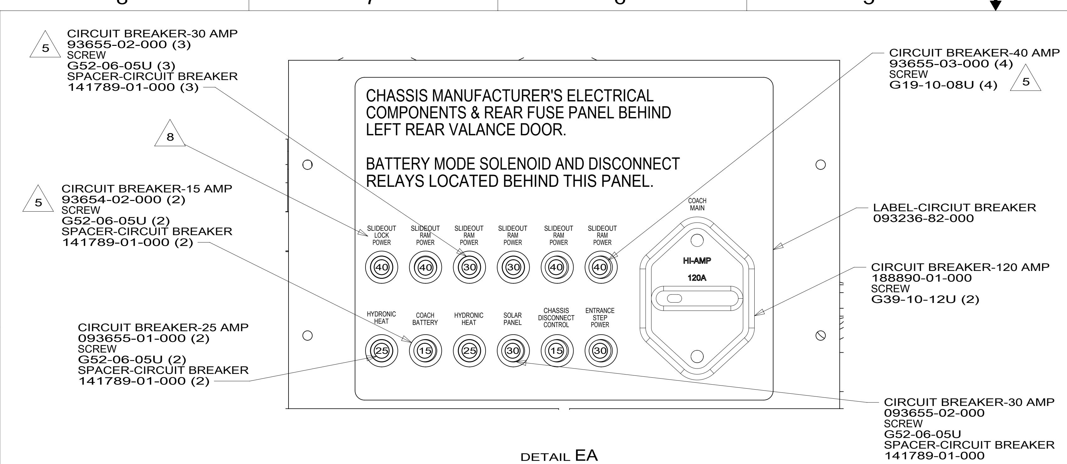
DETAIL EA
