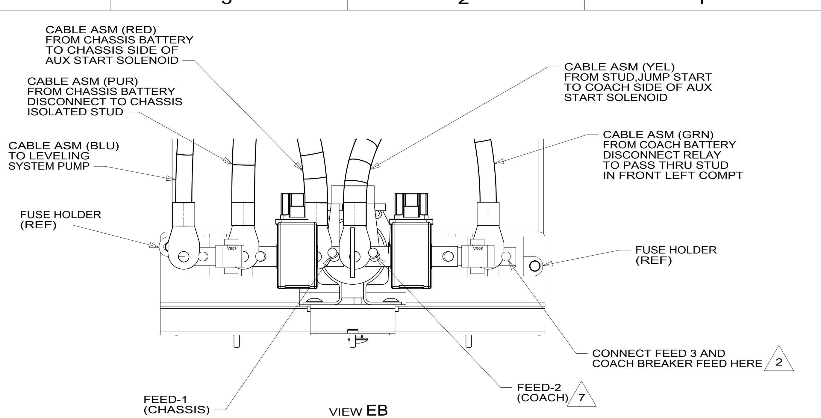
VIEW EB
