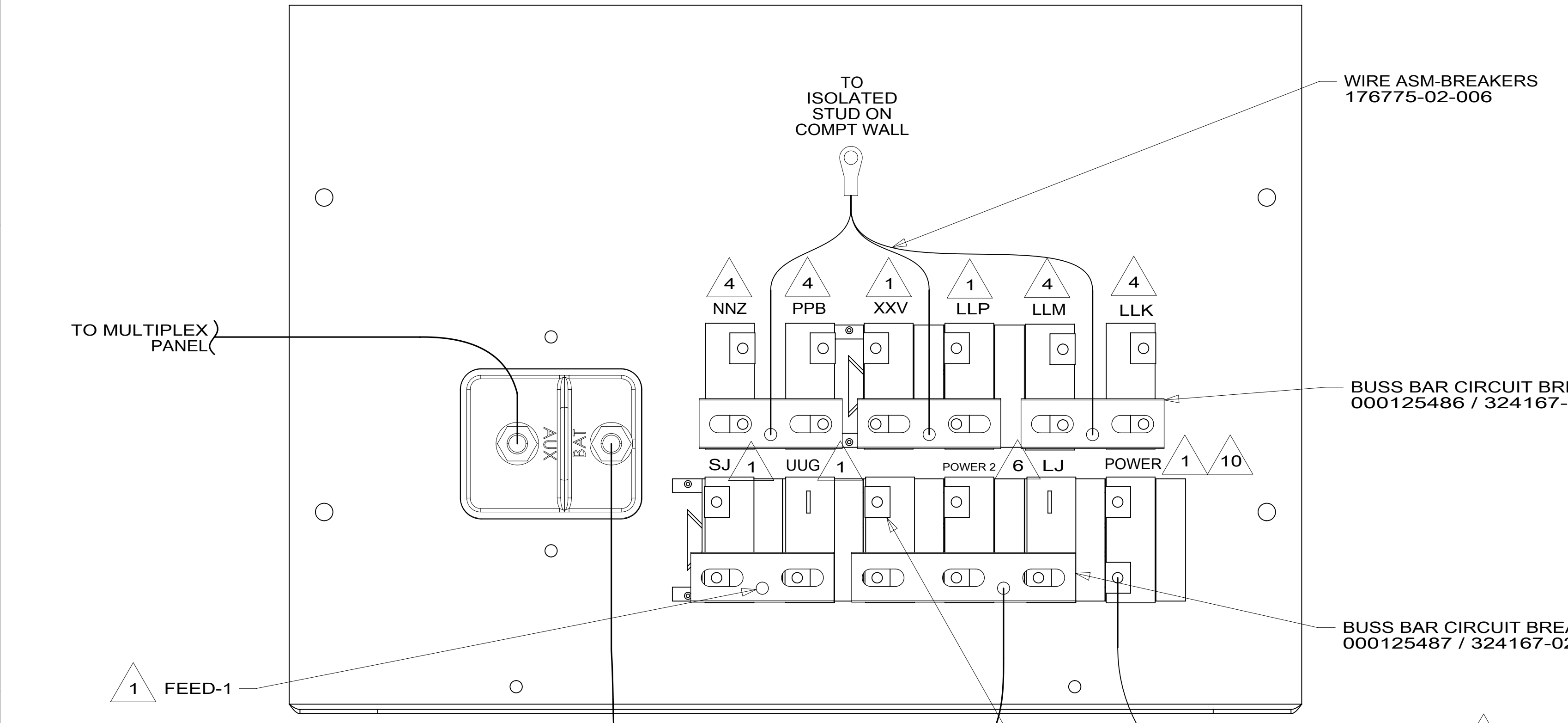
DETAIL EA
