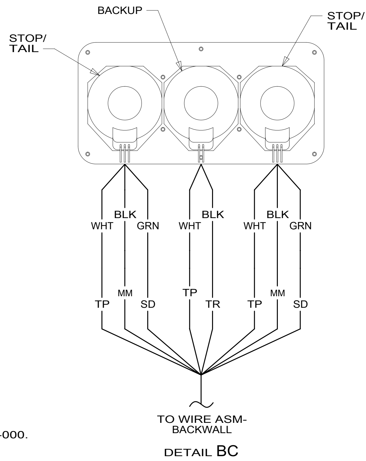
DETAIL BC
