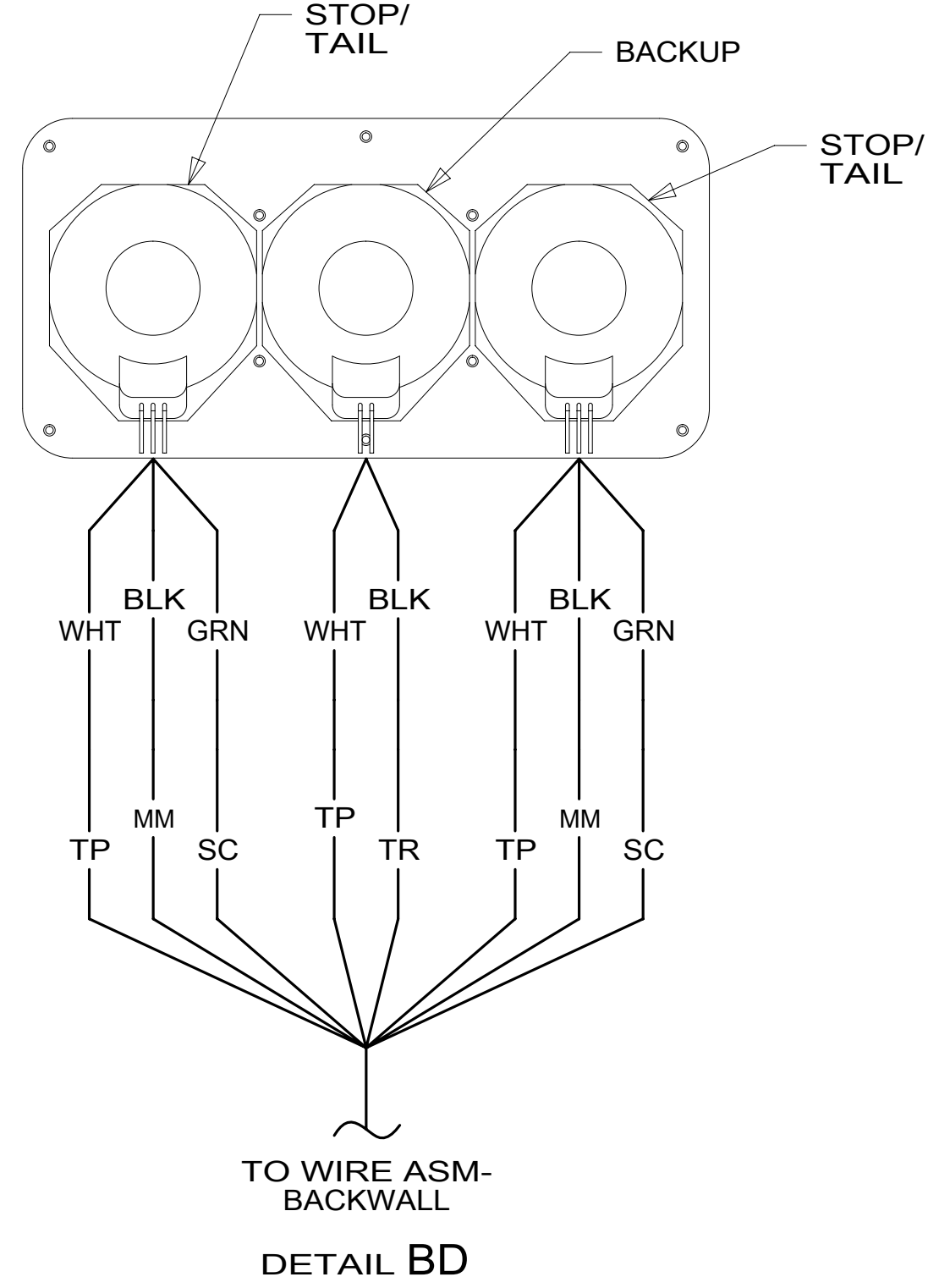
DETAIL BD
