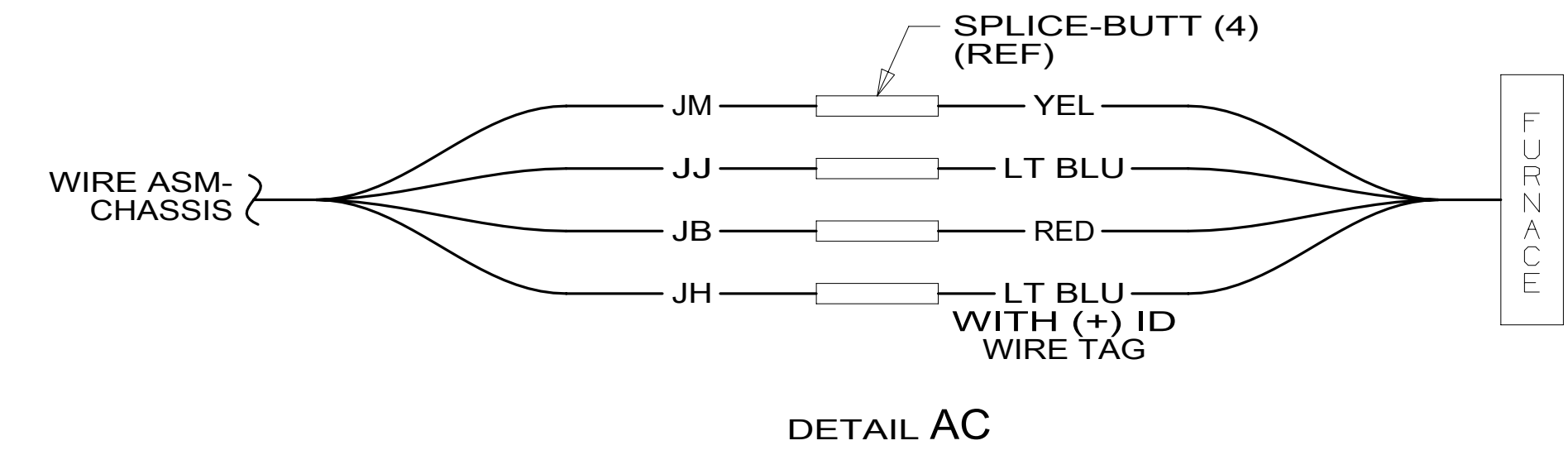
DETAIL AC
