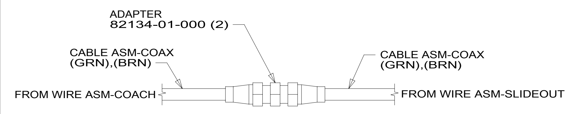
DETAIL DT
