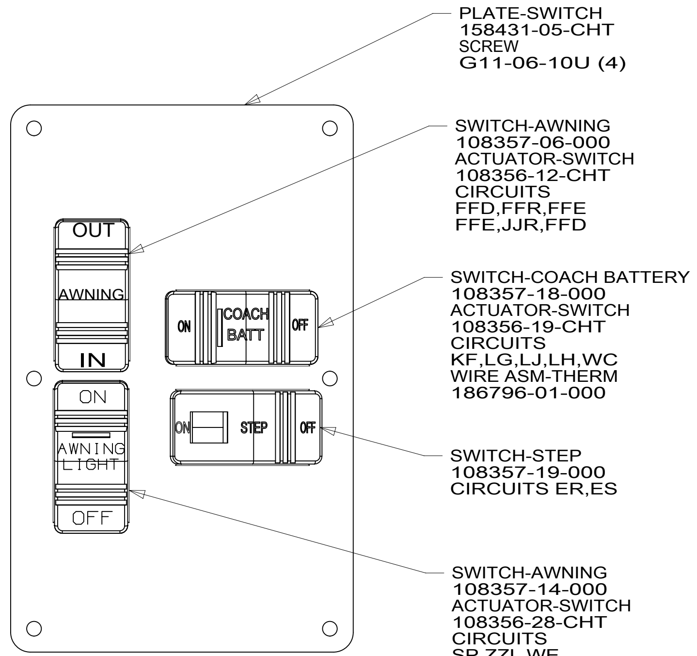
DETAIL DB 1
