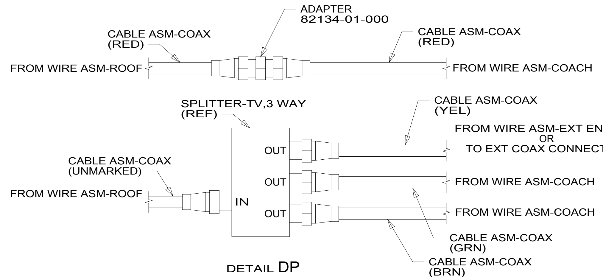
DETAIL DP
