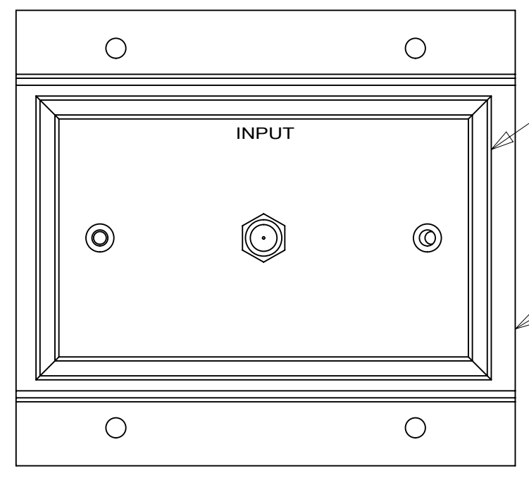
VIEW AA
