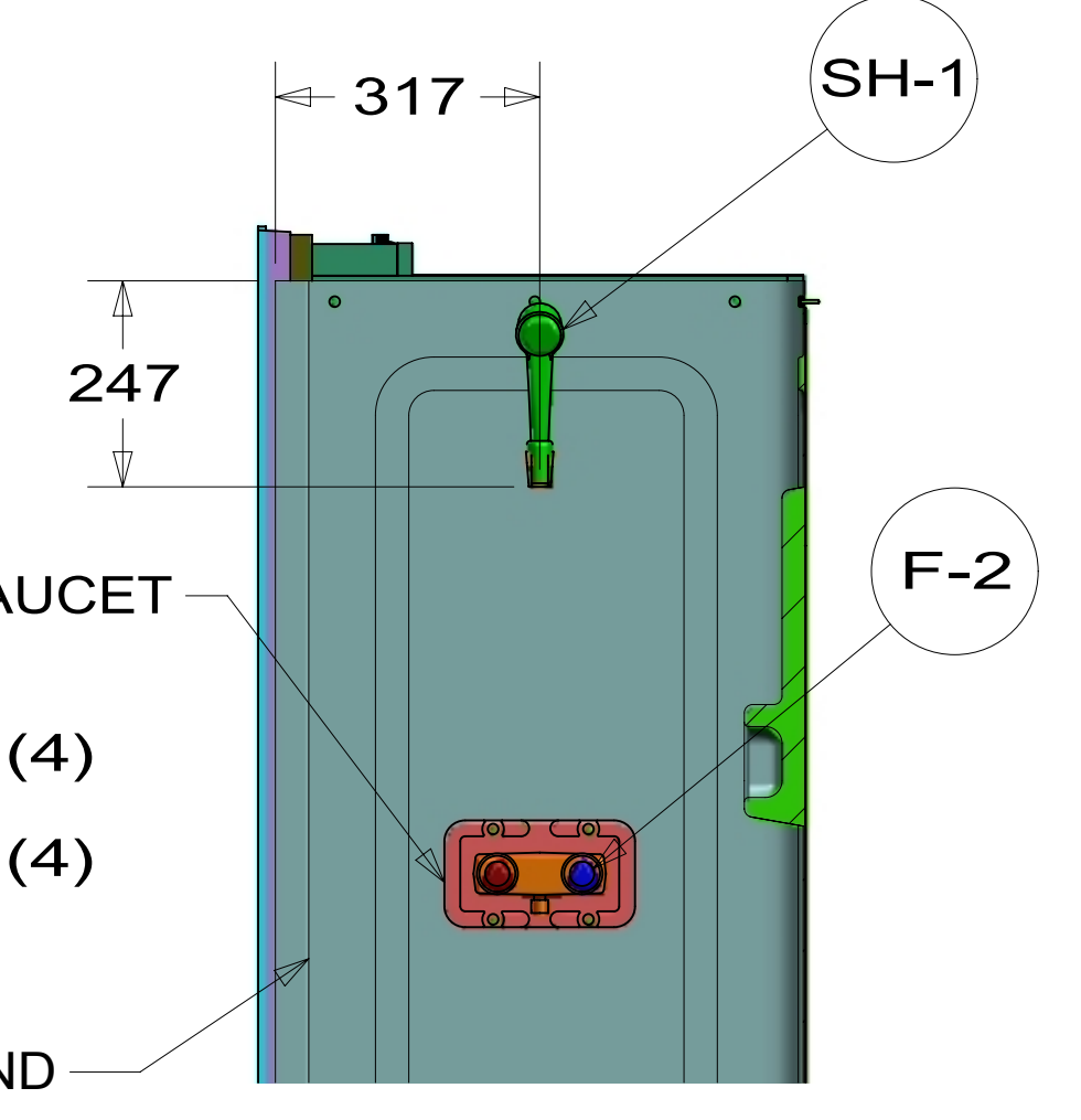
SECTION BE-BE
