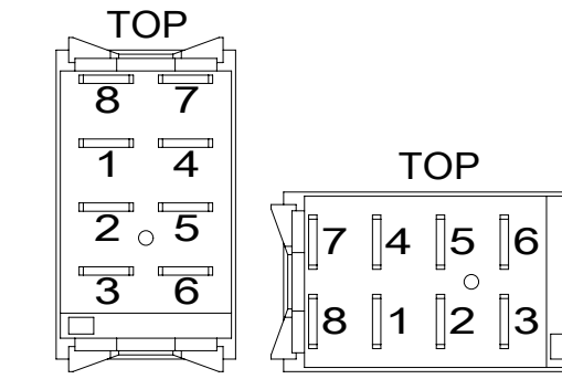
DETAIL DP
