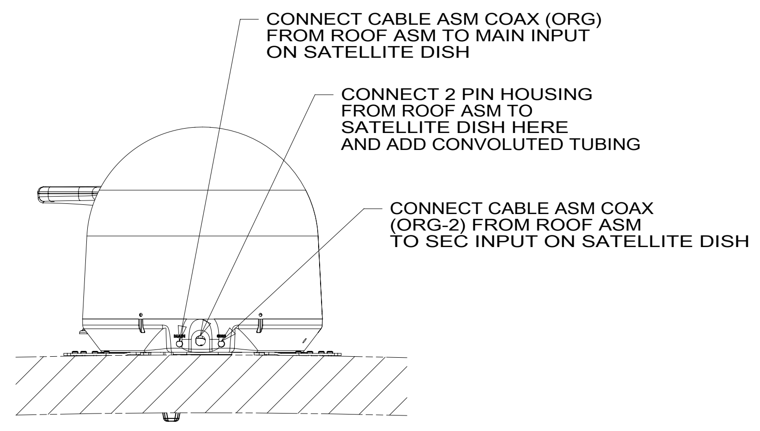
SECTION FC-FC
