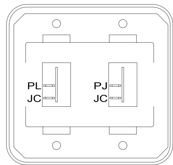
DETAIL DC
