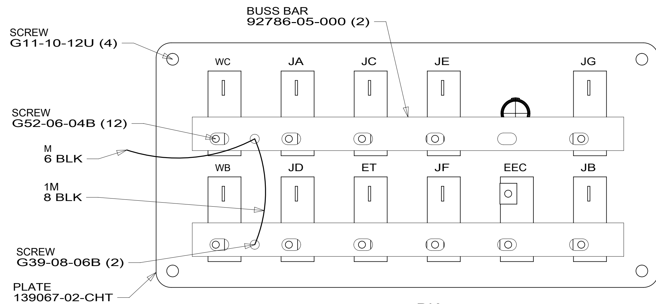
DETAIL DK (BACK VIEW)
