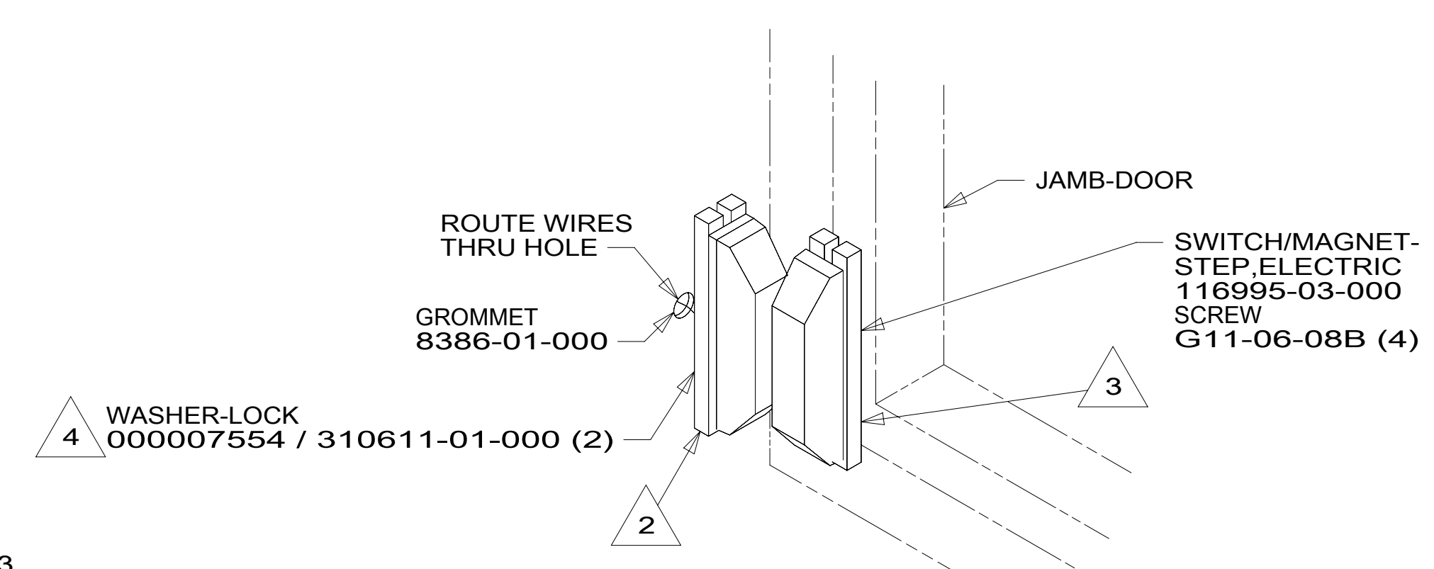
DETAIL CA
