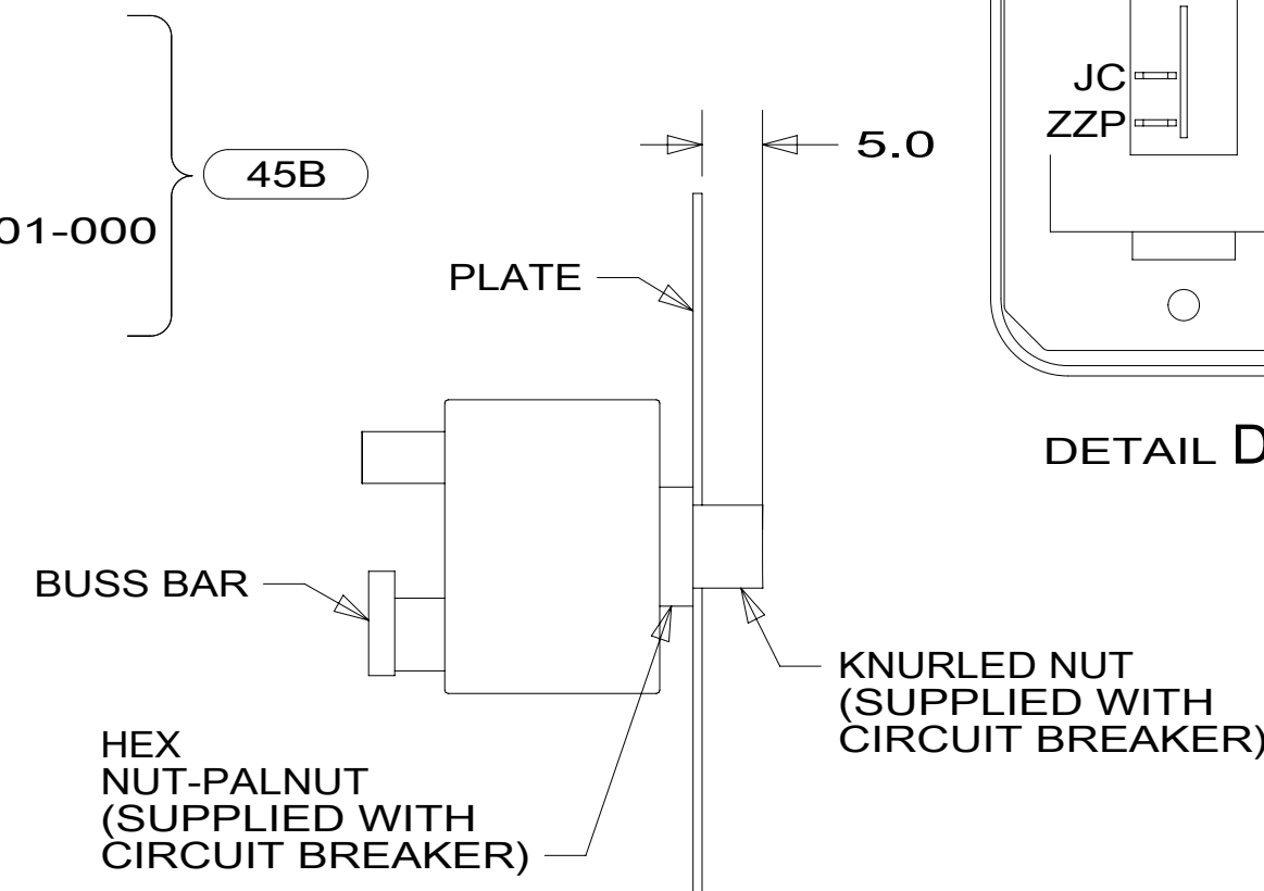
DETAIL DL-DL
