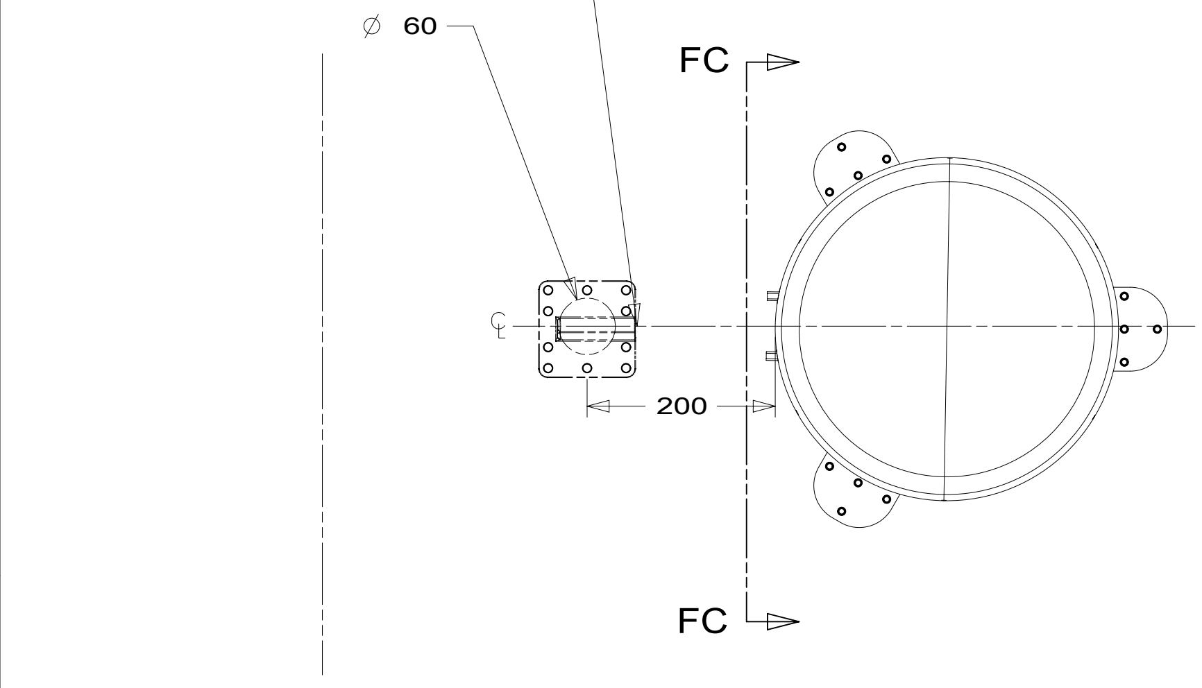
DETAIL FB
