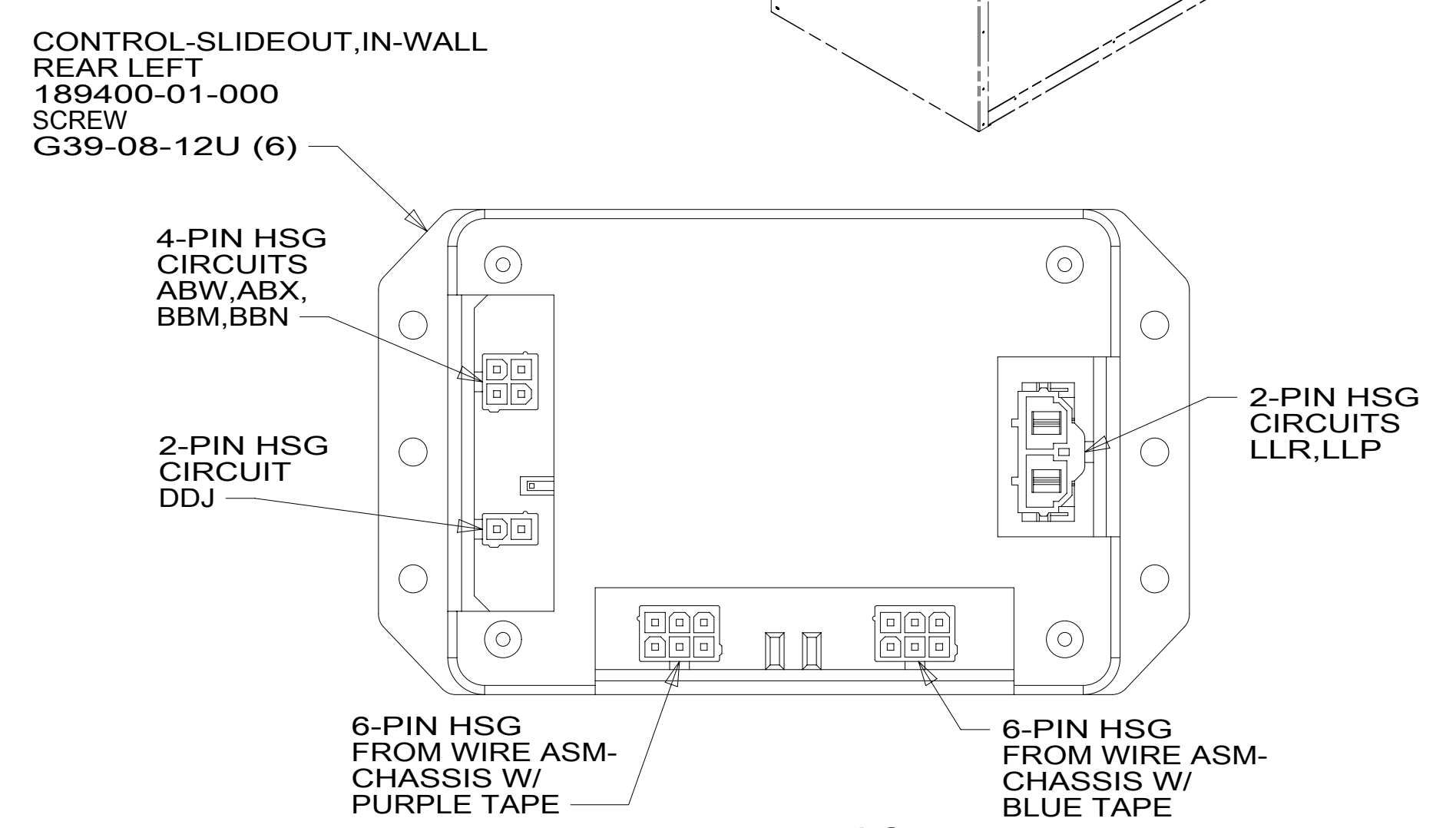
DETAIL AC
