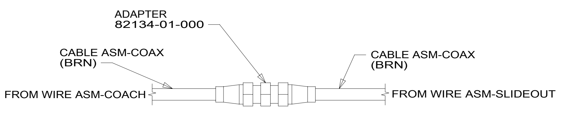
DETAIL DB 1
