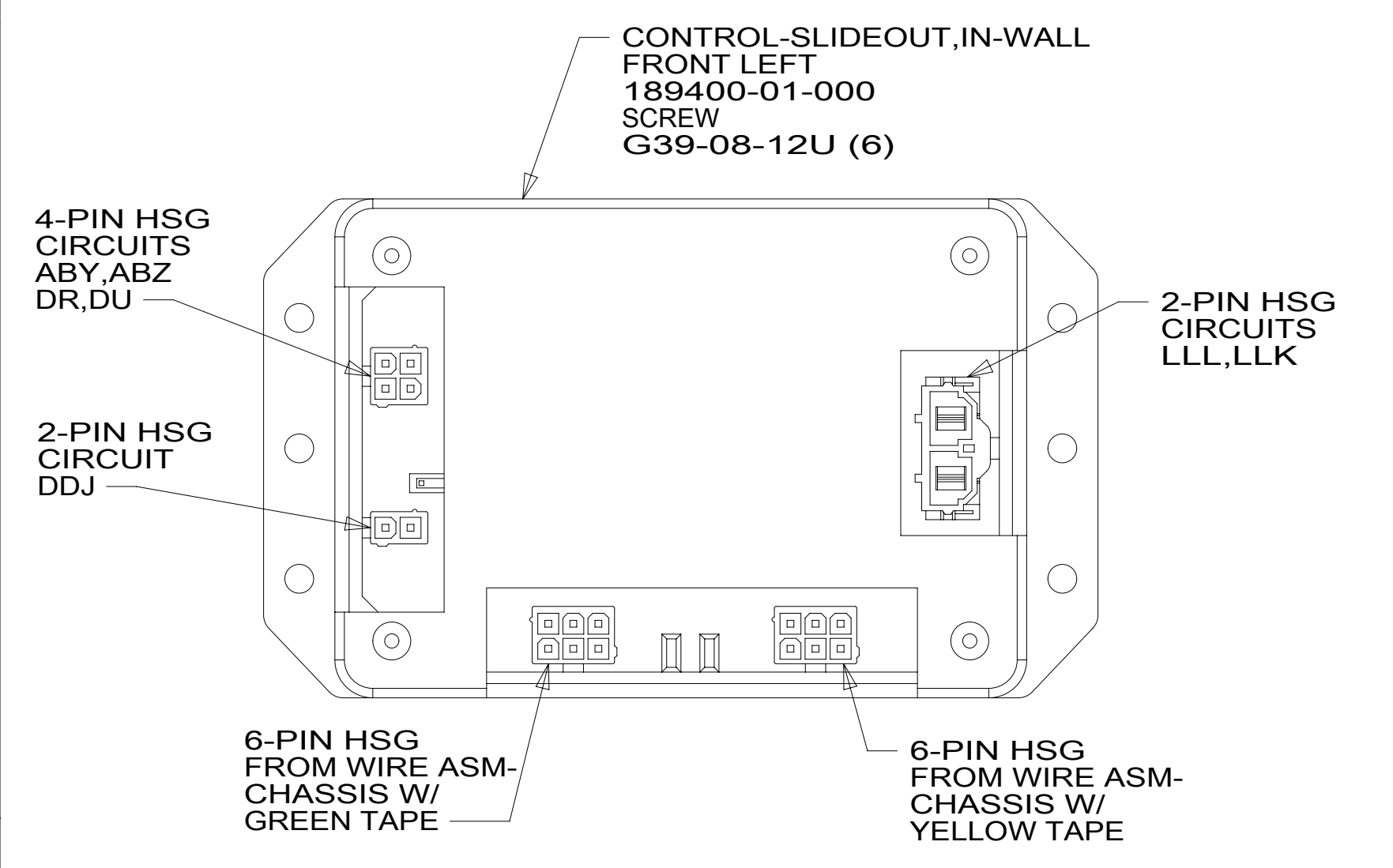
DETAIL AB
