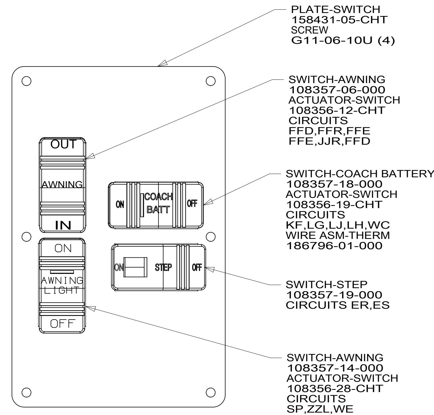
DETAIL DB 1
