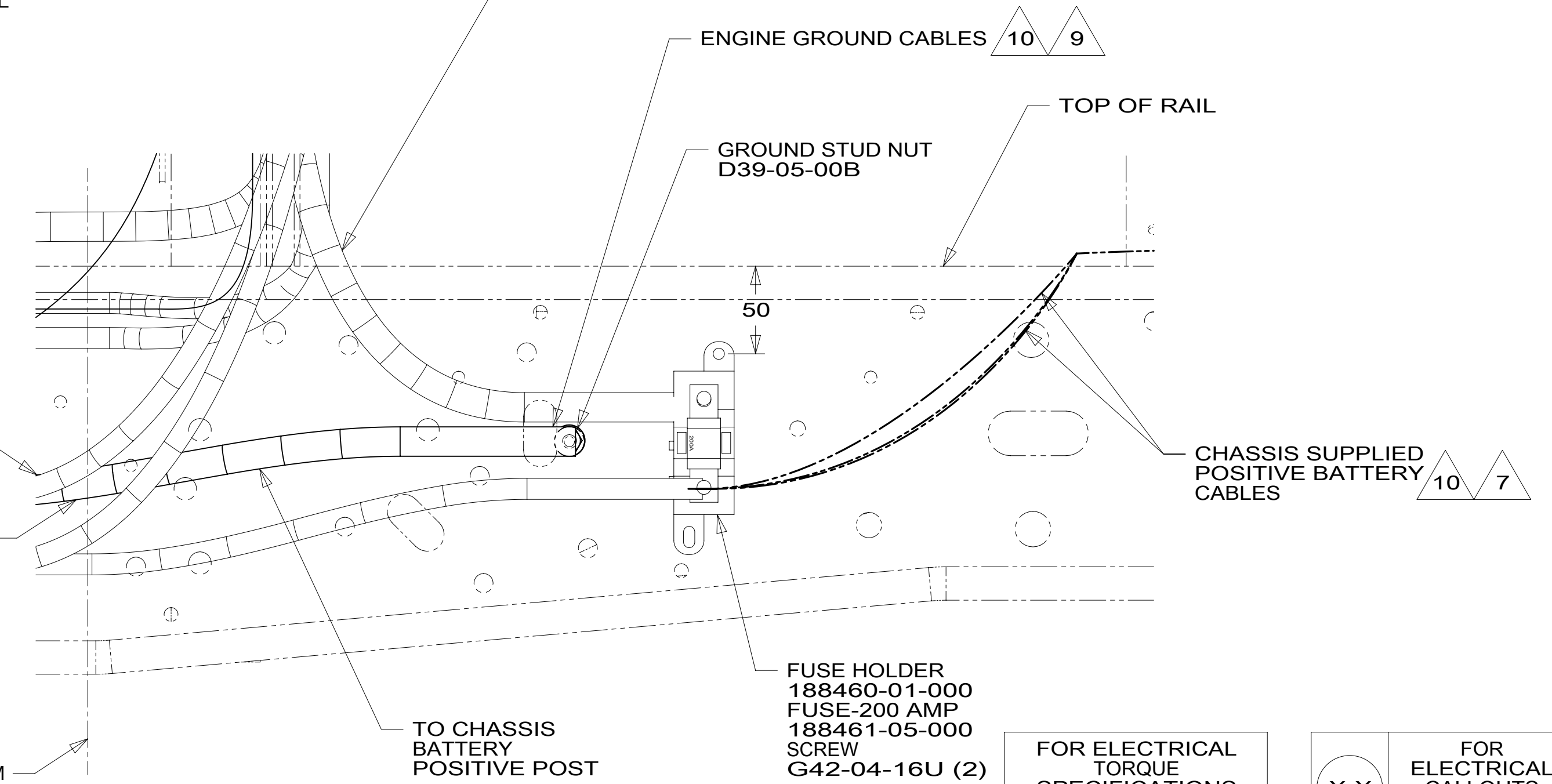
VIEW AA
