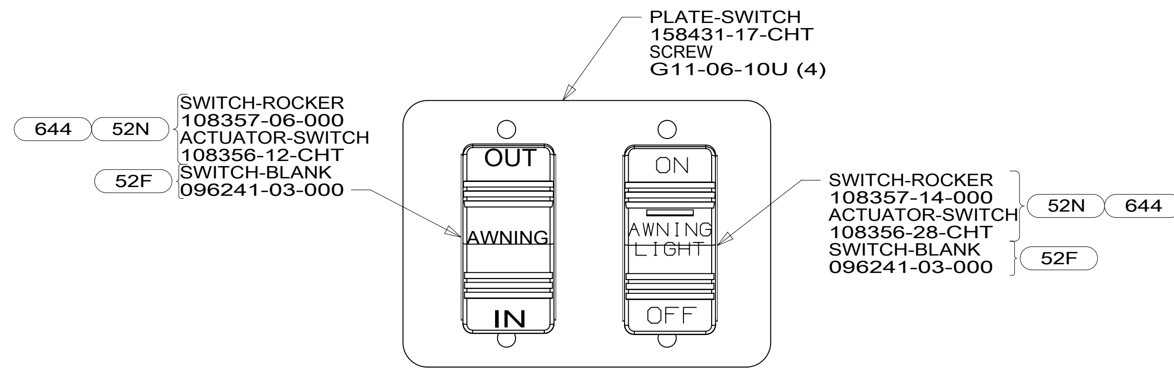
DETAIL CD
