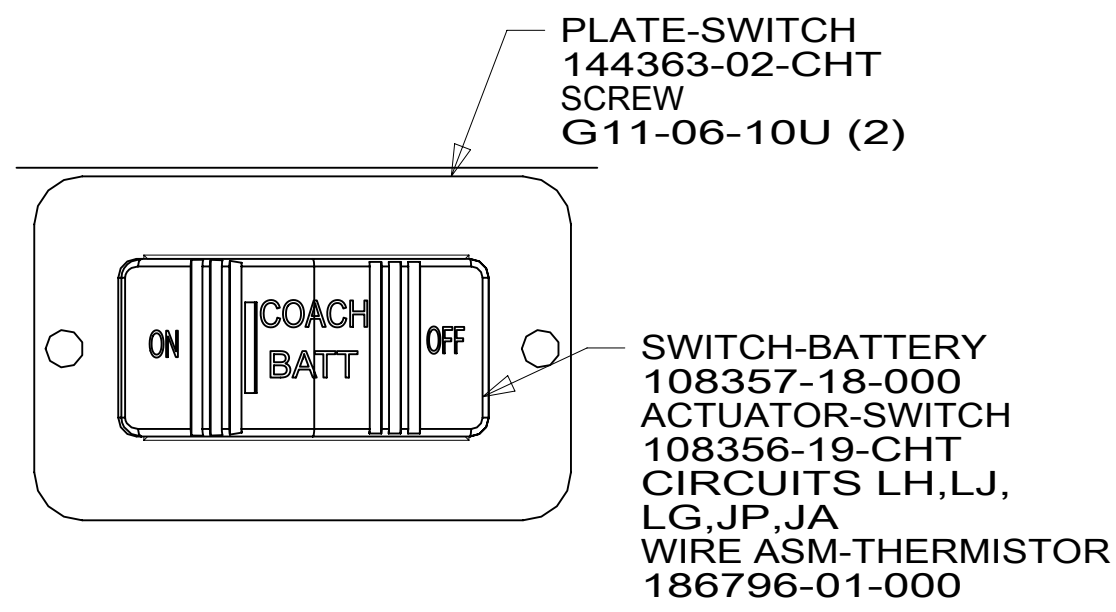
DETAIL CA
