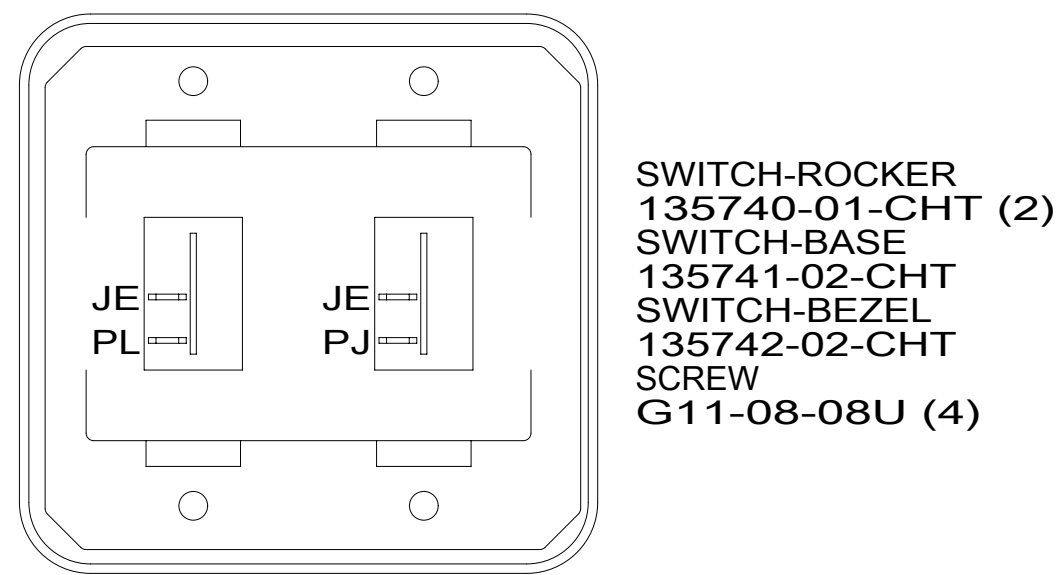
DETAIL CB
