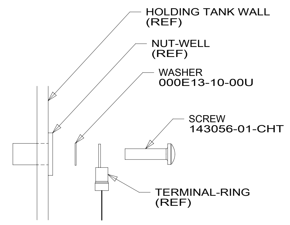
DETAIL AC 6
