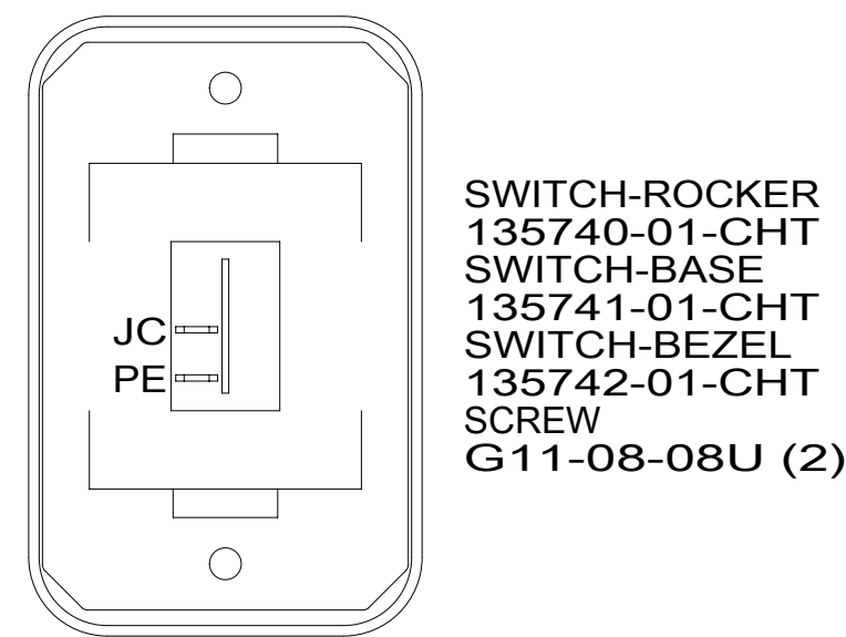
DETAIL CC
