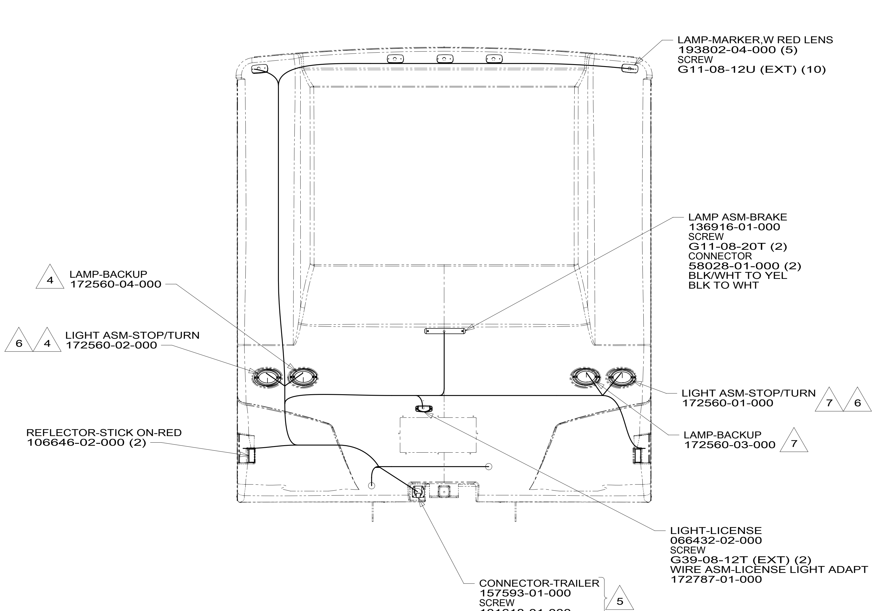
VIEW BB
