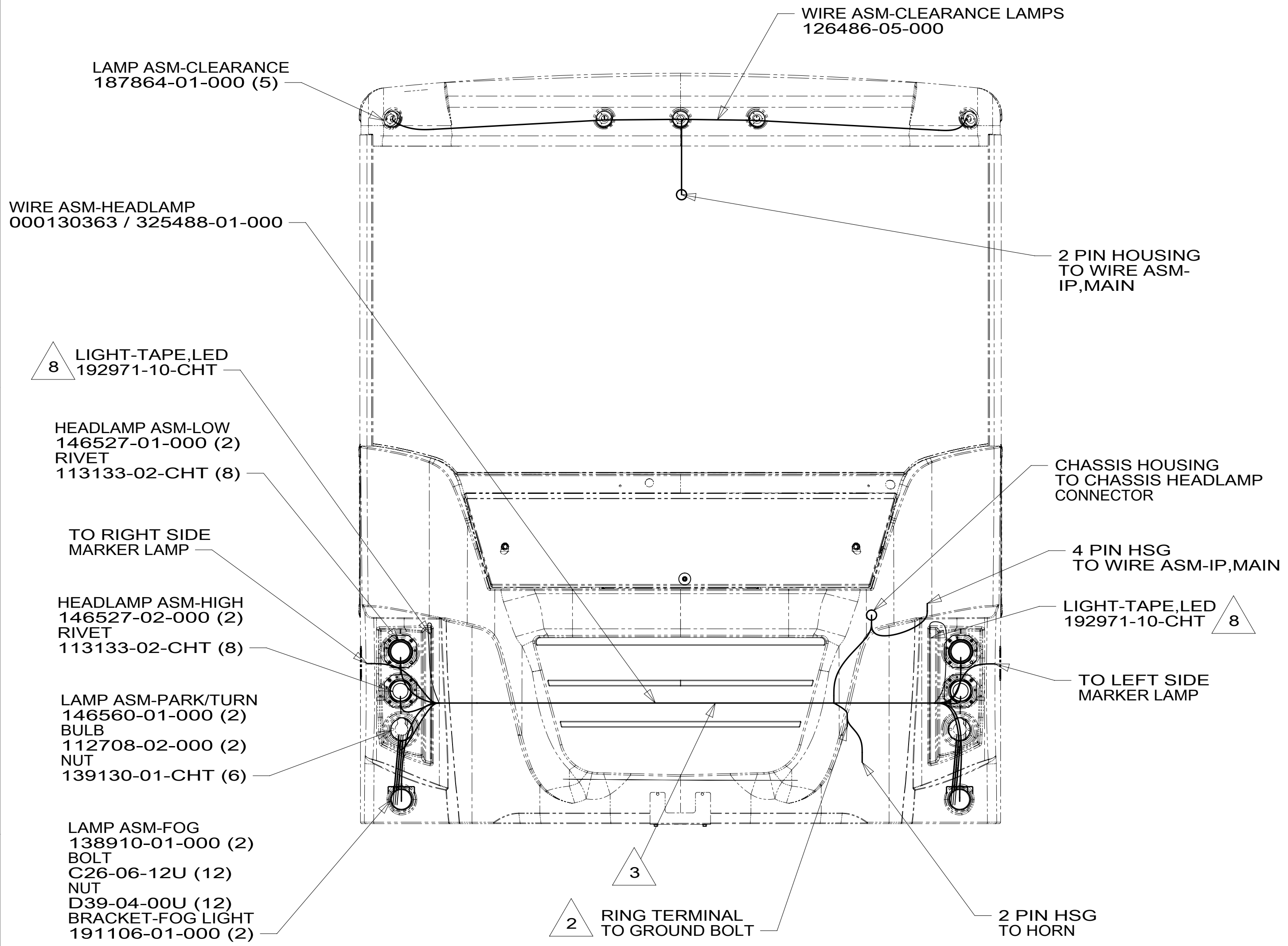
VIEW BA
