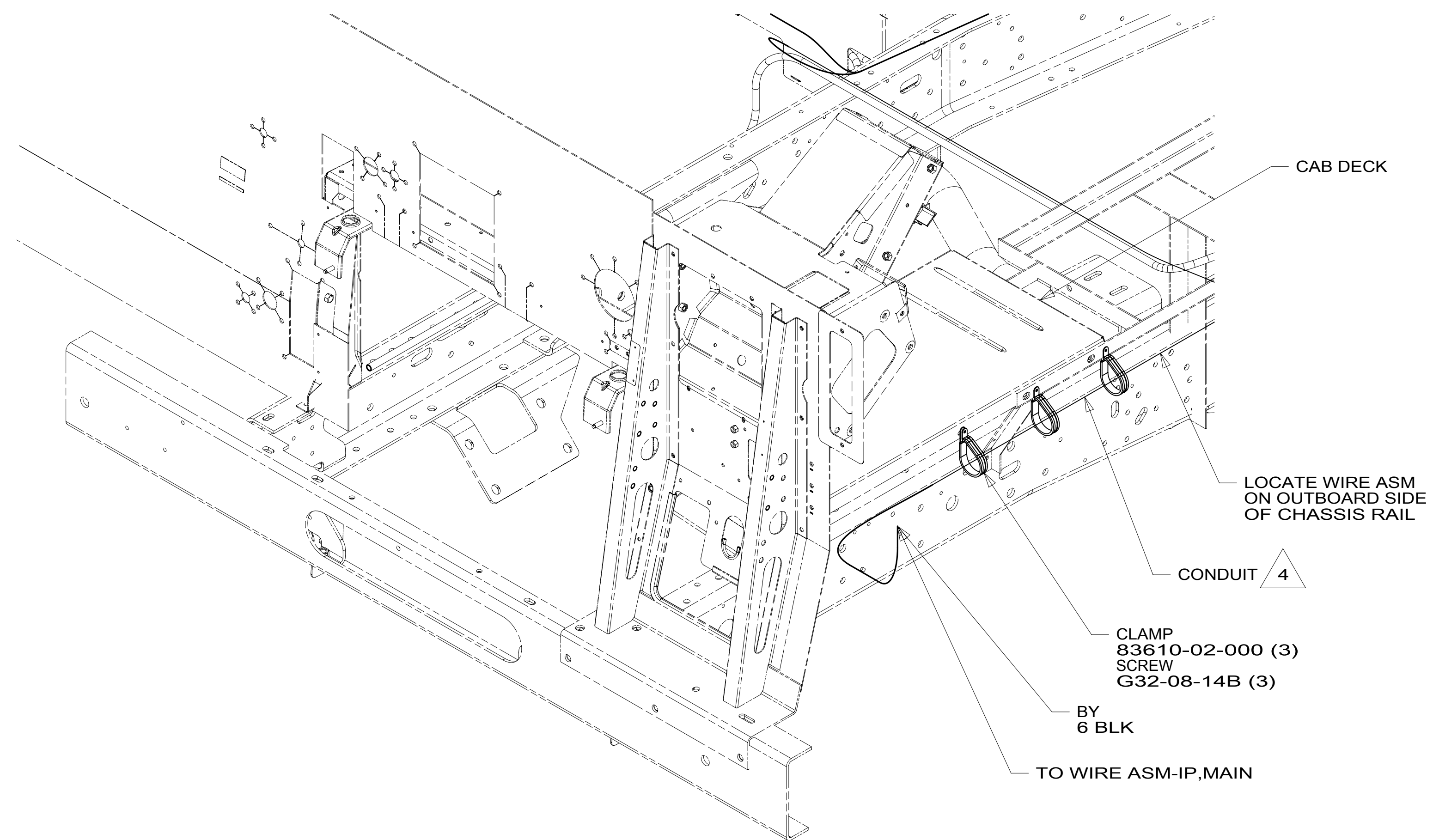
VIEW BA
