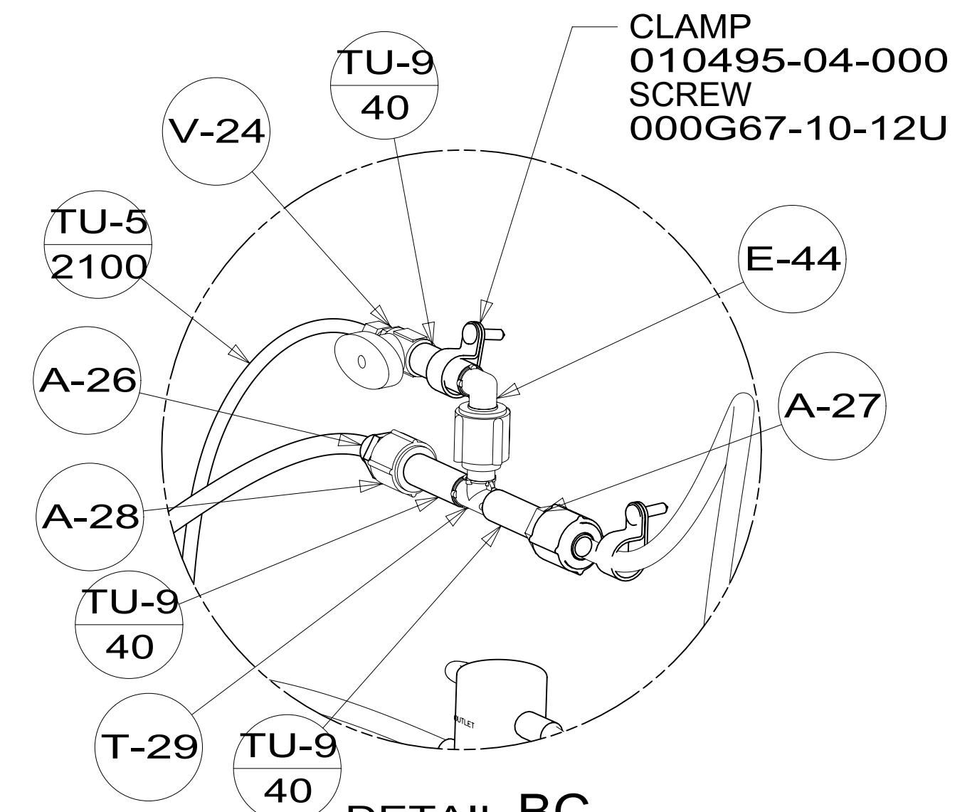
DETAIL BC (SHOWN W/OUT CABINETS) 29B & 79W
