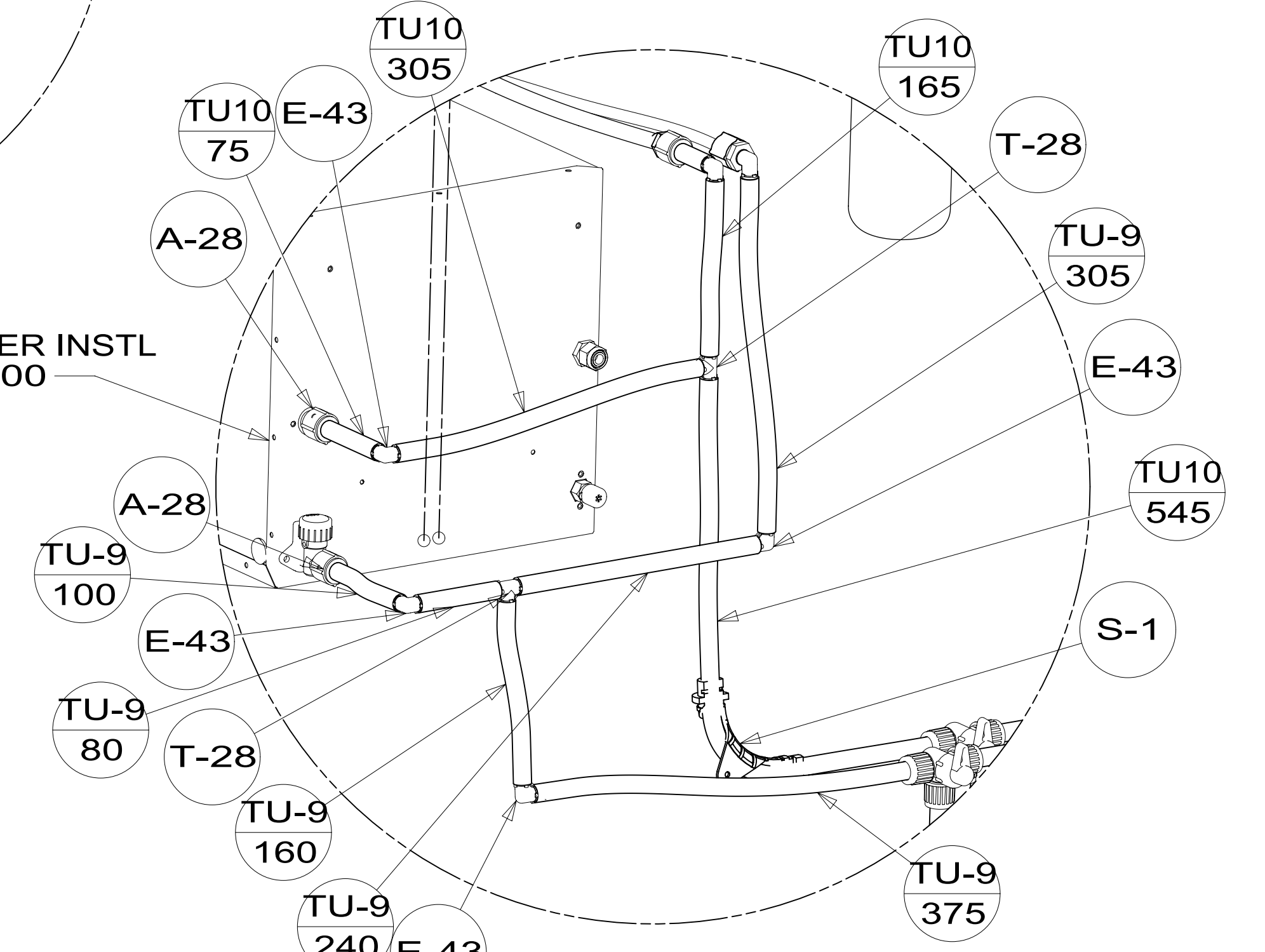
DETAIL BB (SHOWN W/OUT CABINETS & FLOOR) 1BT
