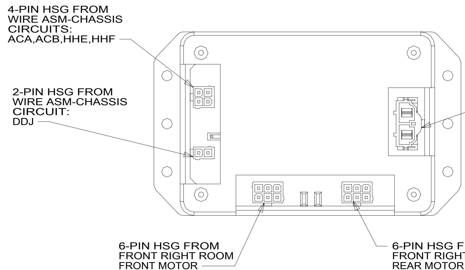
DETAIL GC
