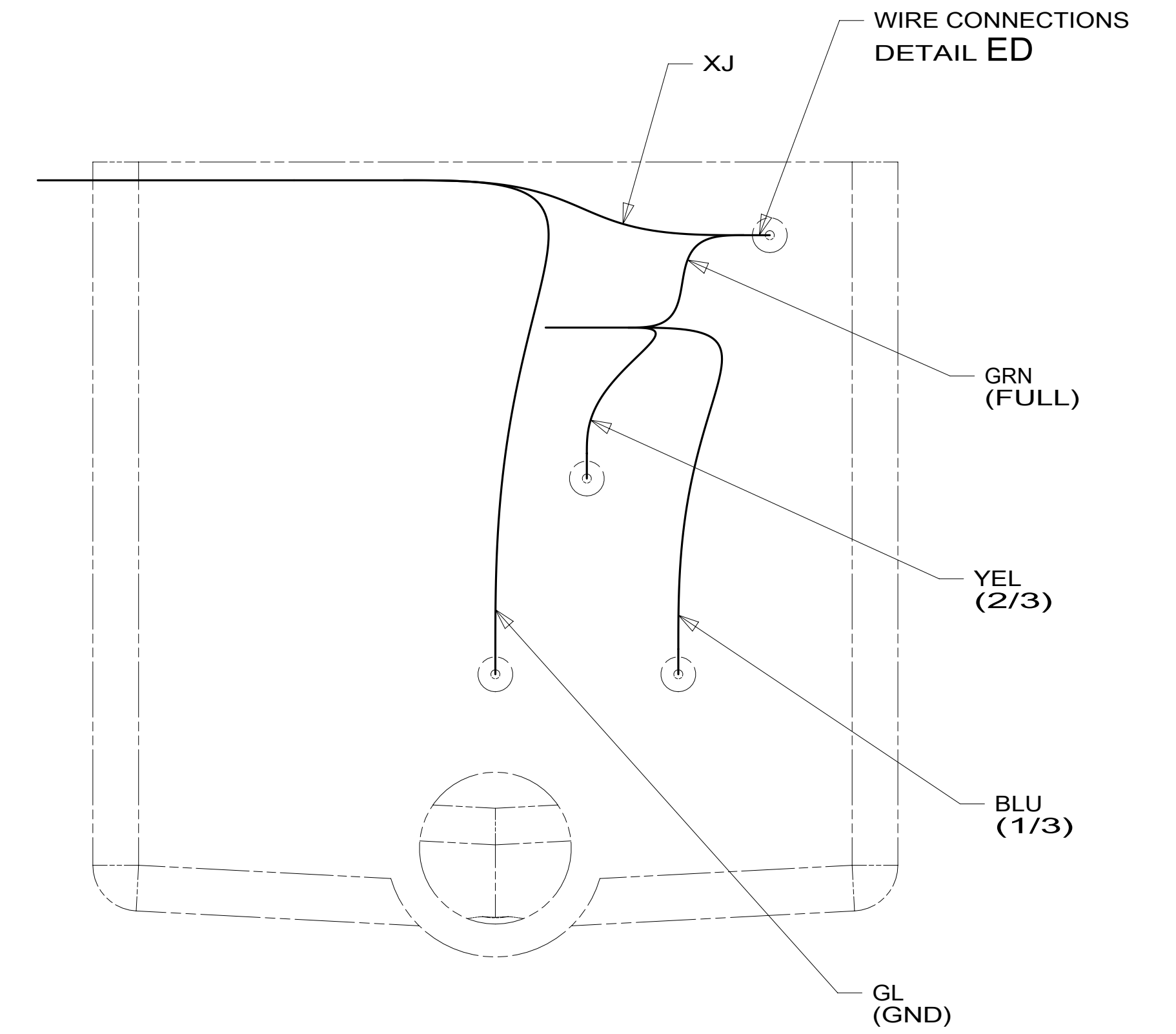
VIEW EC
