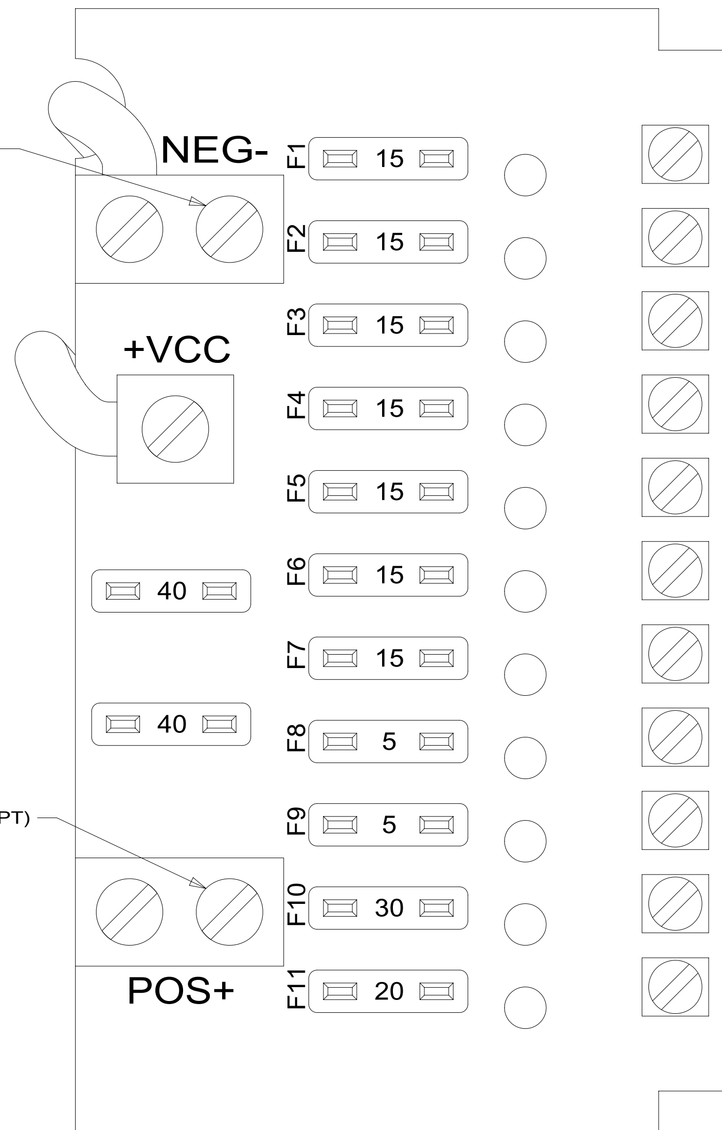
DETAIL CG 1
