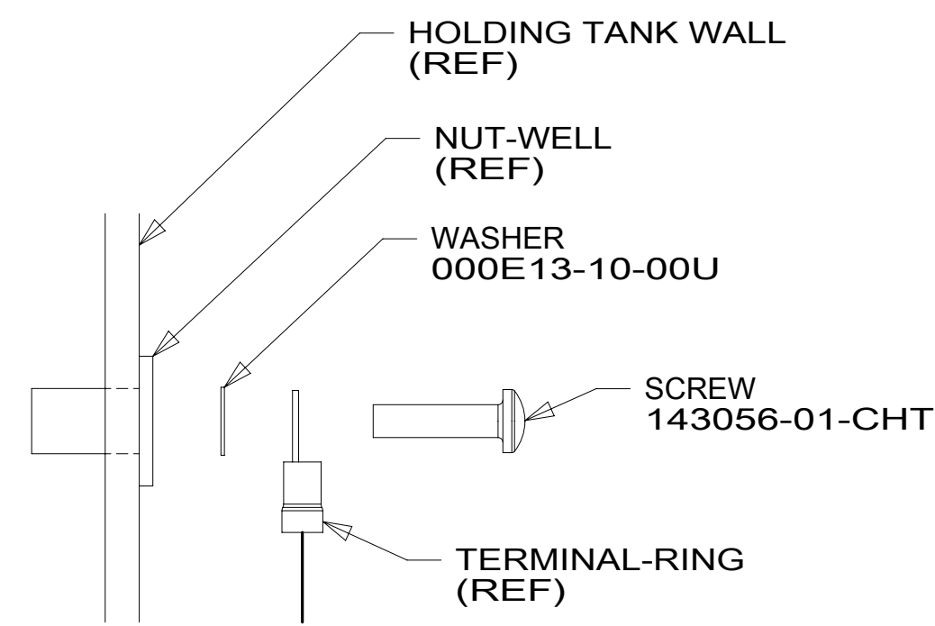
DETAIL ED 1
