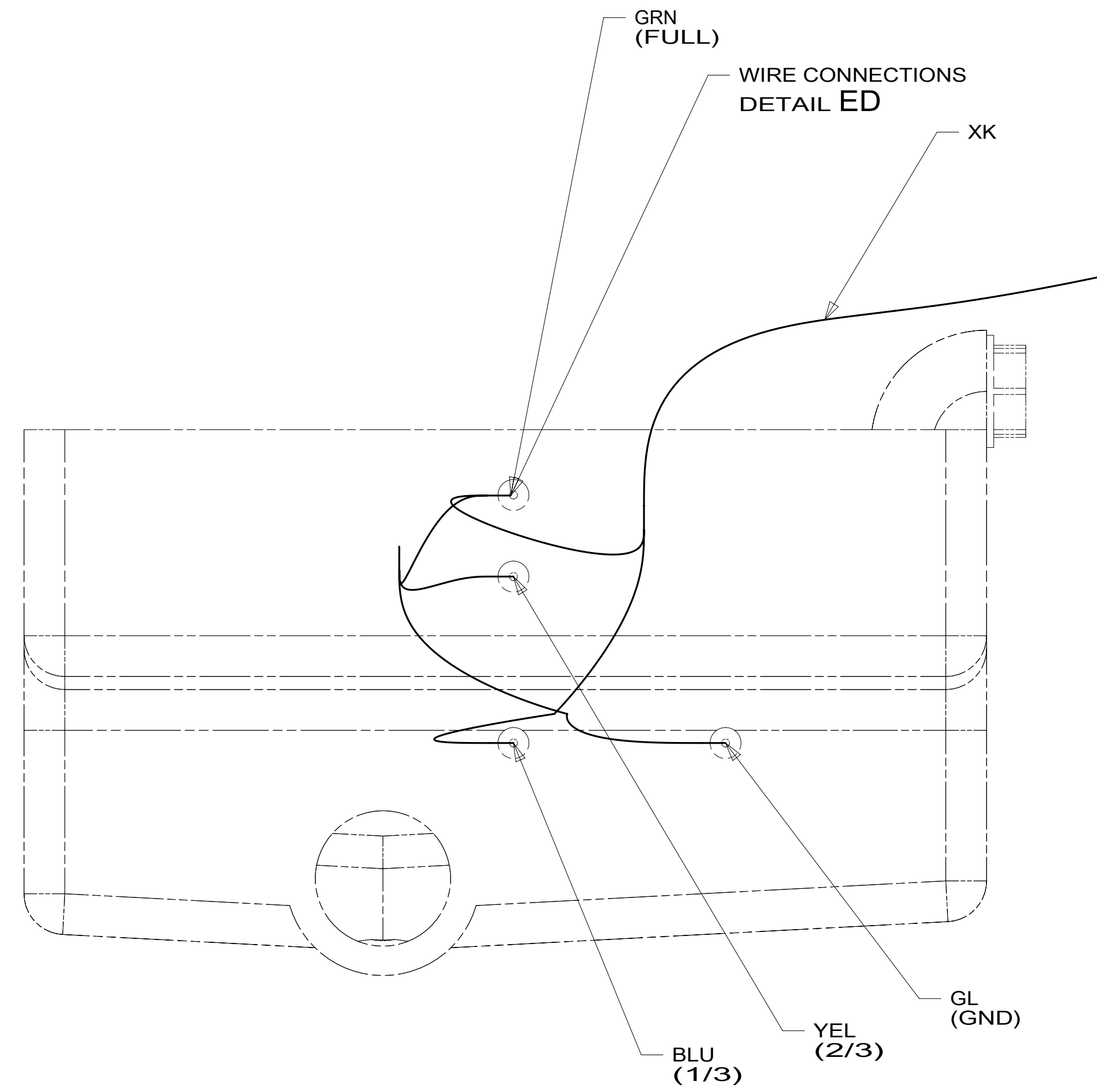
VIEW EB
