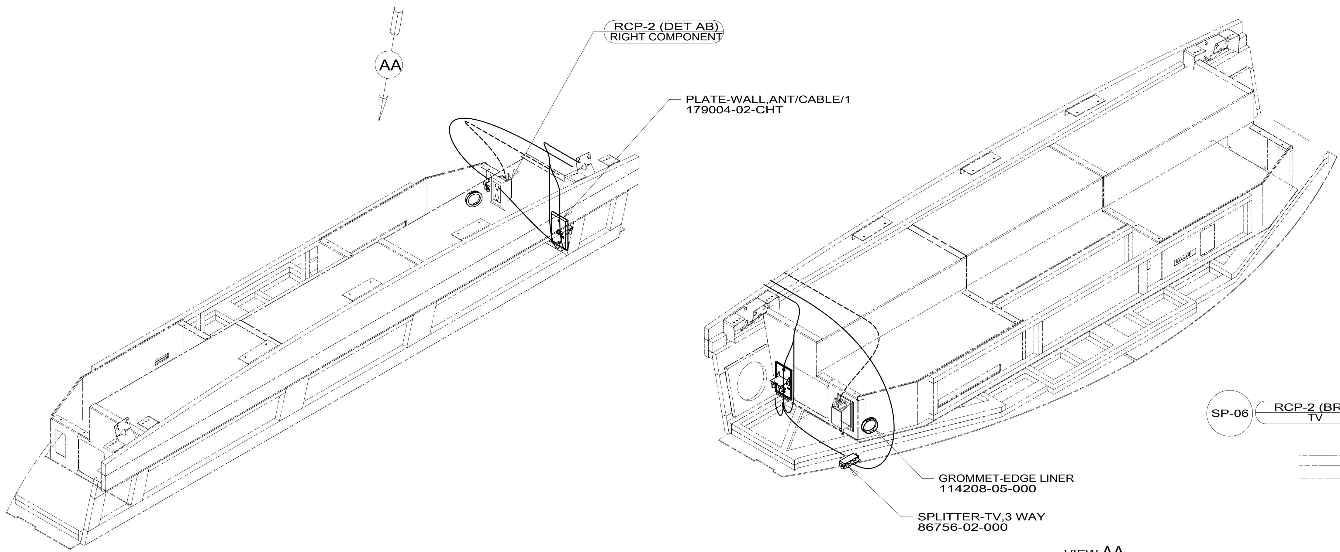
VIEW AA
