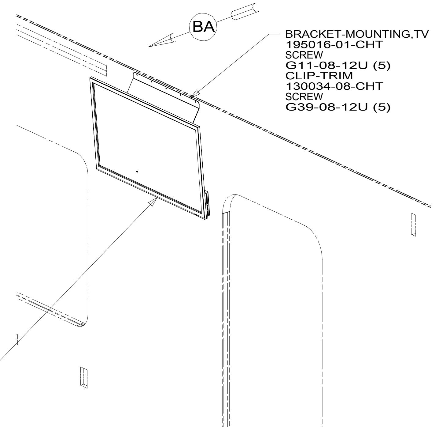
VIEW AA
