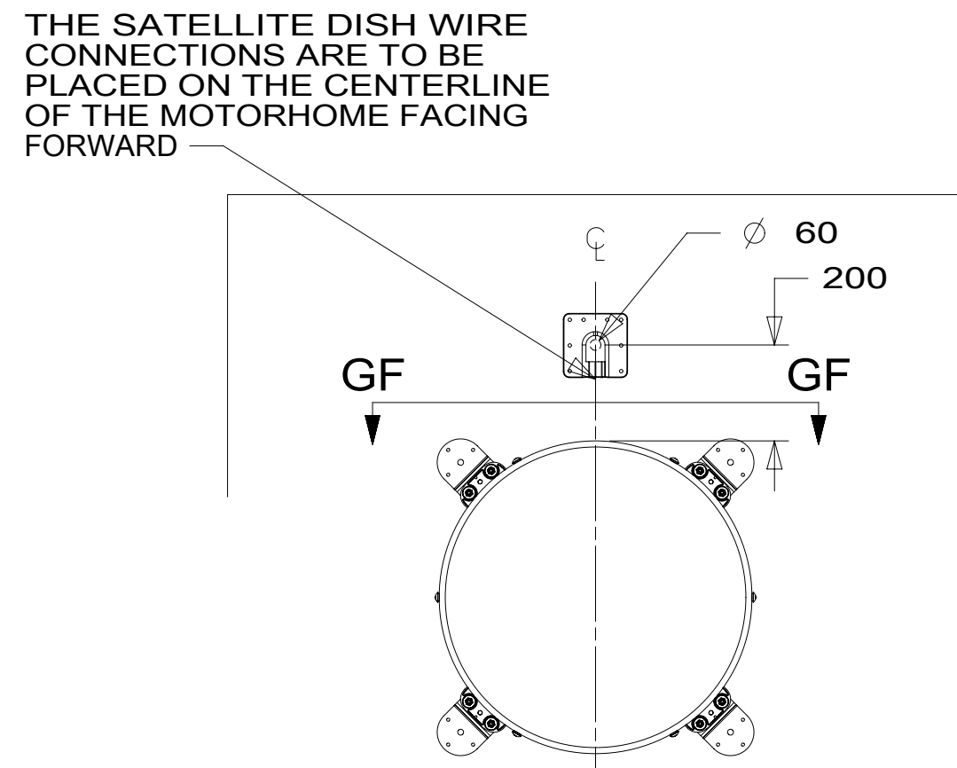
DETAIL GE 2
