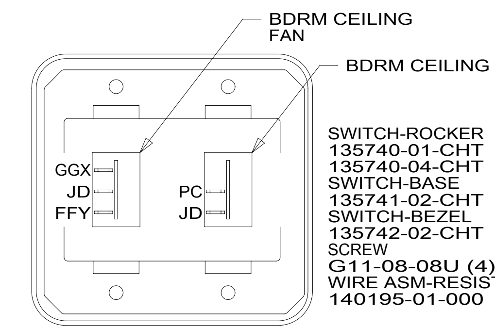
DETAIL EC
