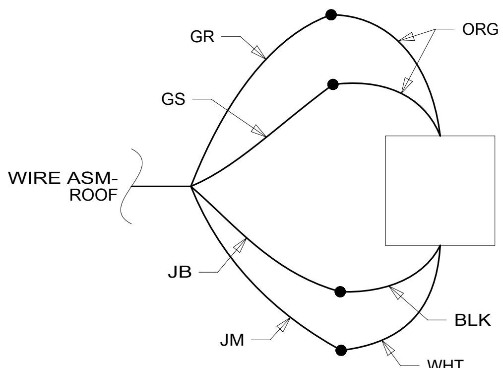
DETAIL GC
