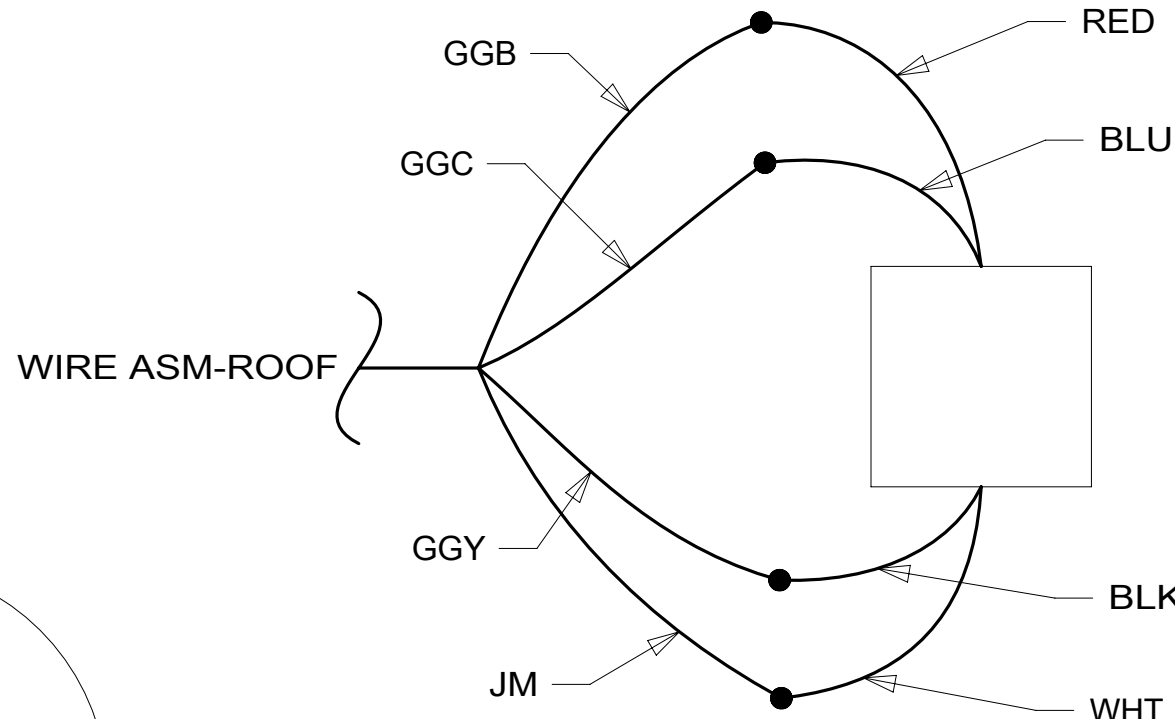
DETAIL GA
