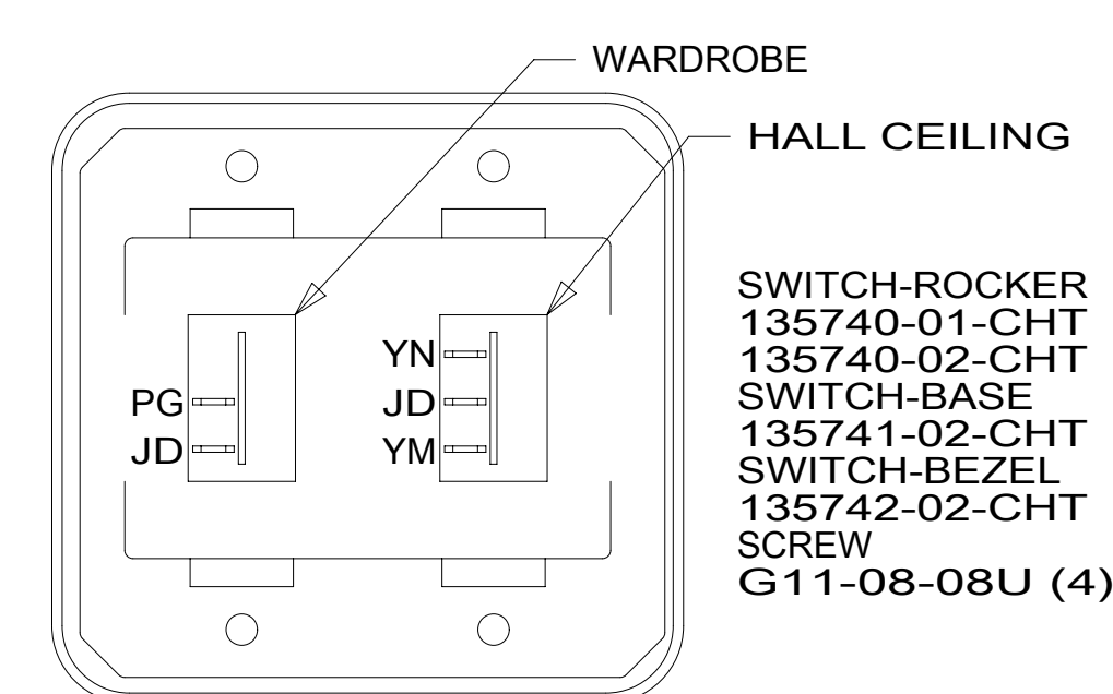
DETAIL EE
