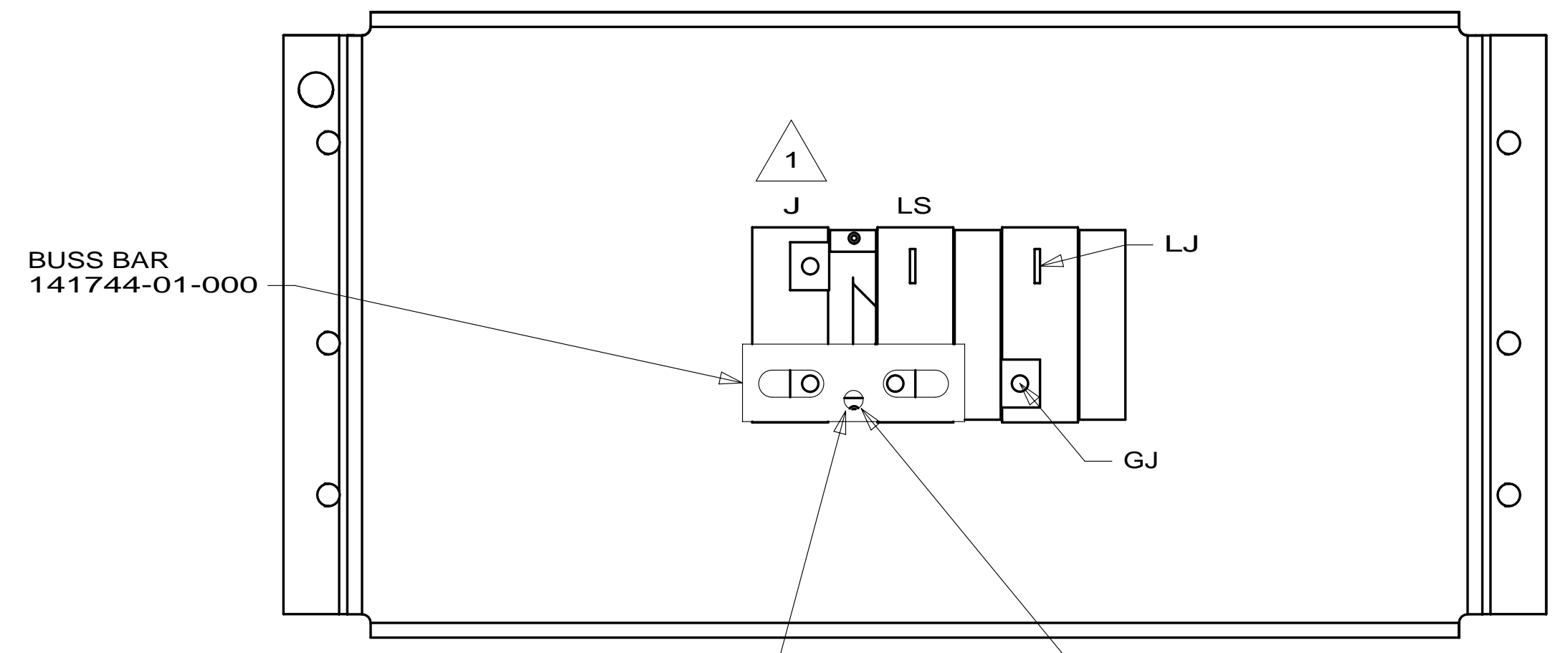
VIEW BB
