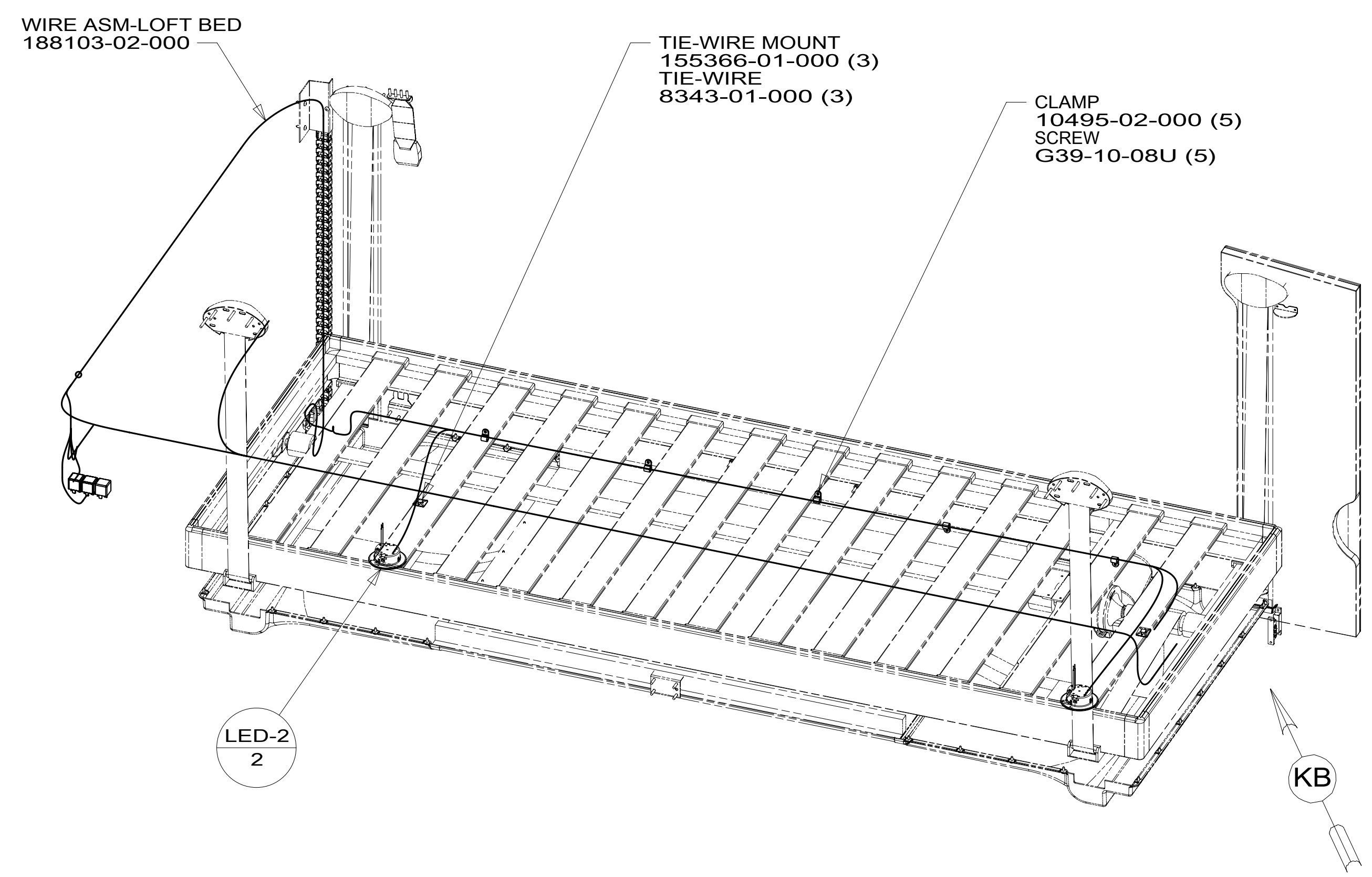
DETAIL KA 45B
