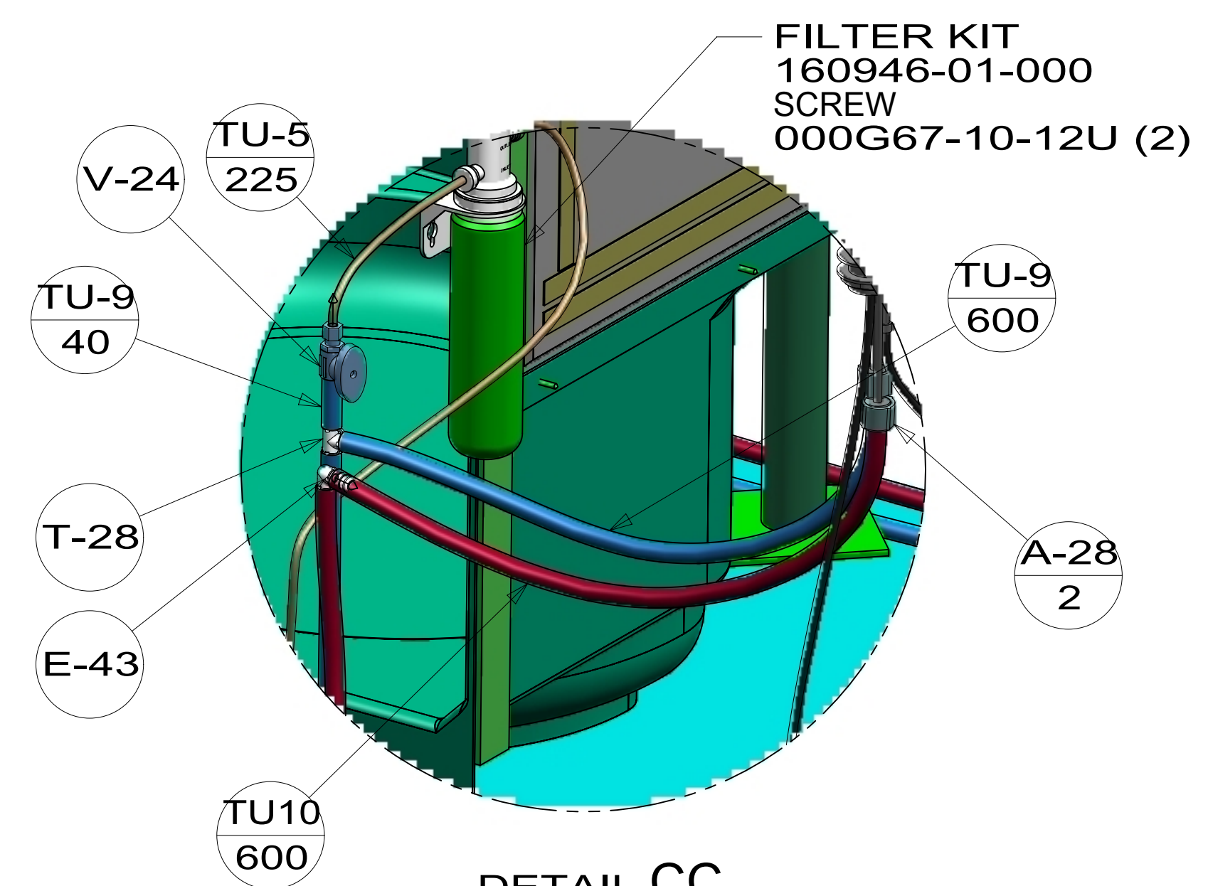
DETAIL CC (SHOWN W/OUT CABINETS)
