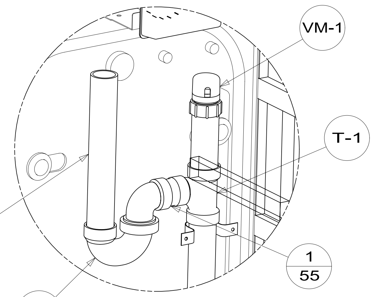
DETAIL CD 21S
