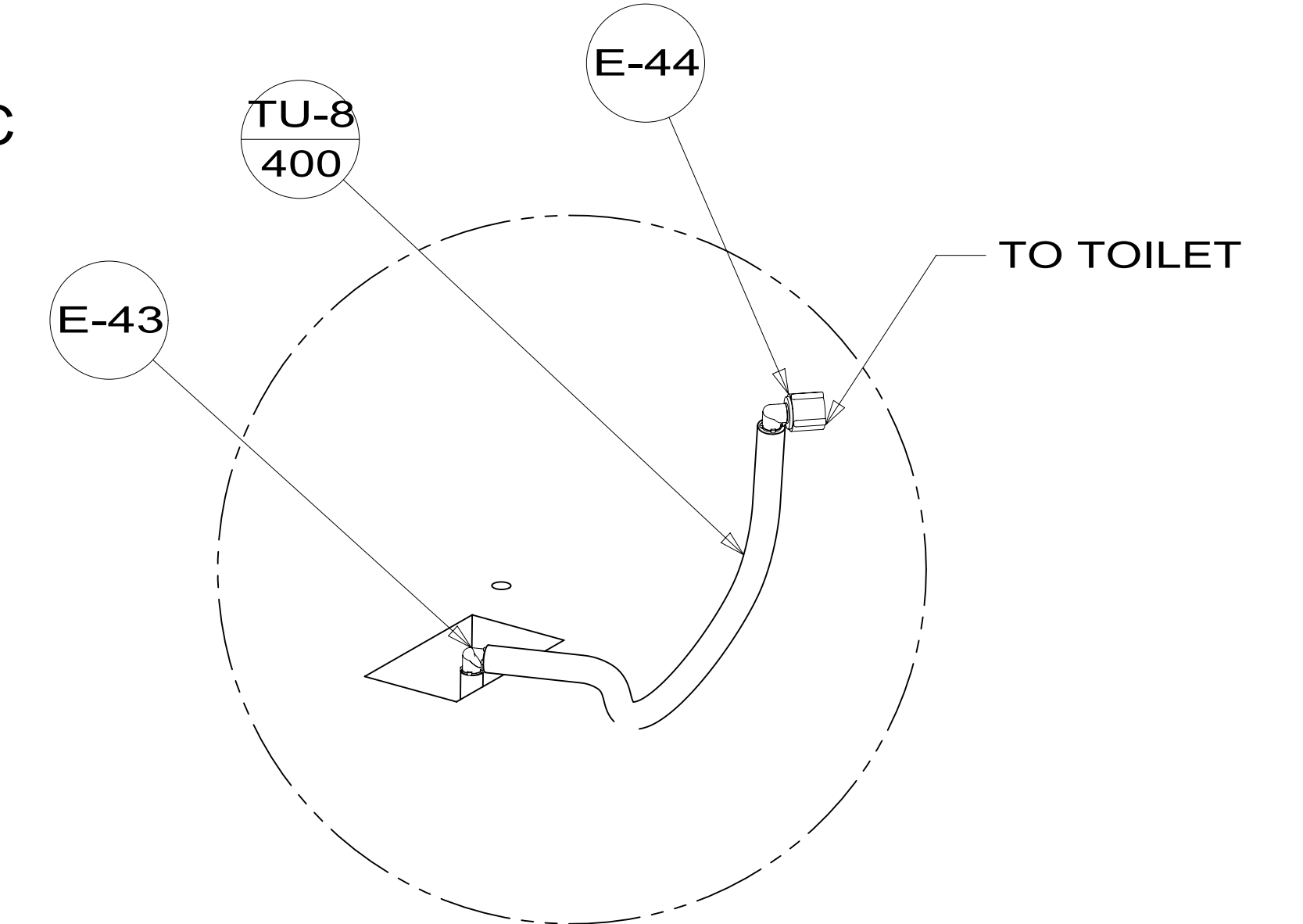
DETAIL CE (SHOWN W/OUT CABINETS)
