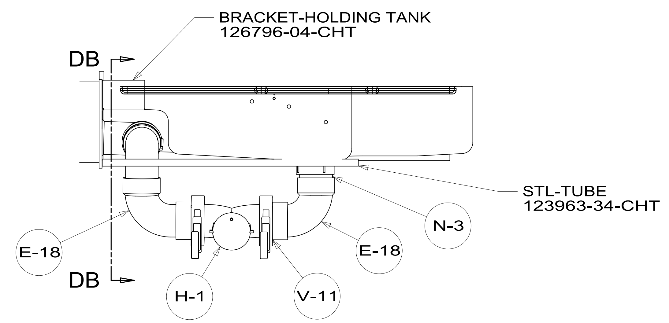
VIEW DA (SHOWN W/OUT PANEL ASM)
