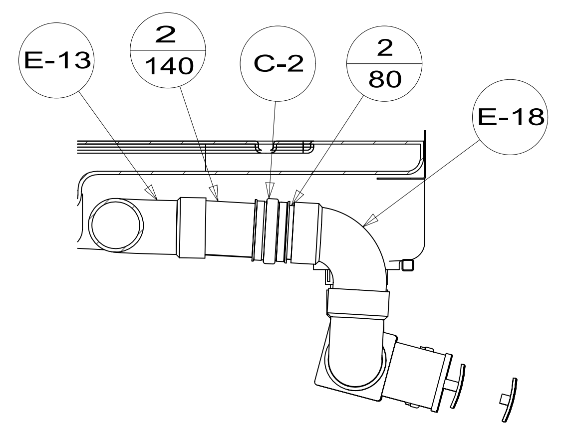
SECTION DB-DB
