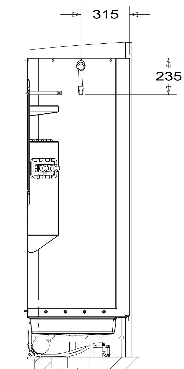
SECTION BE-BE
