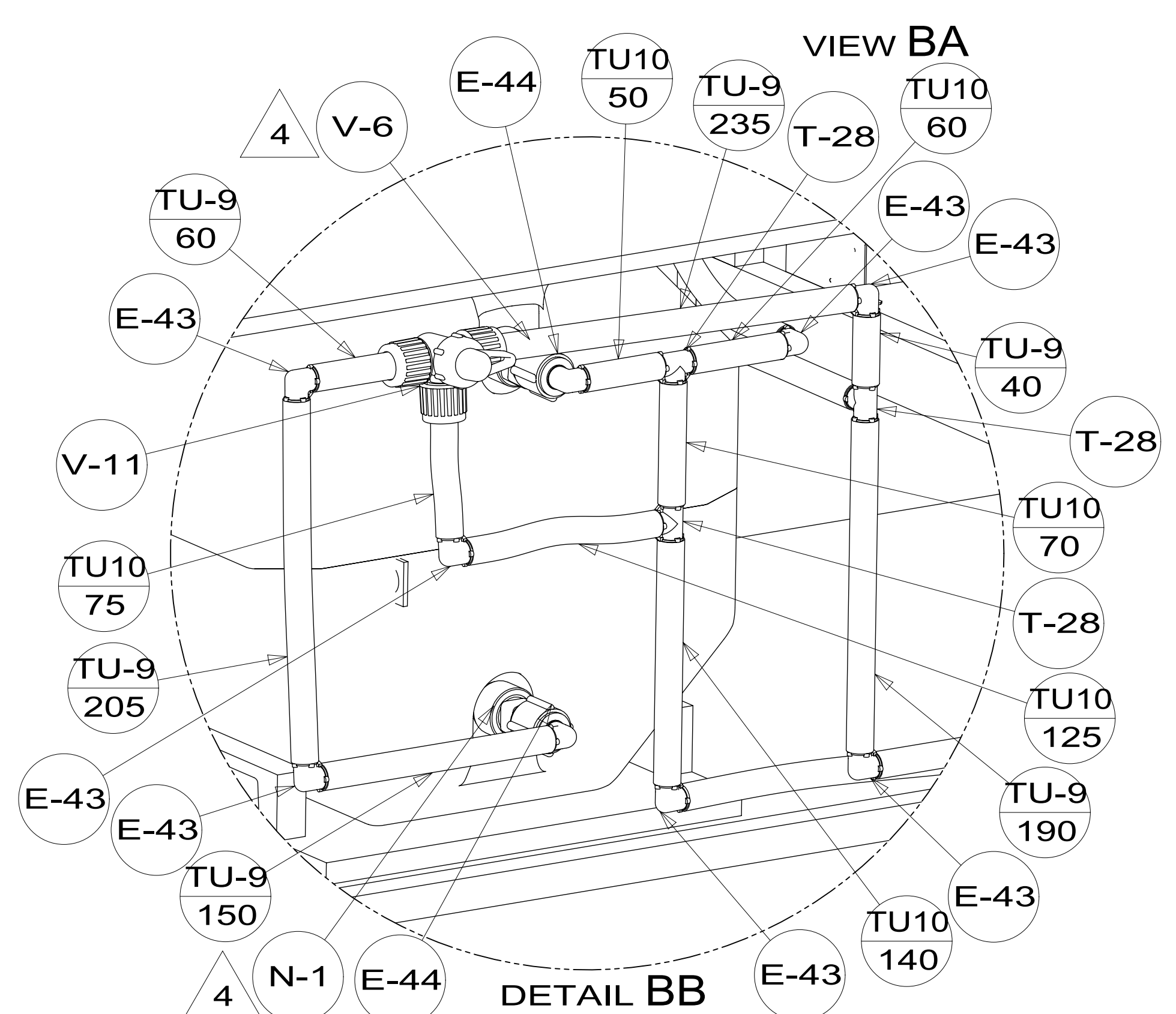
DETAIL BB
