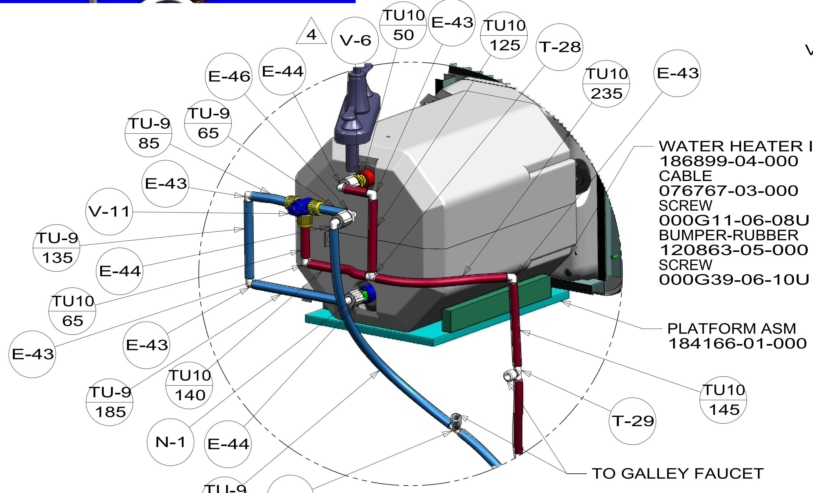
DETAIL BC (SHOWN W/OUT CABINETS & FAUCET)
