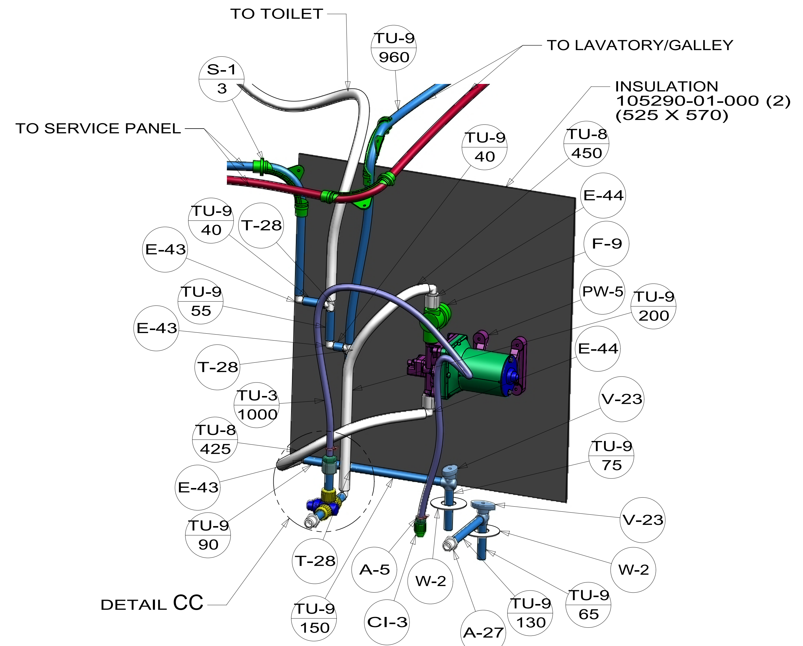
VIEW CB (SHOWN W/OUT TANKS)
