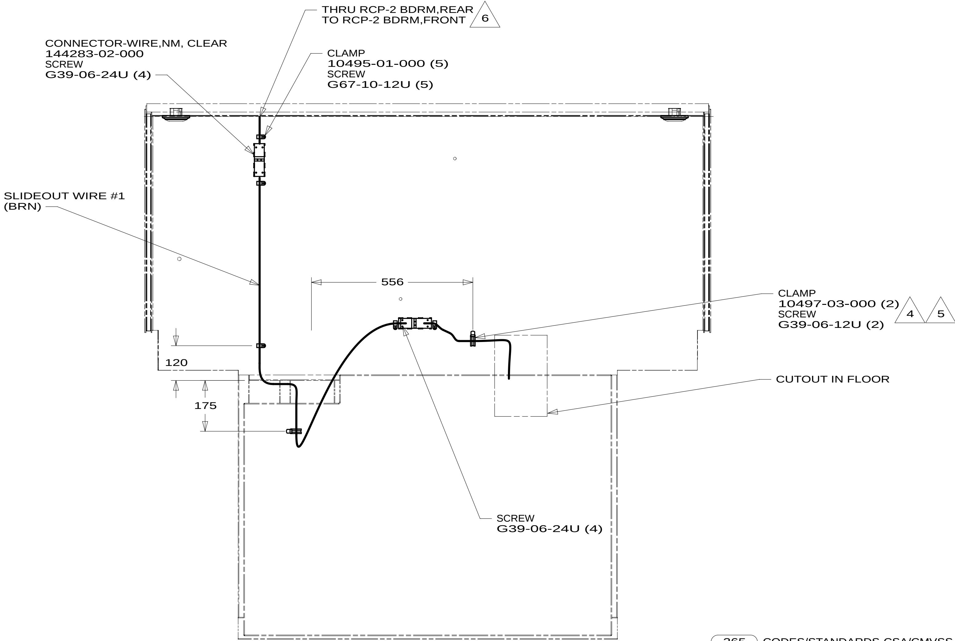
DETAIL DB
