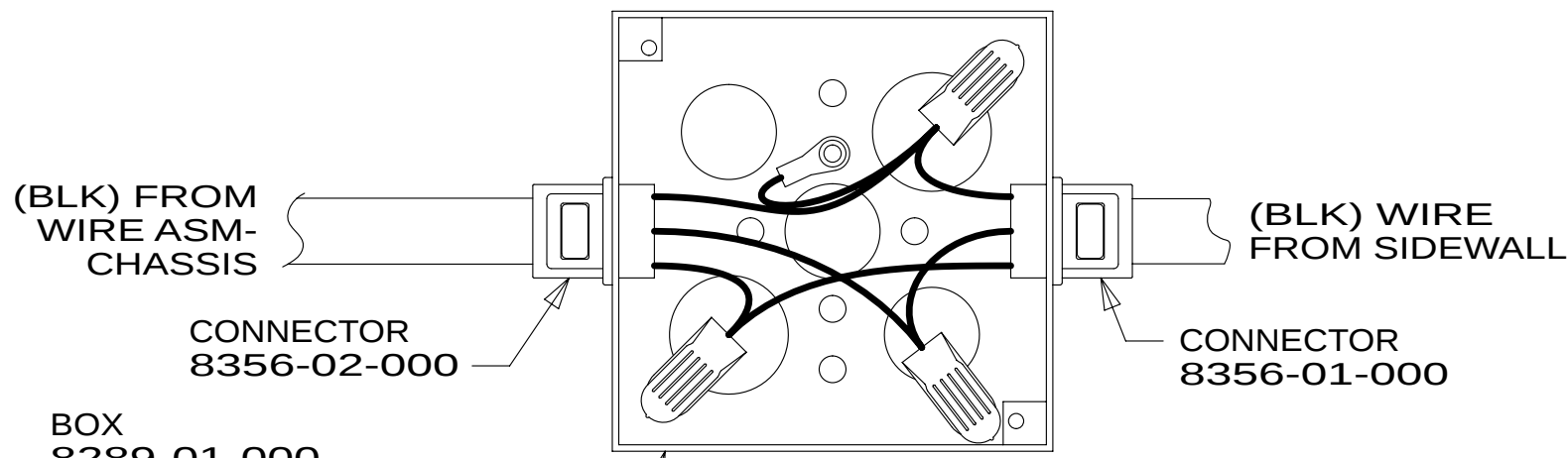
DETAIL BB
