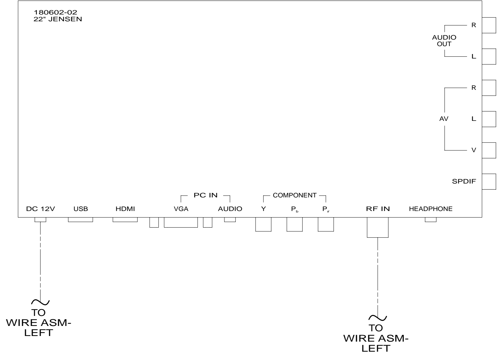
DETAIL FA
