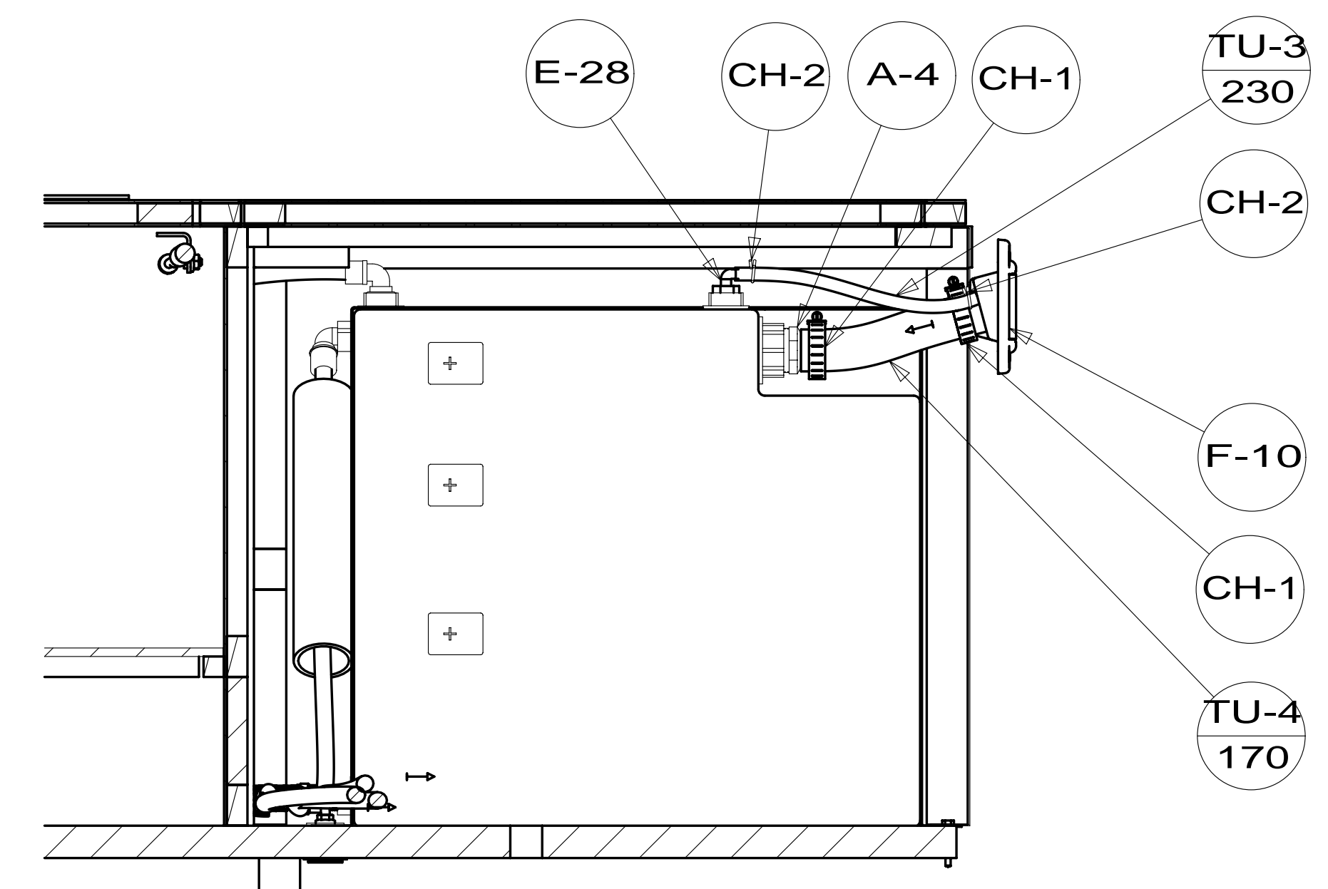
SECTION EC-EC
