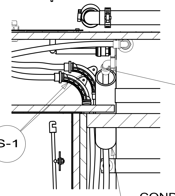
SECTION BF-BF
