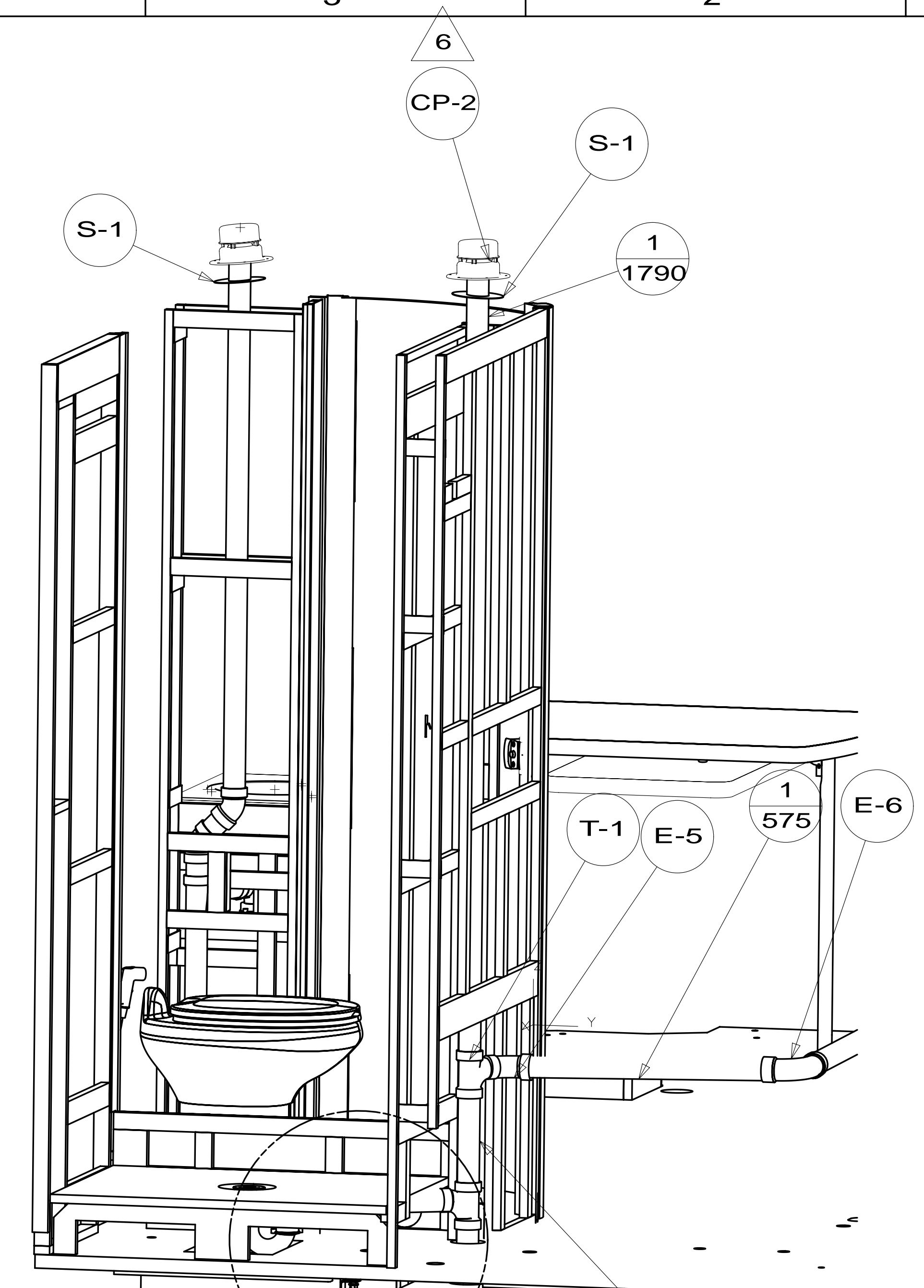
DETAIL DB
