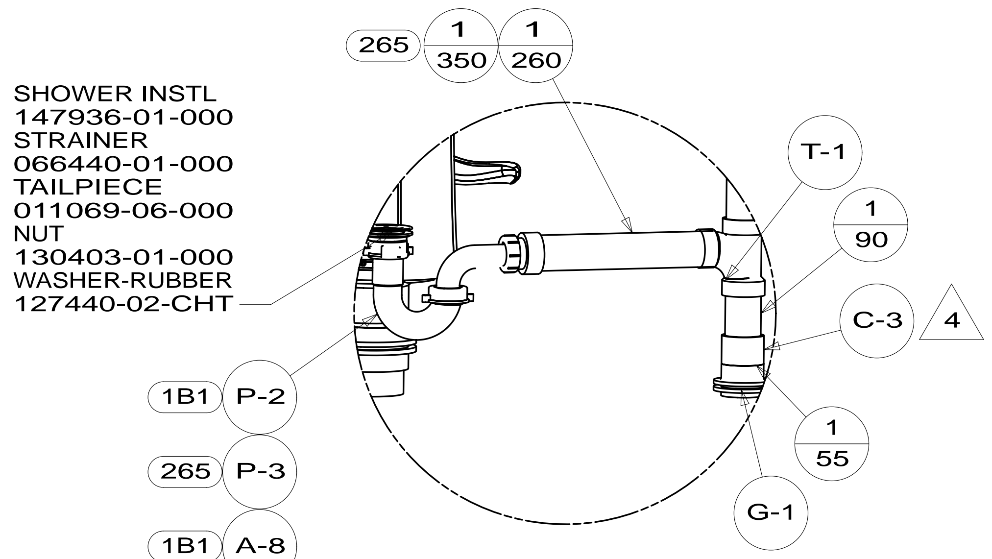
DETAIL DB (SHOWN W/OUT CABINETS AND FLOOR)
