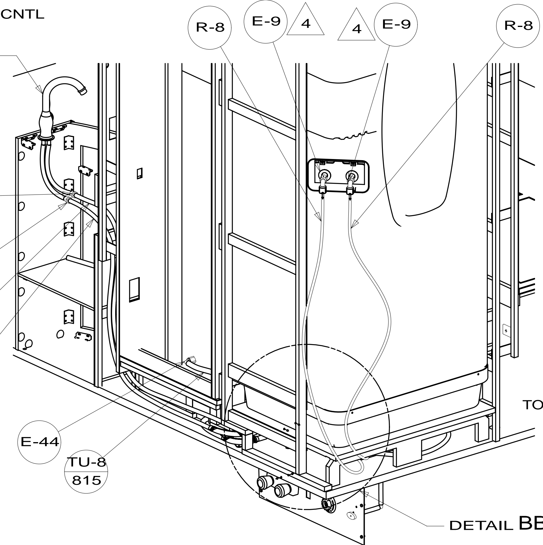
VIEW BA
