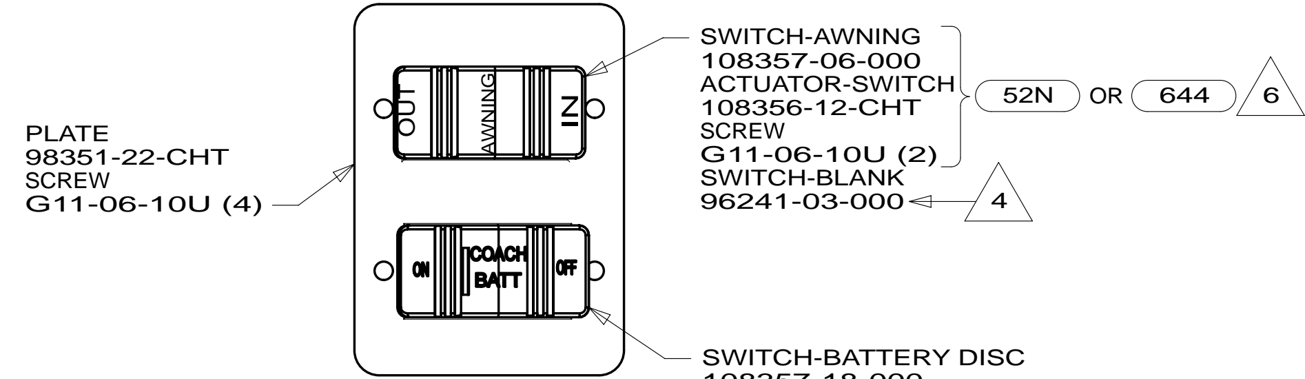
DETAIL CH
