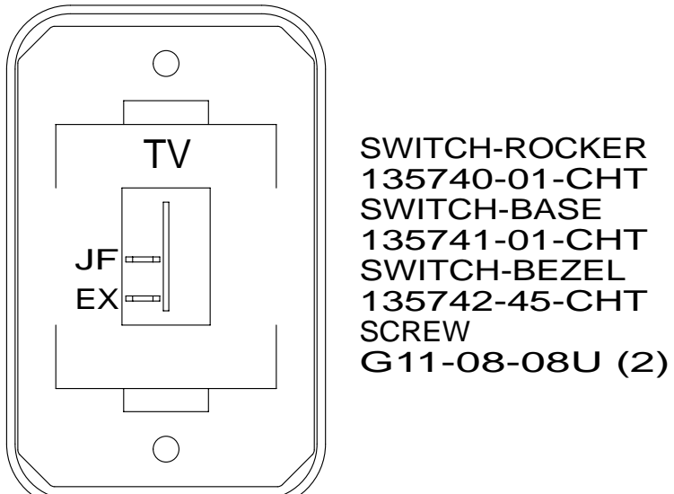
DETAIL CB 644
