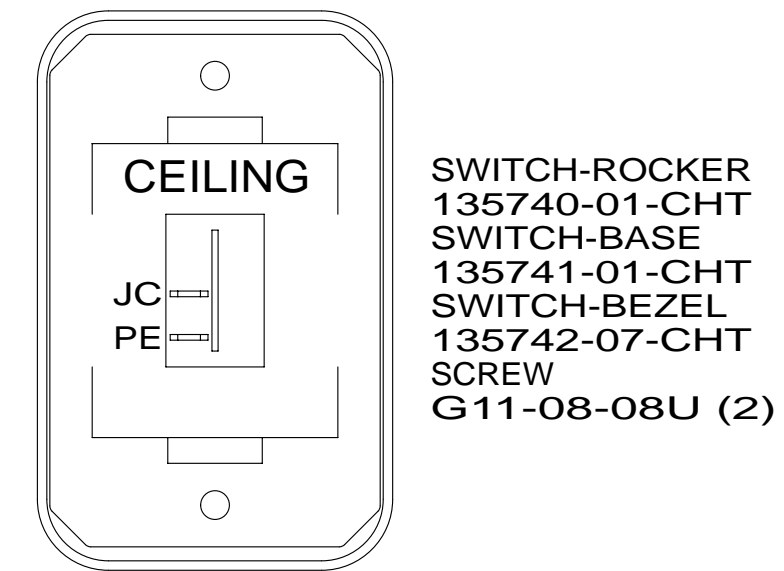
DETAIL CG
