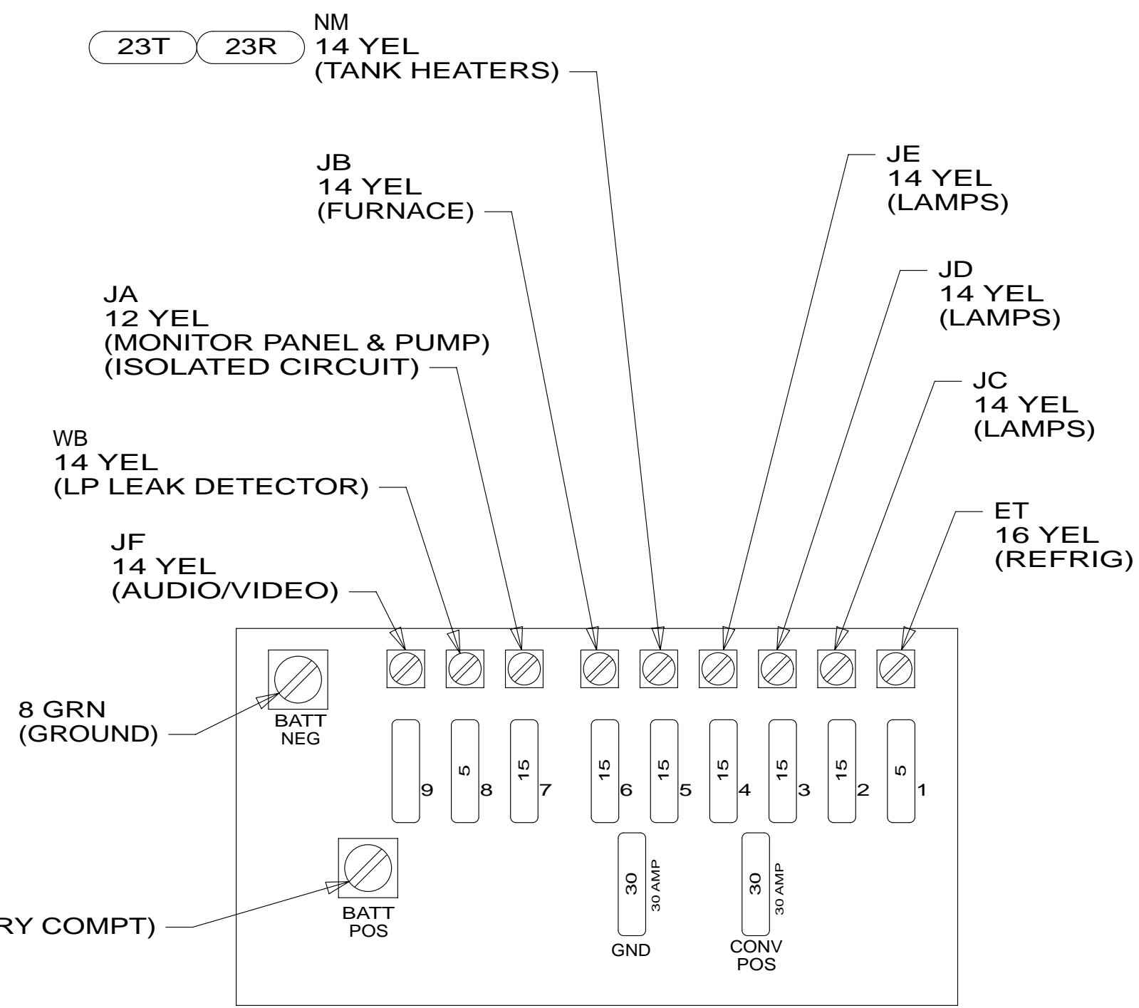
DETAIL CA
