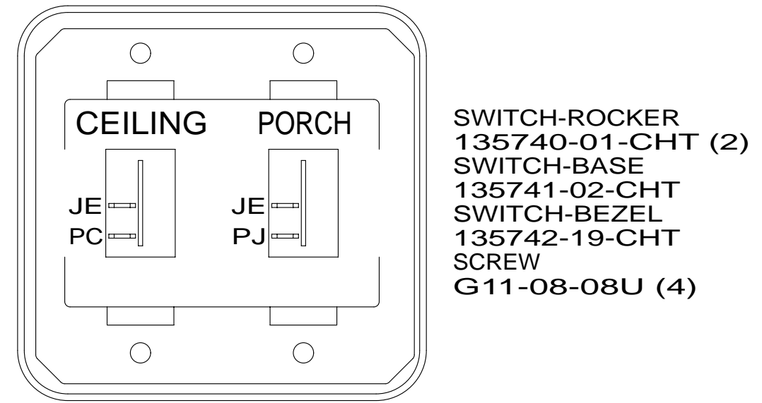
DETAIL CF
