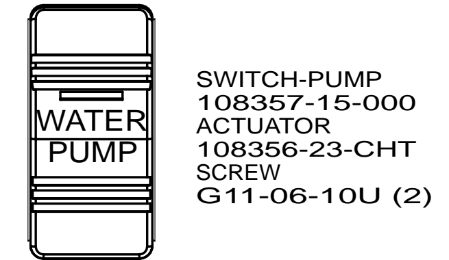
DETAIL CD
