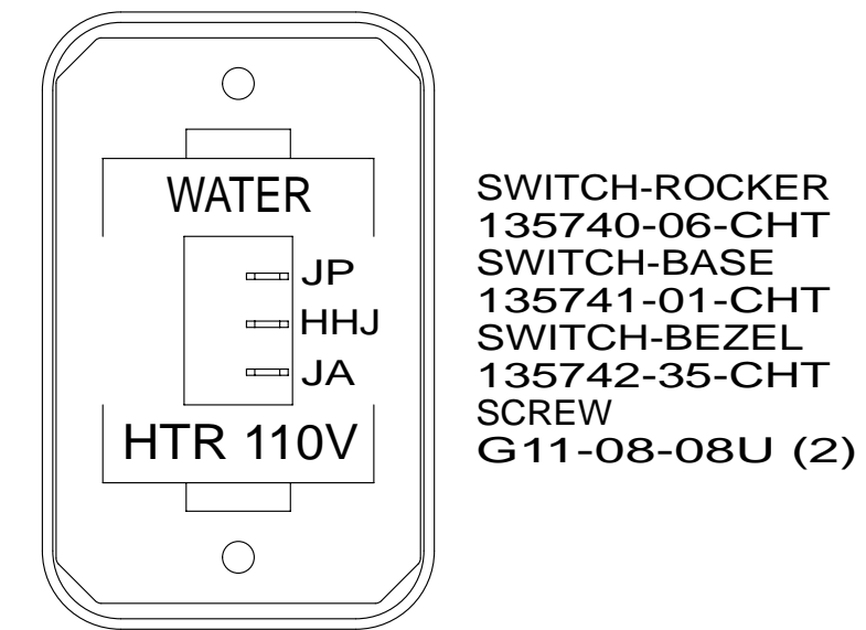
DETAIL CC 53B
