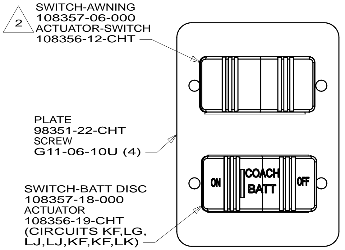
DETAIL CF
