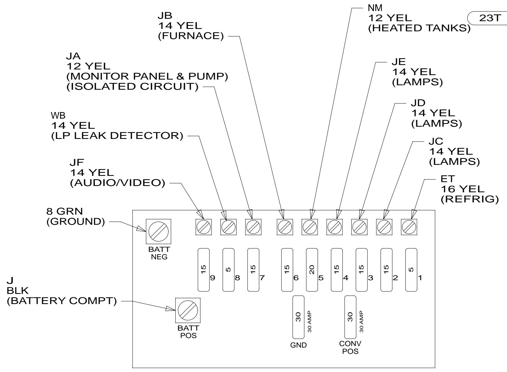
DETAIL CE 1
