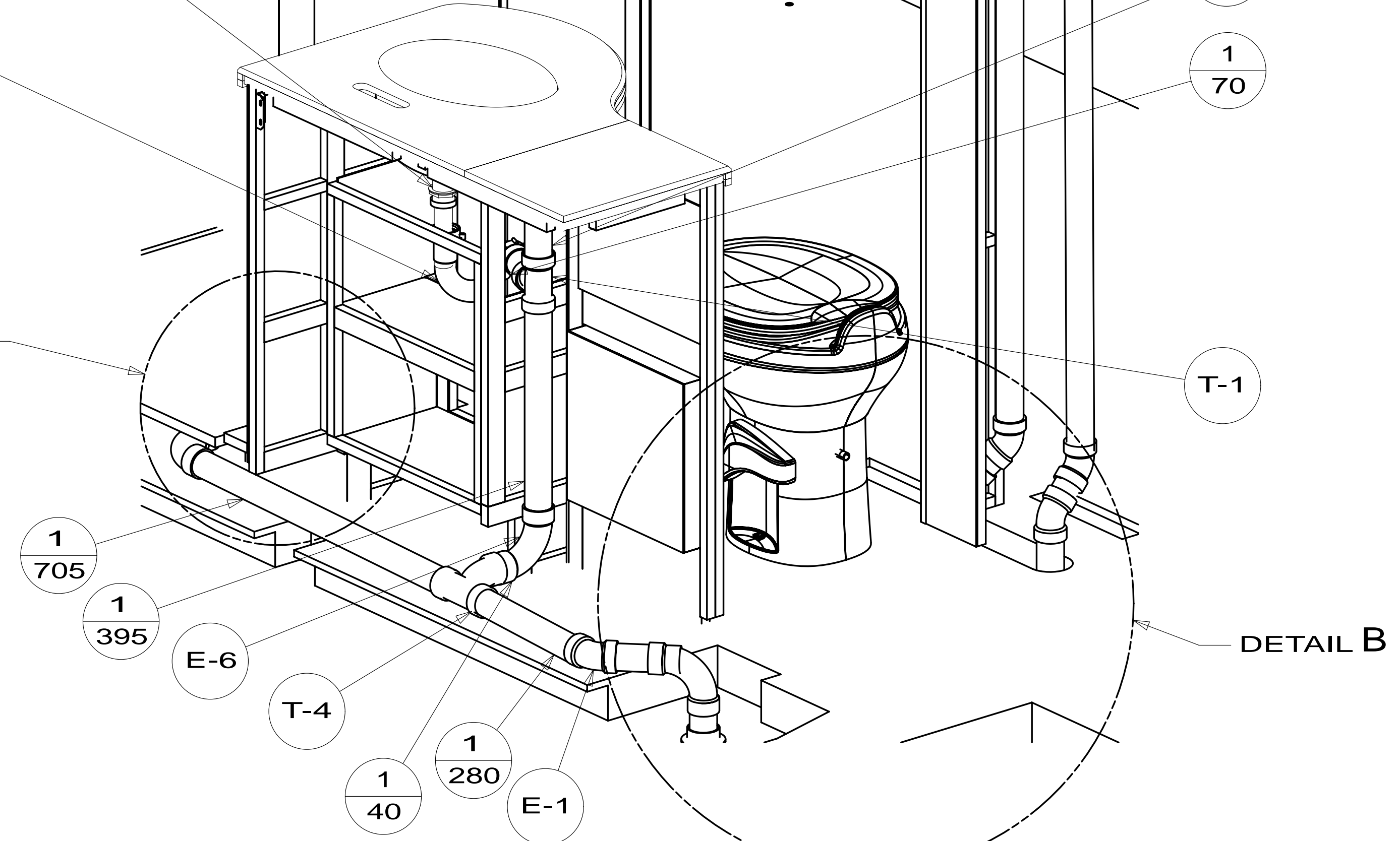
VIEW A
