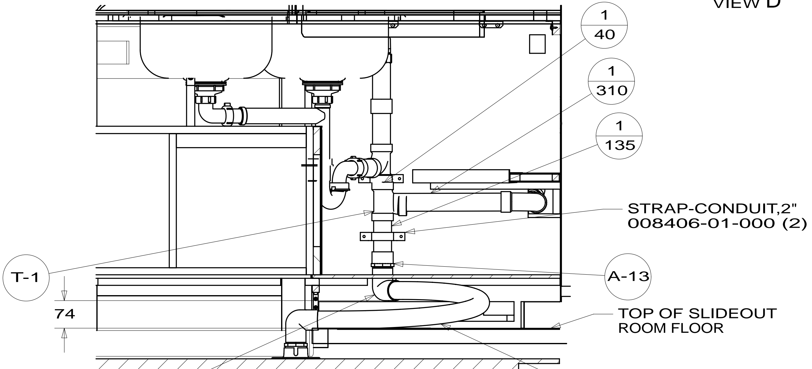
SECTION F-F (ROTATED)
