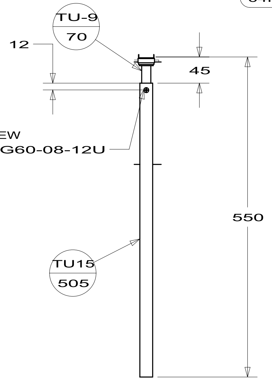
DETAIL R
