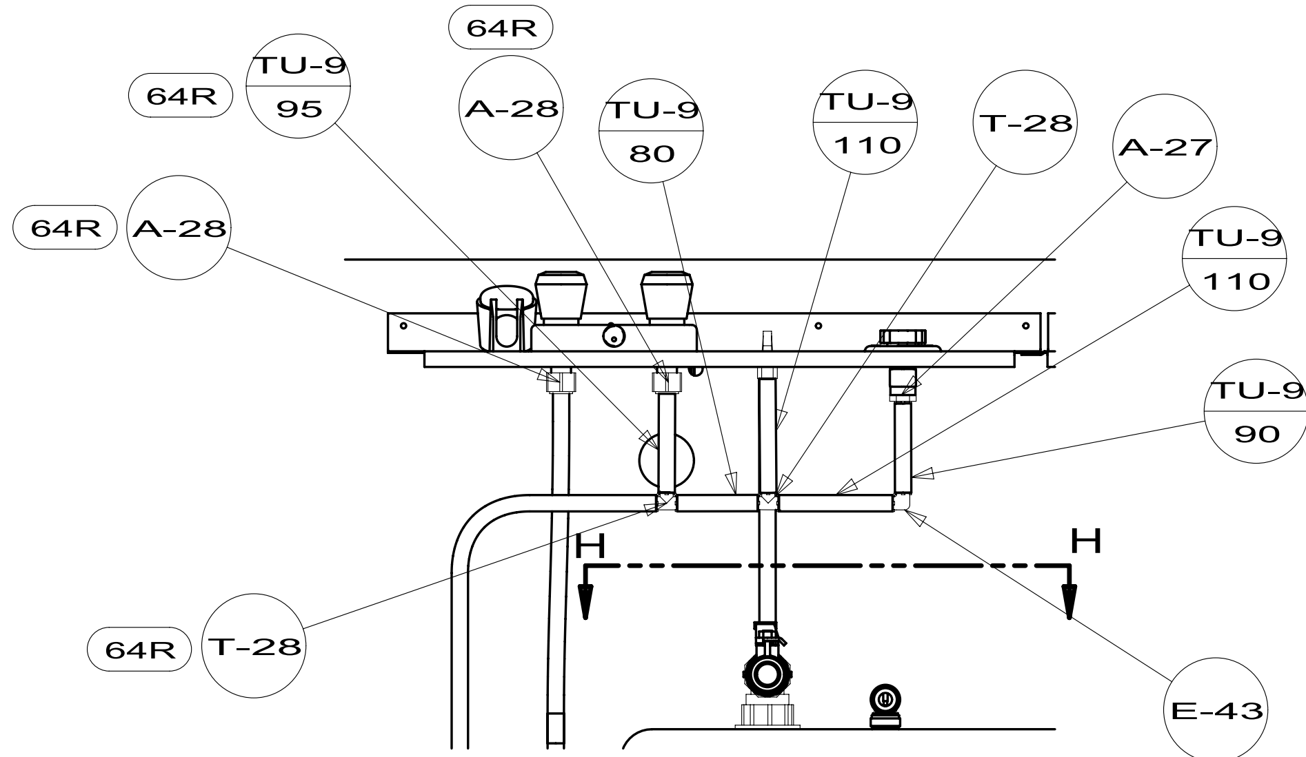
VIEW G
