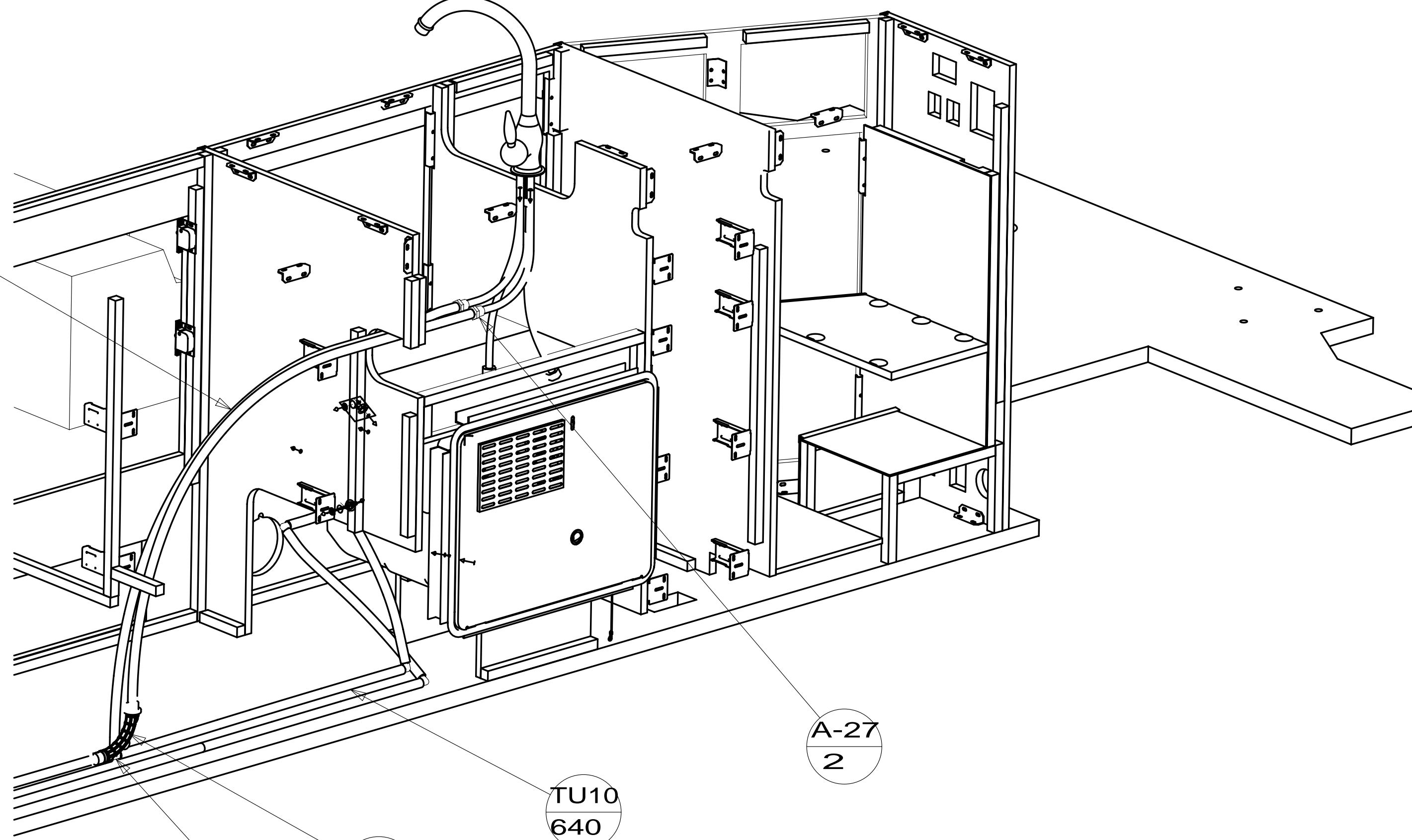
VIEW D
