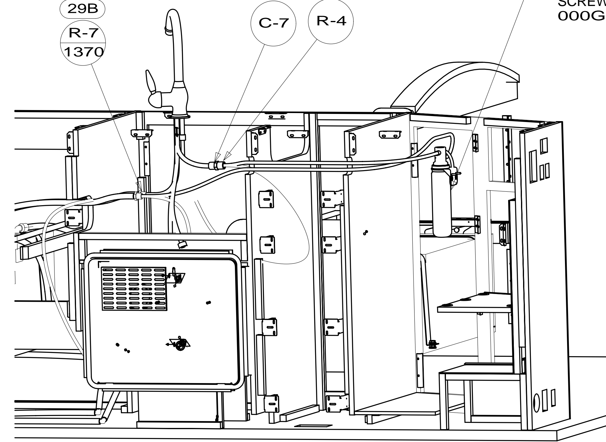
VIEW C
