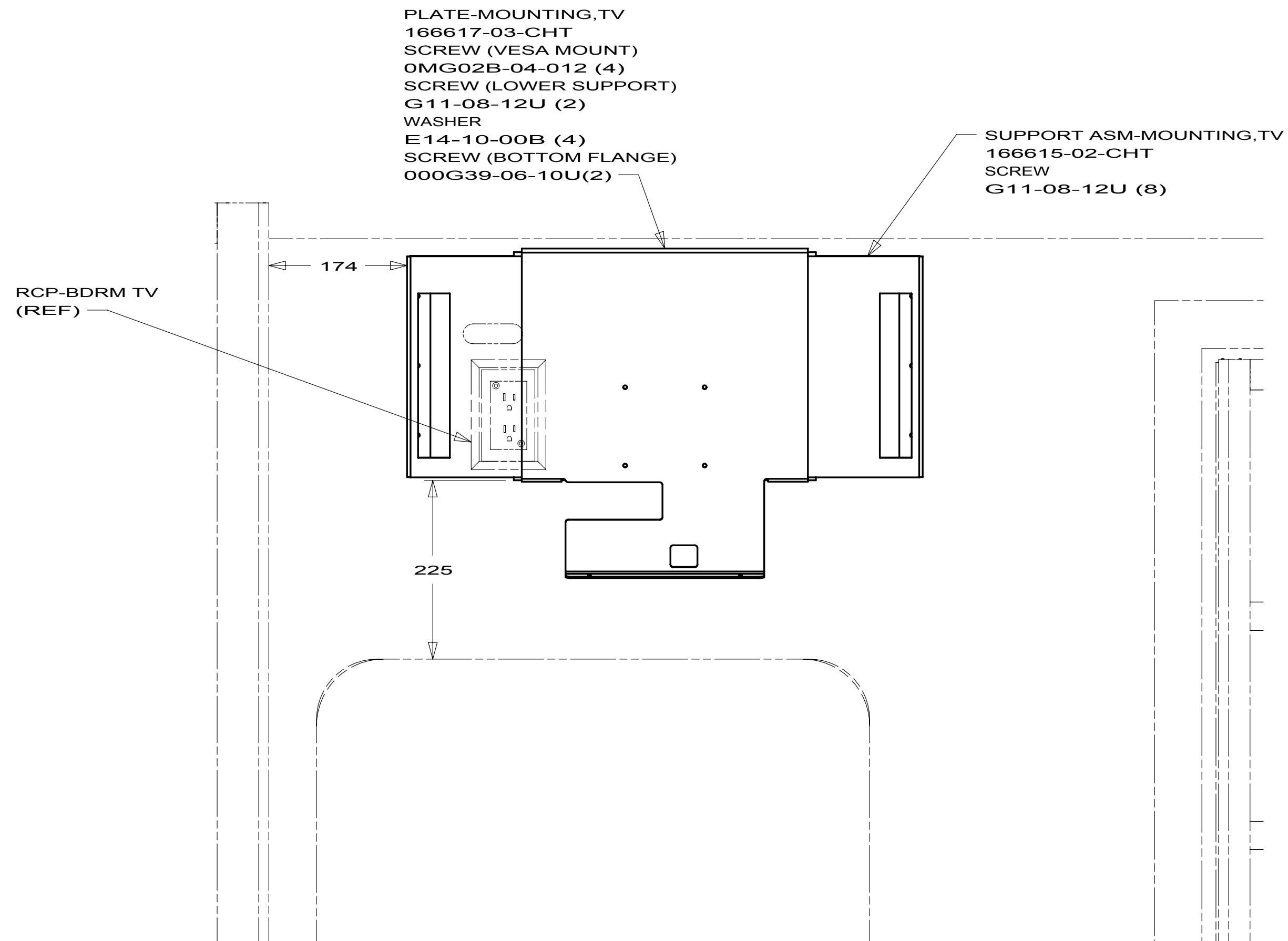
VIEW KA (TV NOT SHOWN)
