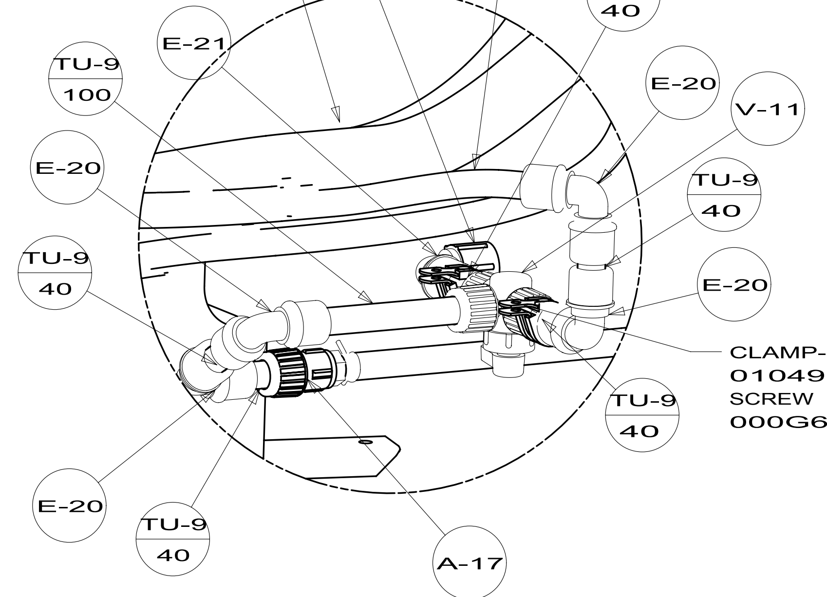
DETAIL F
