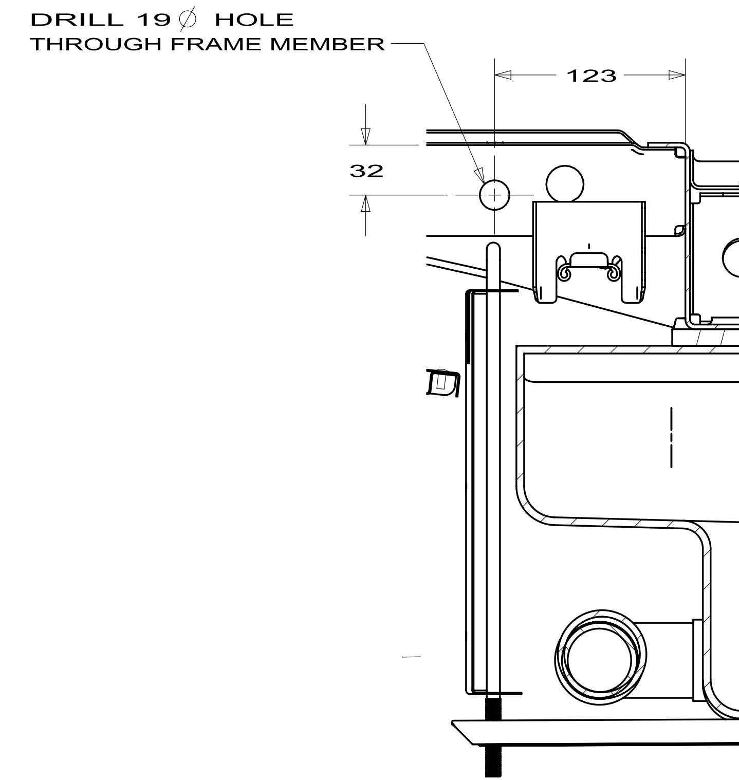
SECTION J-J
