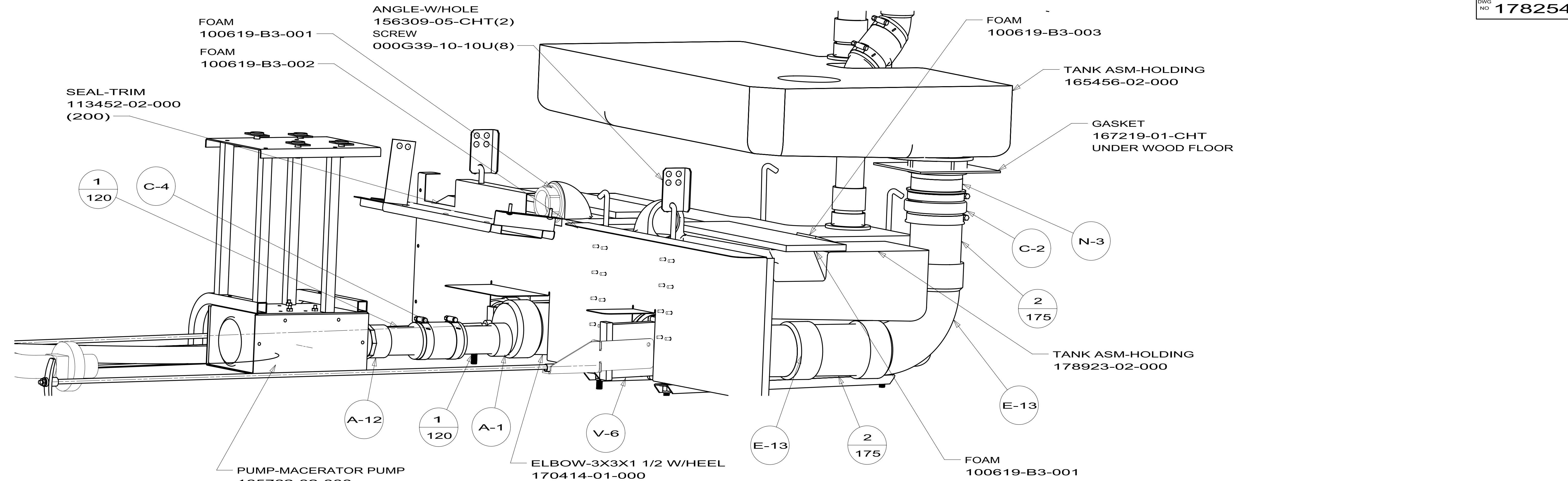
VIEW C
