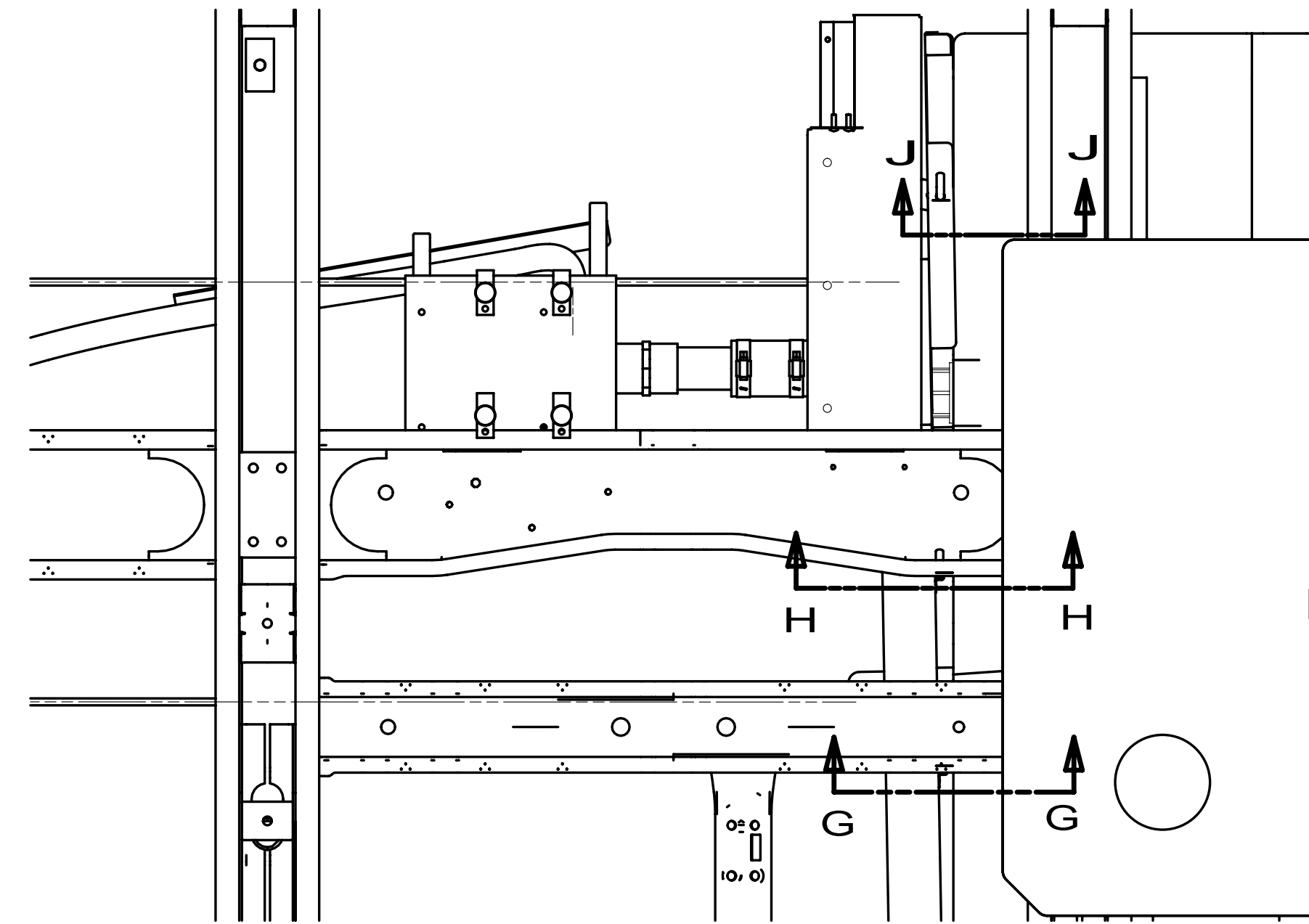
VIEW F
