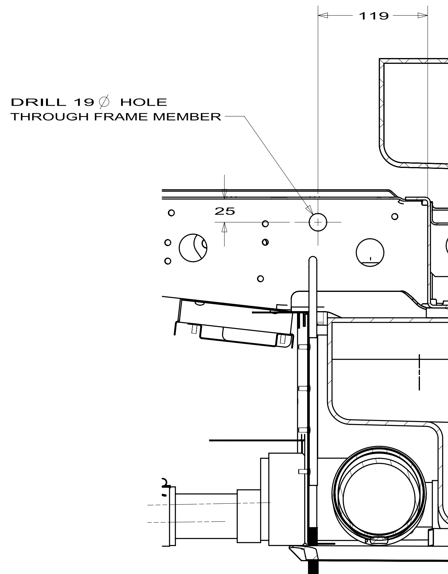
SECTION H-H
