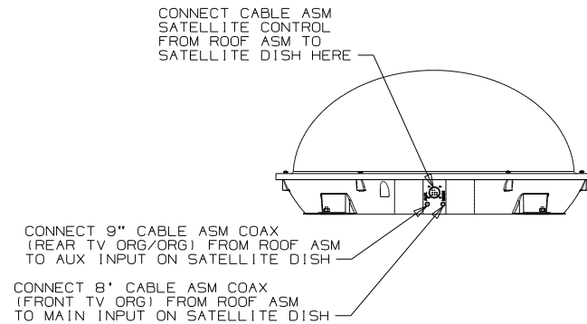
VIEW GF - GF
