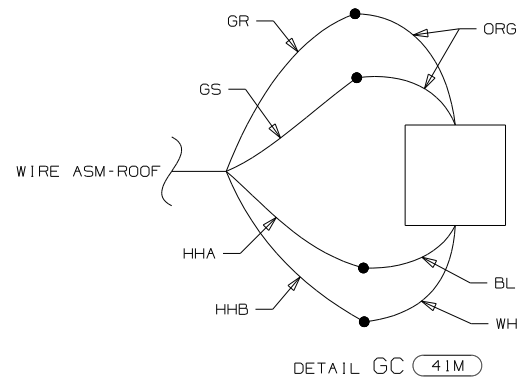
DETAIL GC 41M
