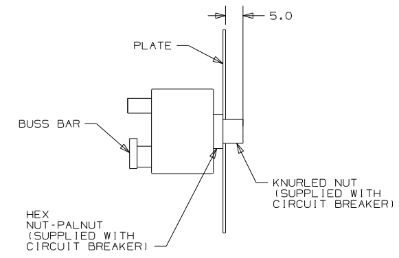
DETAIL DB-DB
