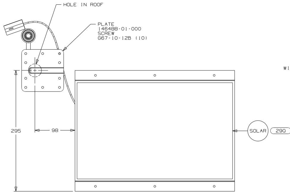
VIEW GA
