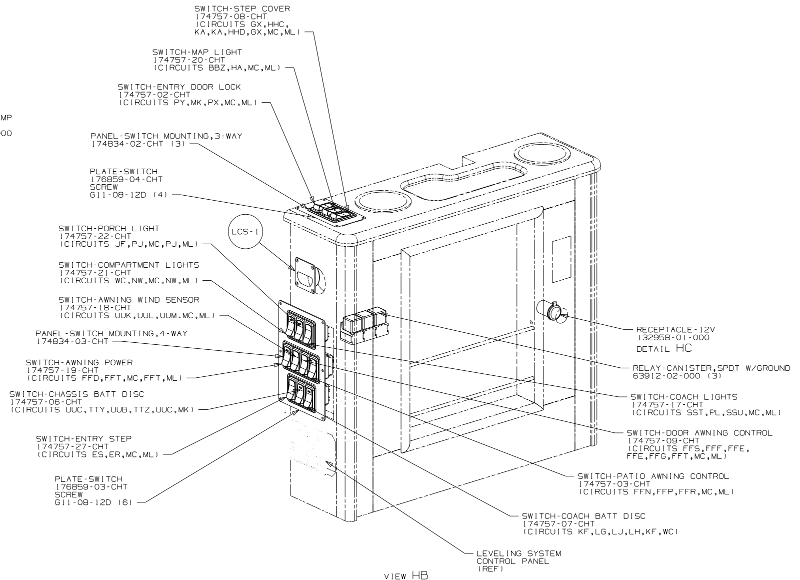
VIEW HB
