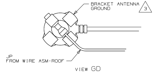
VIEW GD
