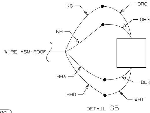
DETAIL GB
