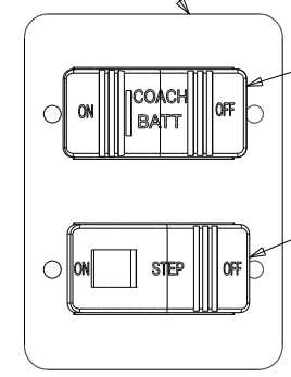
DETAIL DL
