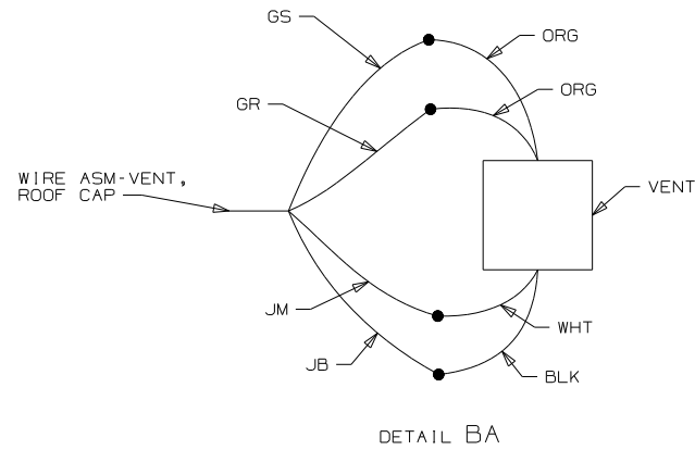
DETAIL BA
