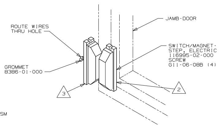
DETAIL DF
