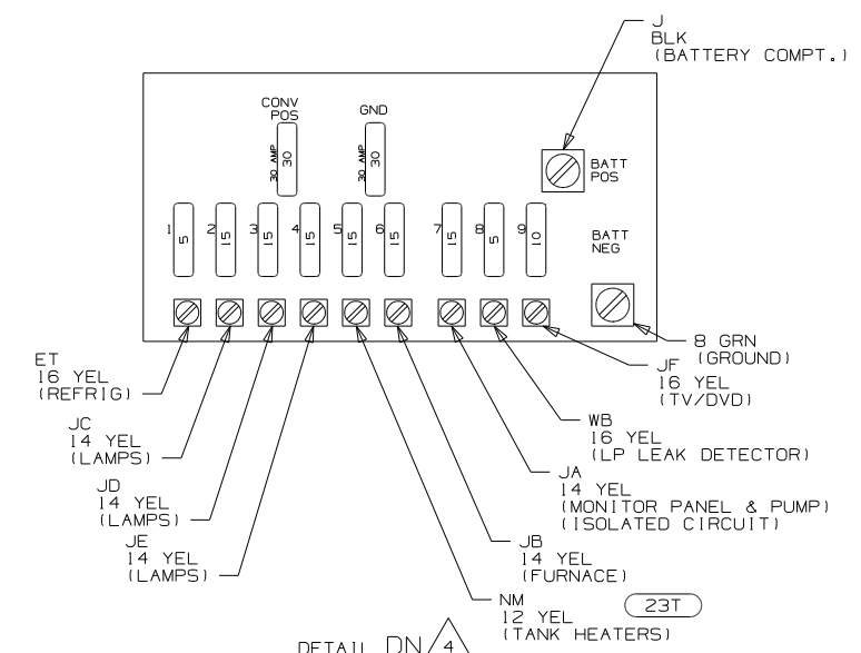
DETAIL DN
