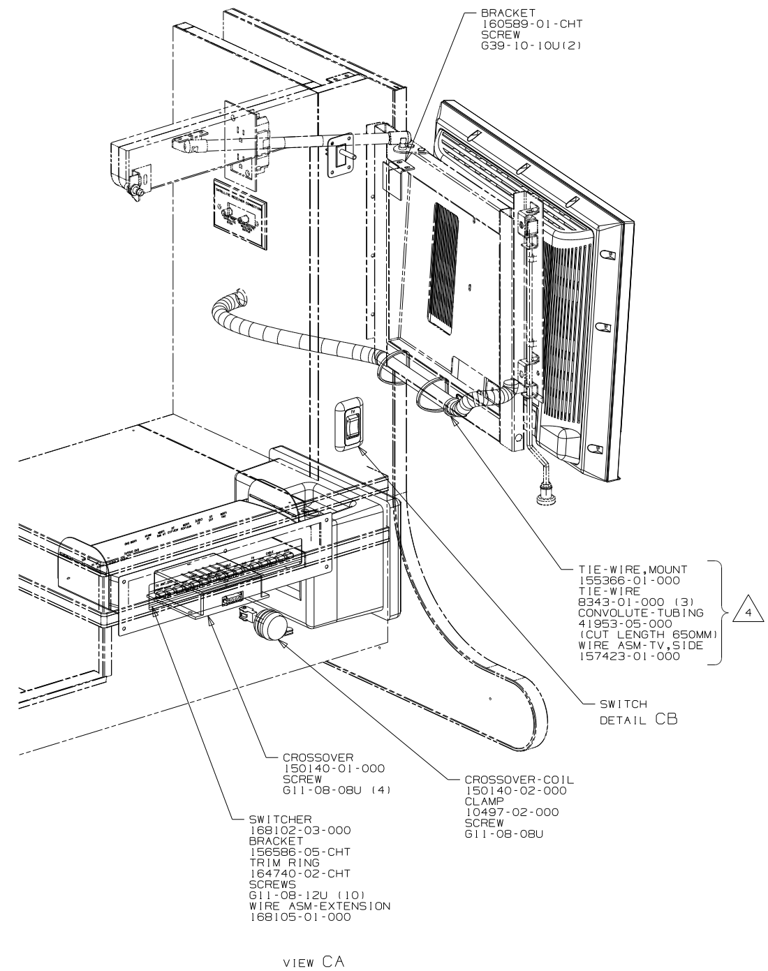
VIEW CA
