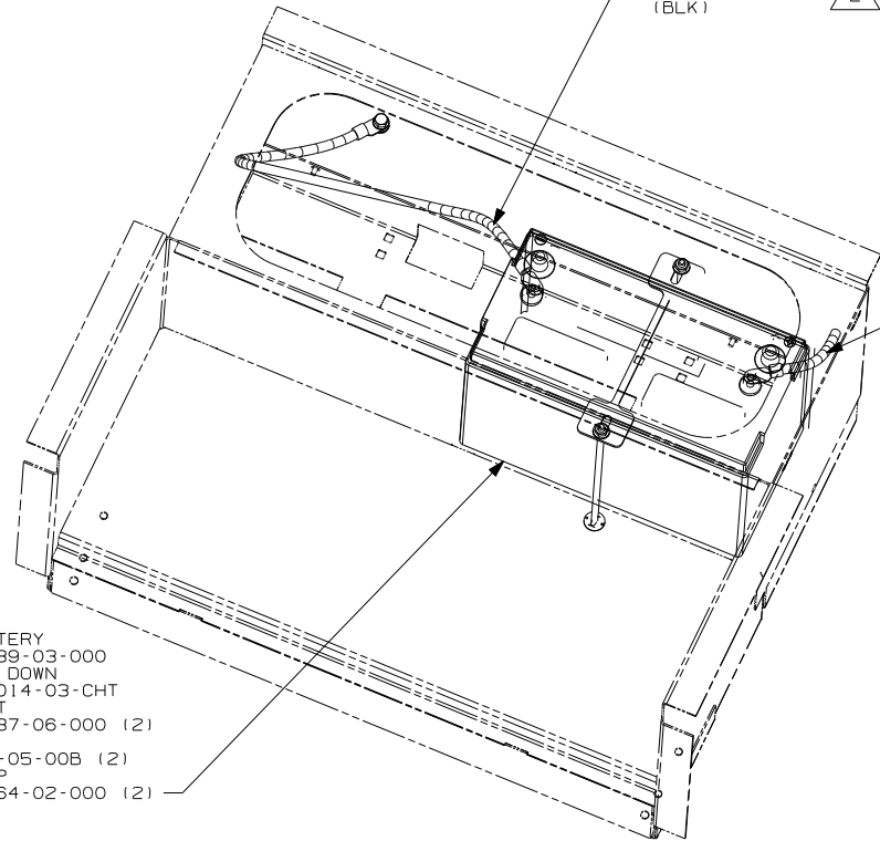
BATTERY BOX
