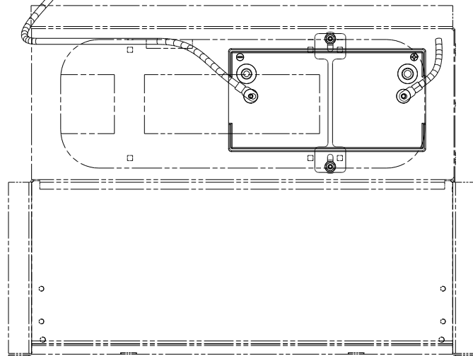
VIEW BA
