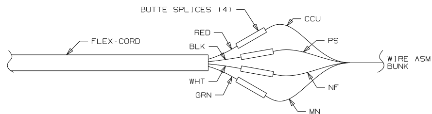
DETAIL CD
