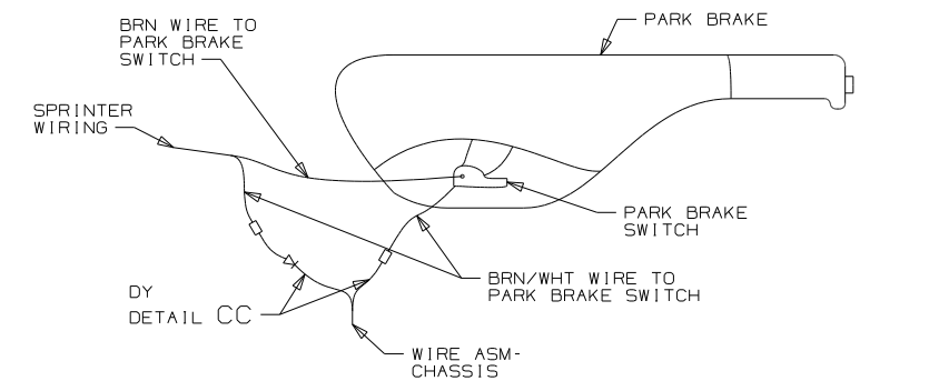
DETAIL CB
