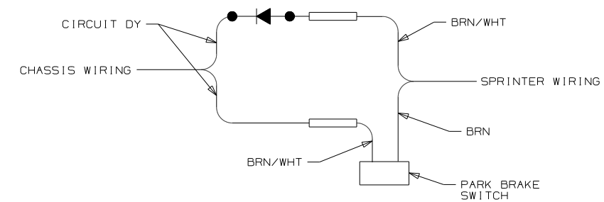
DETAIL CC
