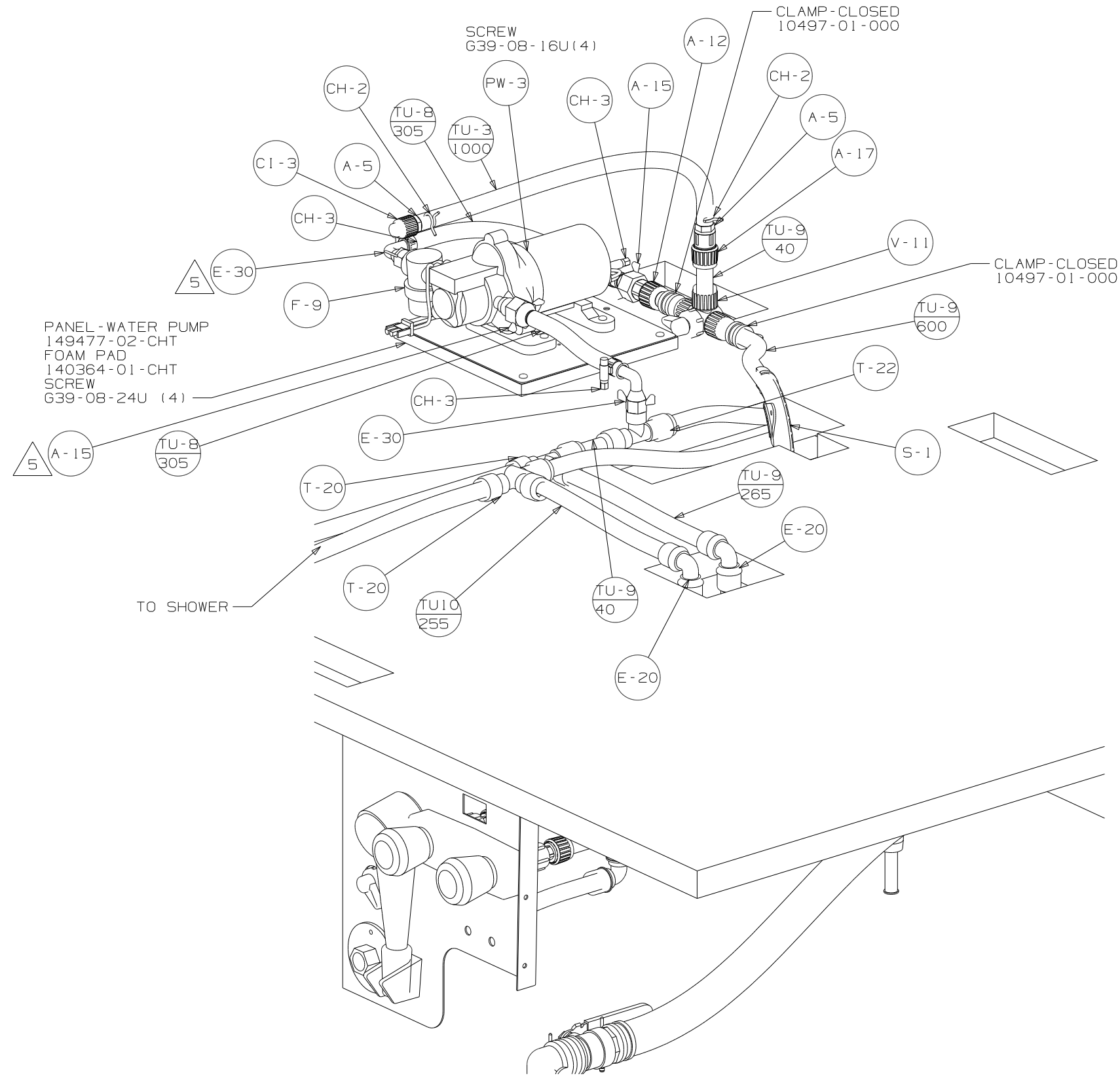
VIEW H
