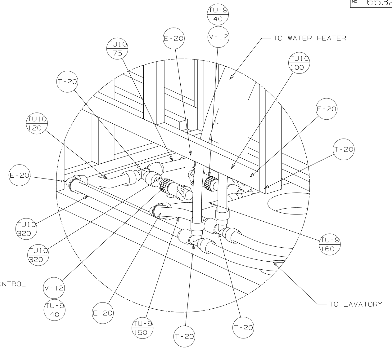
DETAIL D
