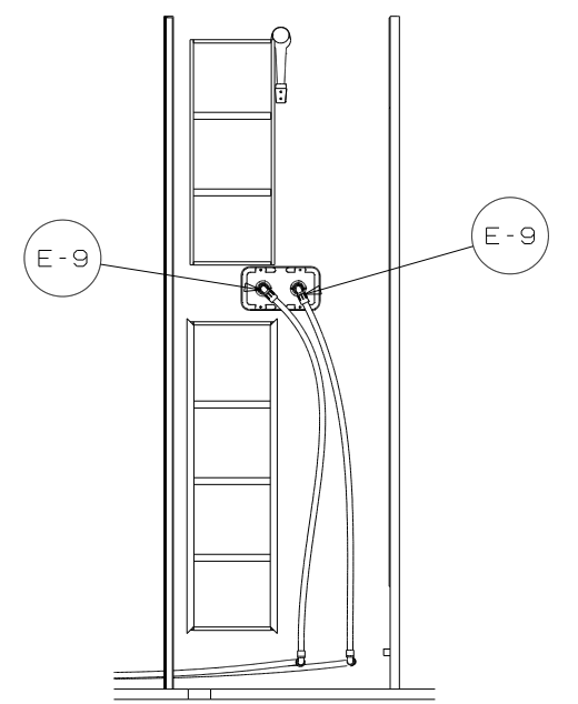
VIEW G
