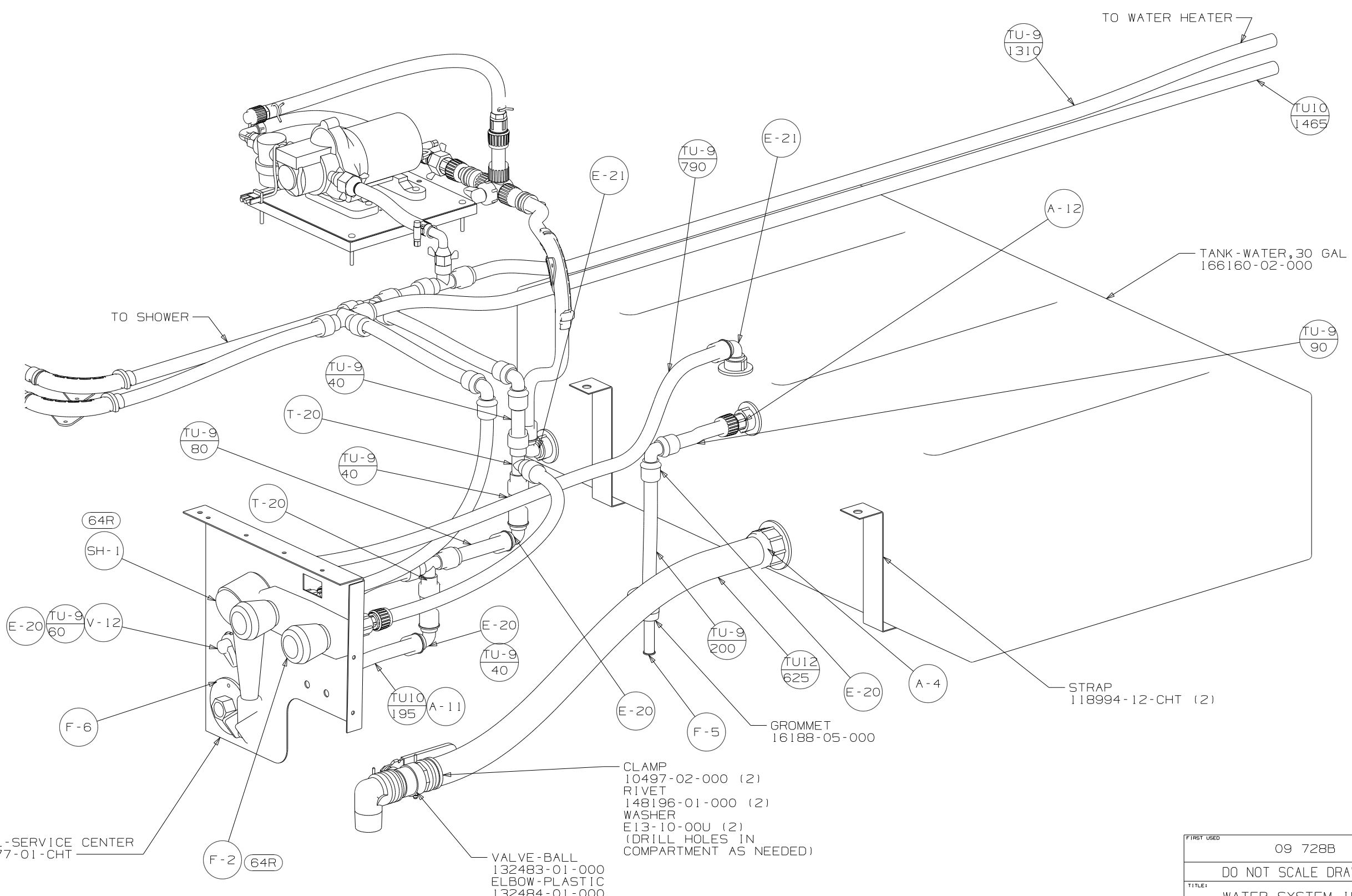
VIEW J
