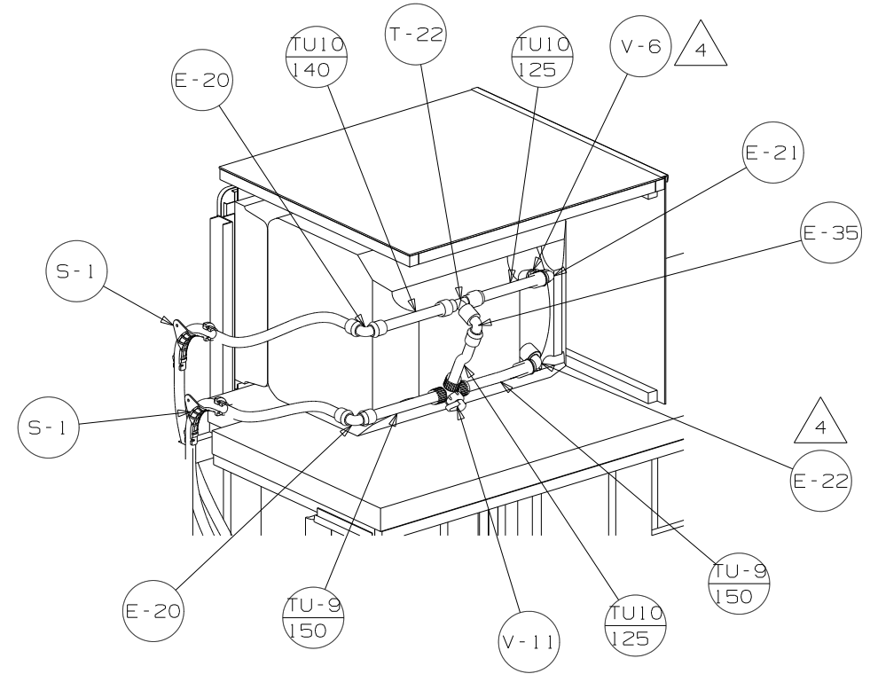
VIEW E
